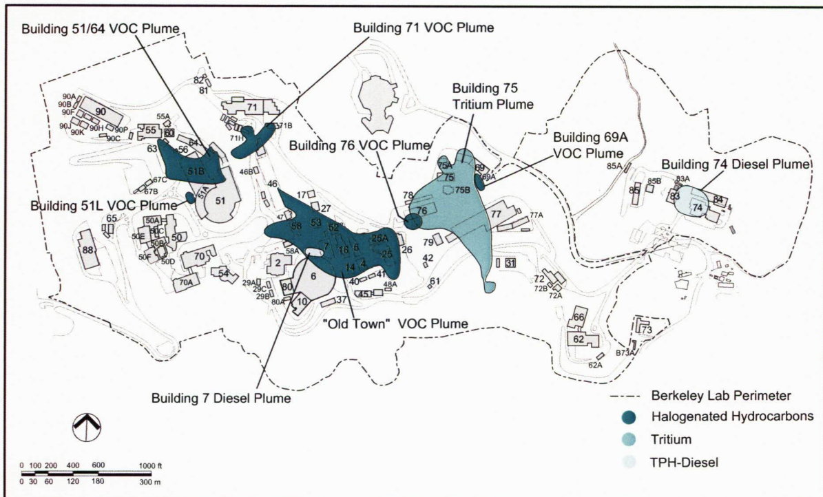
Figure 6-3 Groundwater Contamination Plumes (September 2004)
