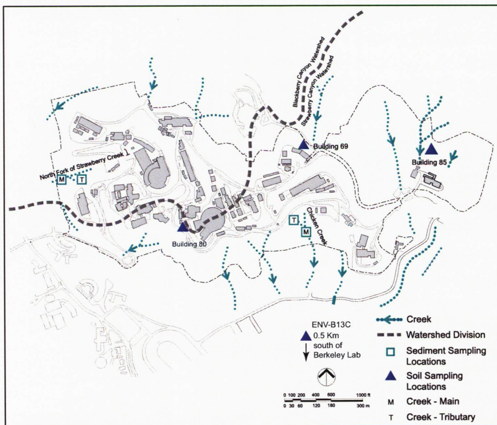
Figure 7-1 Soil and Sediment Sampling Sites
