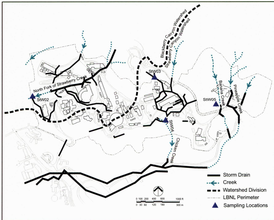
Figure 5-3 Stormwater Sampling Locations
