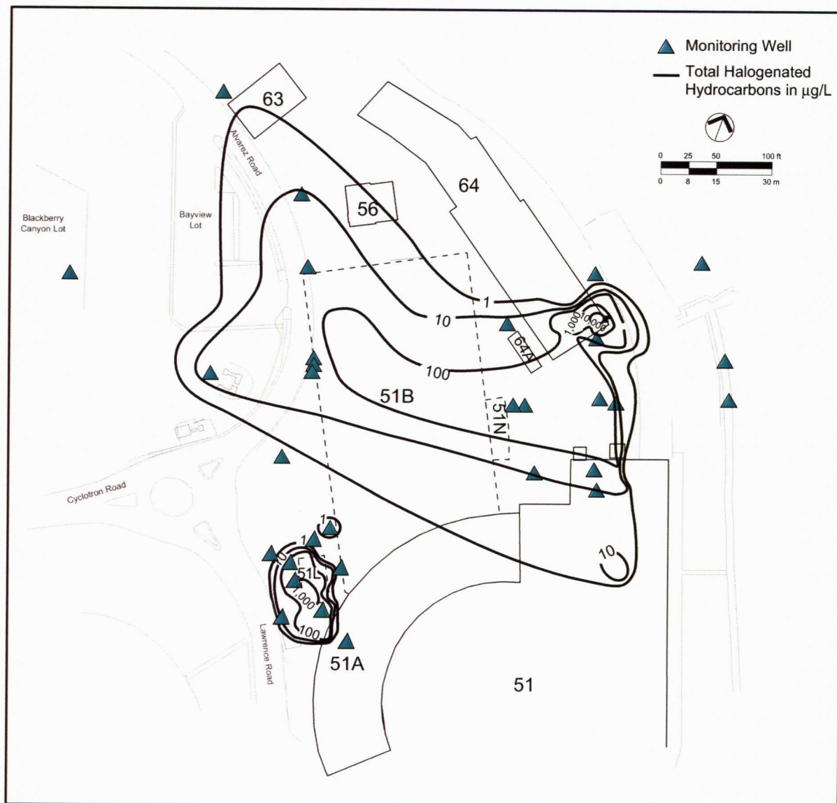
Figure 6-5 Groundwater Contamination (Total Halogenated Hydrocarbons in Micrograms per Liter [ \mu\text{g/L} ]) at Building 51/64 VOC Plume (September 2004)
