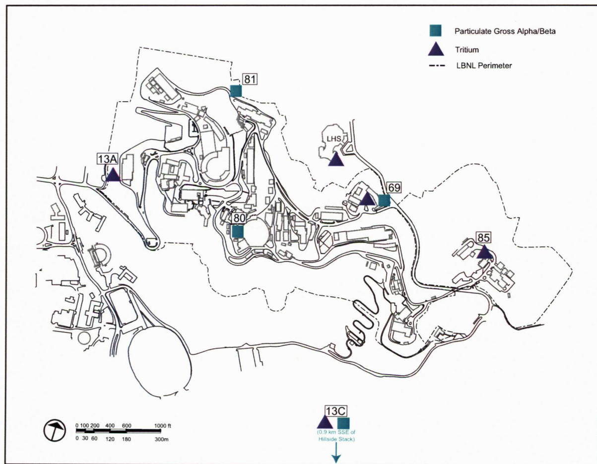
Figure 4-3 Ambient-Air Monitoring Network Sampling Locations
