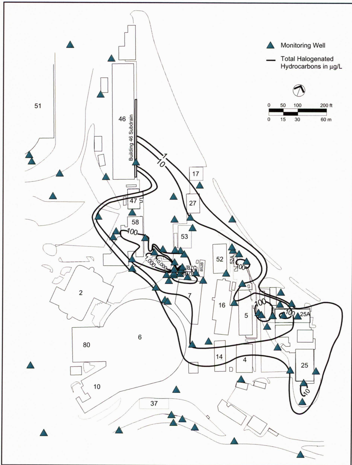
Figure 6-4 Groundwater Contamination (Total Halogenated Hydrocarbons in Micrograms per Liter [ \mu\text{g/L} ]) in Old Town Area (September 2004)
