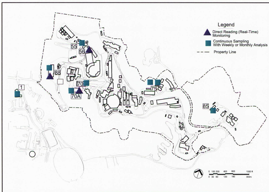
Figure 4-1 Locations of Building Exhaust Sampling and Monitoring in 2004
