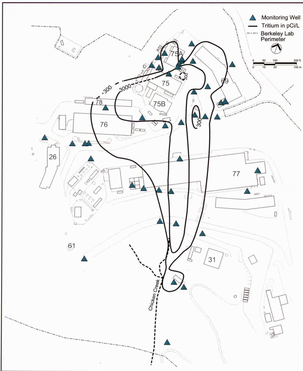
Figure 6-6 Groundwater Contamination (Tritium in Picocuries per Liter [pCi/L]) (September 2004)
