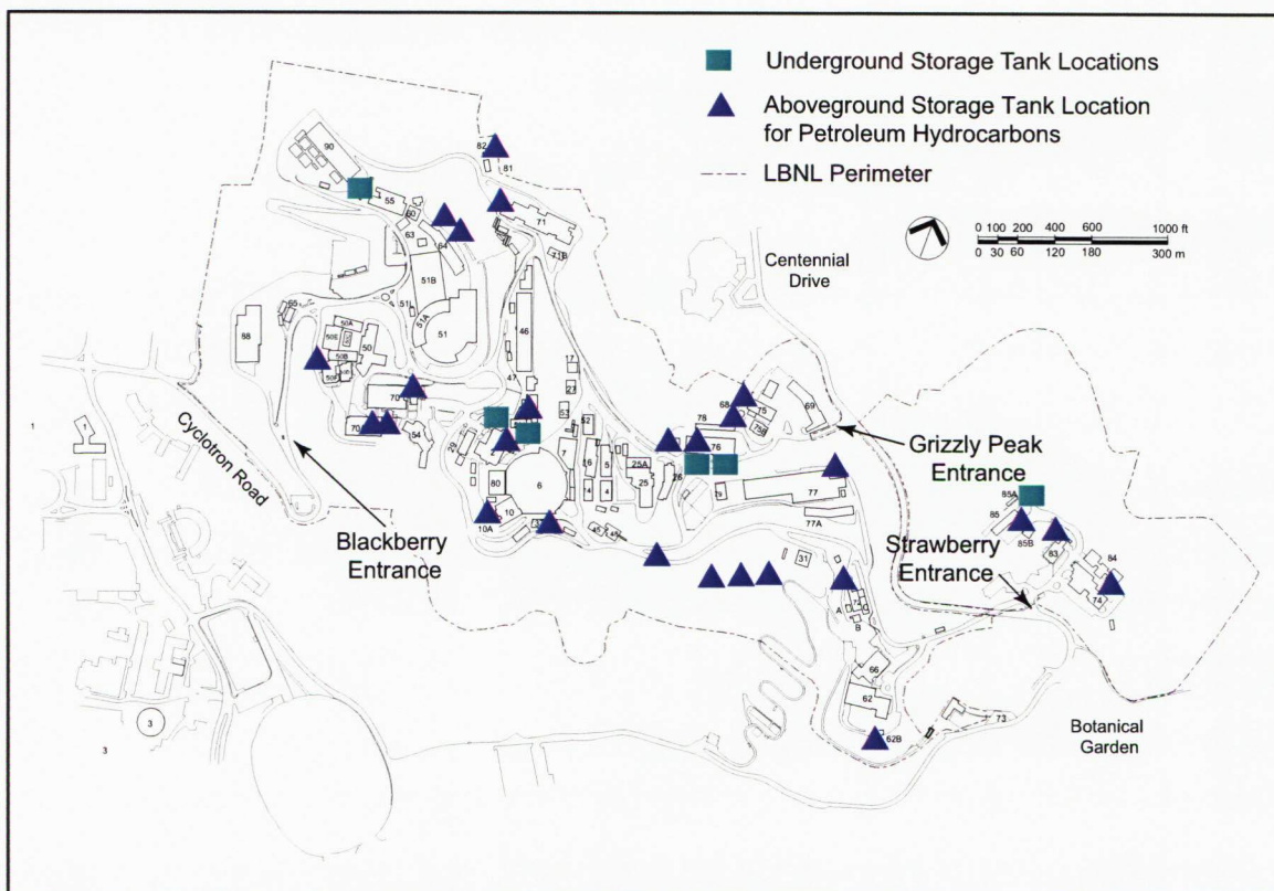
Figure 3-2 Aboveground and Underground Storage Tank Locations at the end of Calendar Year 2004
