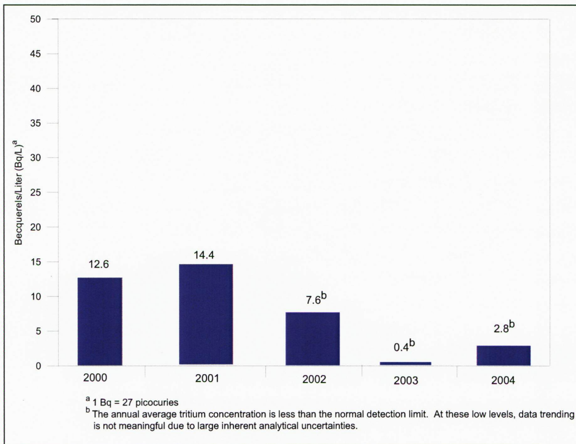
Figure 5-2 Annual Averages for Tritium in Chicken Creek (2000–2004)
