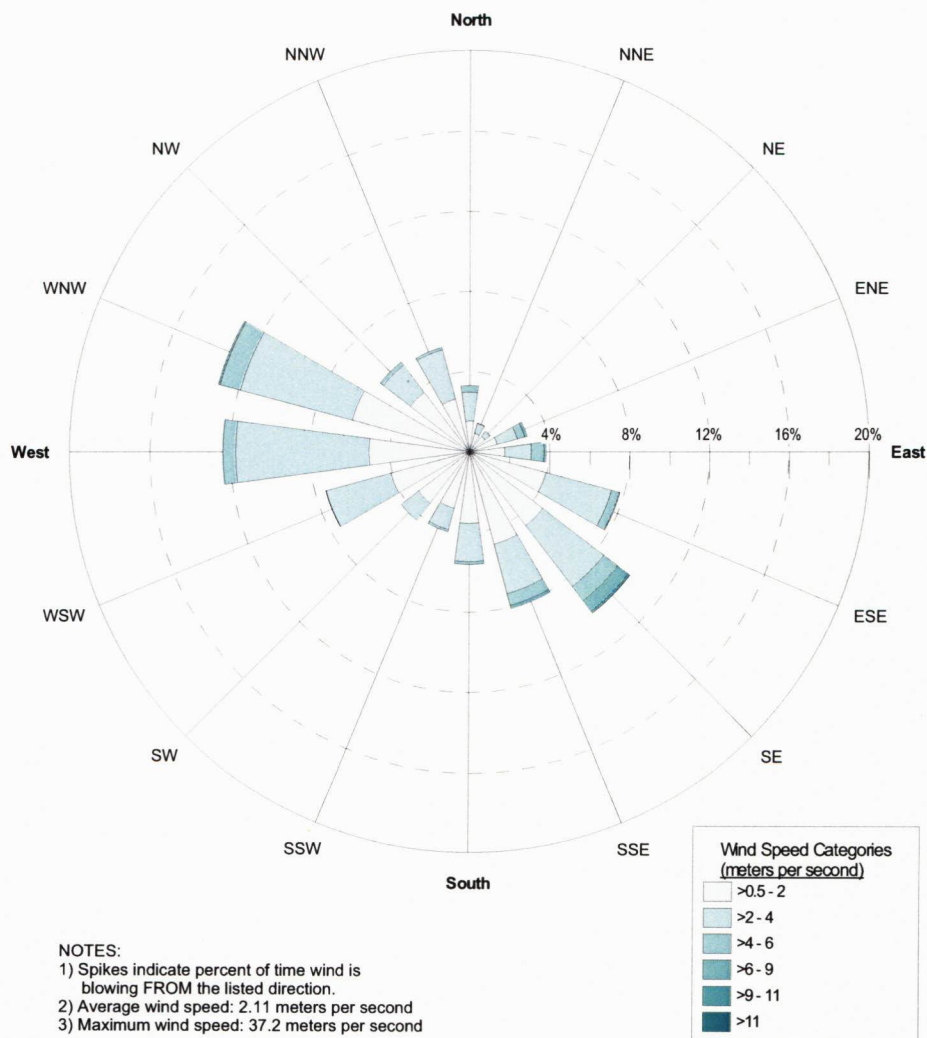
Figure 2-6 Annual Wind Patterns
