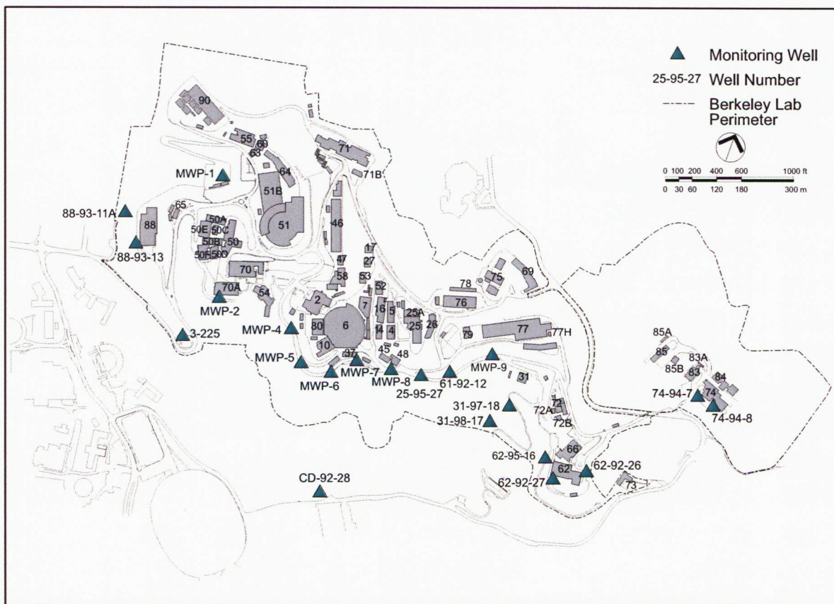
Figure 6-2 Approximate Locations of Monitoring Wells Closest to the Berkeley Lab Property Line
