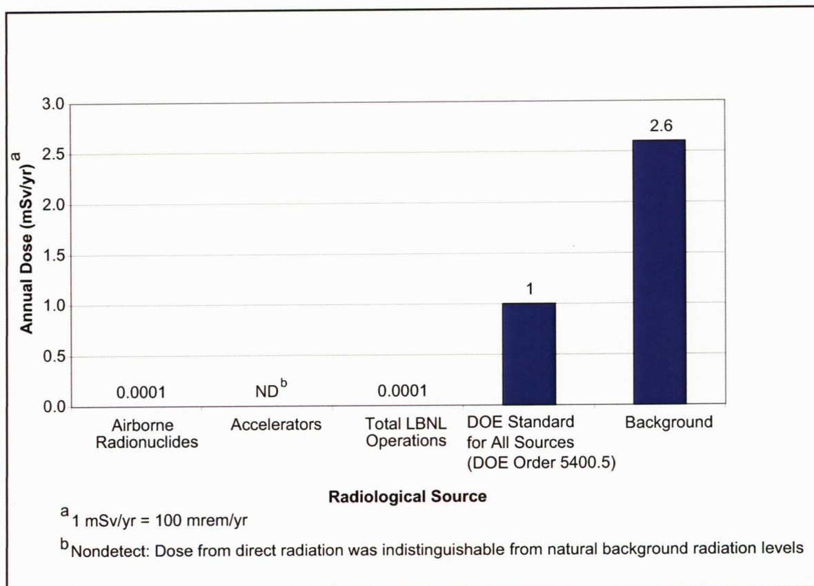
Figure 9-2 Comparison of Radiological Dose Impacts for 2004
