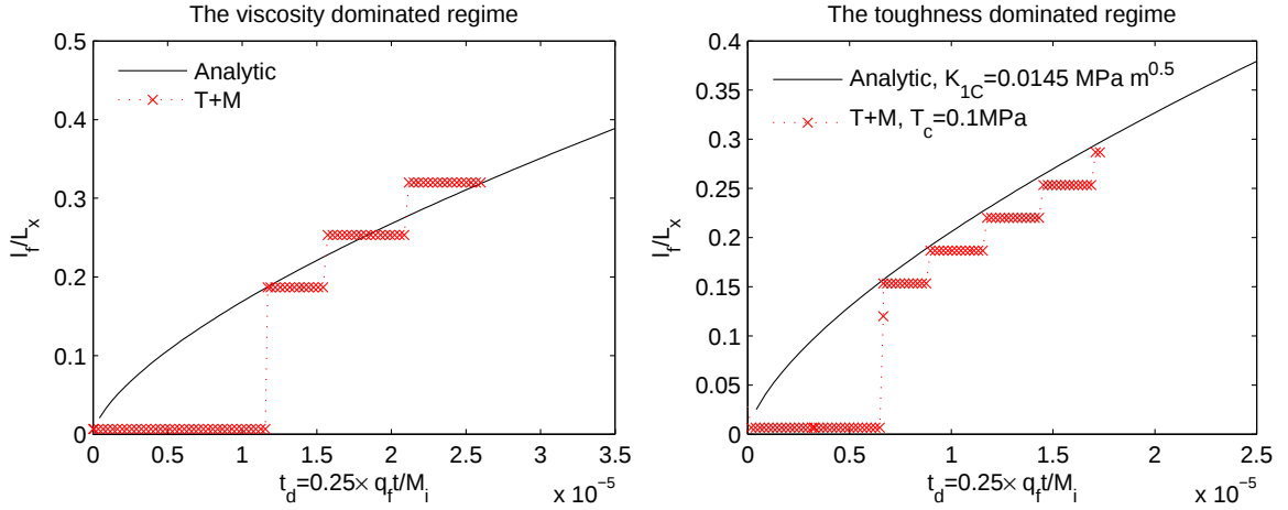
Figure 10: Comparison between the numerical solutions of T+M and the analytical solutions of the fracture propagation. Left: the viscosity dominated regime. Right: the toughness dominated regime. M_i is the initial mass of water in place. The numerical solutions match analytical solutions, validating T+M.
