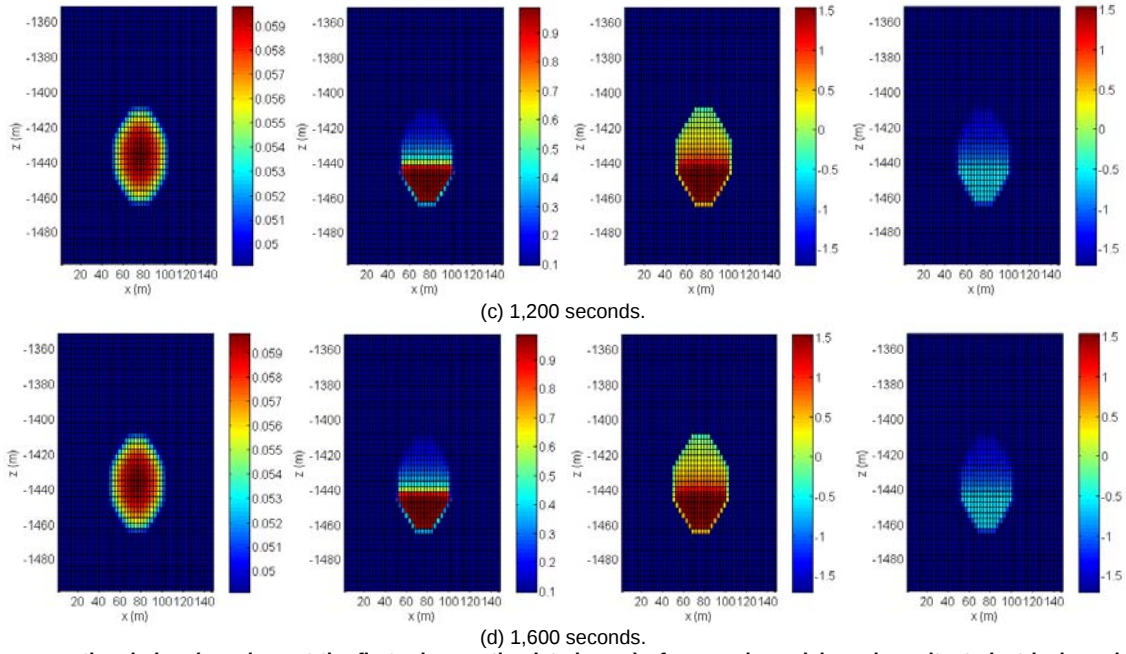
Fig. 11 Cross-sectional view (x-z plane at the first y layer, stimulated zone) of reservoir models and resultant electrical conductivity models. The 1 st column and the 2 nd column show changes in porosity and fluid saturation values over time, respectively. The 3 rd column shows changes in conductivity values when the electrically-engineered high-conductivity fluid (10,000 S/m) is injected. The 4 th column shows changes in conductivity values when the brine (3.33 S/m) is injected. At the top of the third column, the yellow vertical line segments indicate observation wells for the vertical crosswell EM configuration. Two yellow \otimes indicates the positions of horizontal wells for the horizontal crosswell EM configuration. The color charts for the 1 st and 2 nd column are linear and those for the 3 rd and 4 th column are based on the common log.
