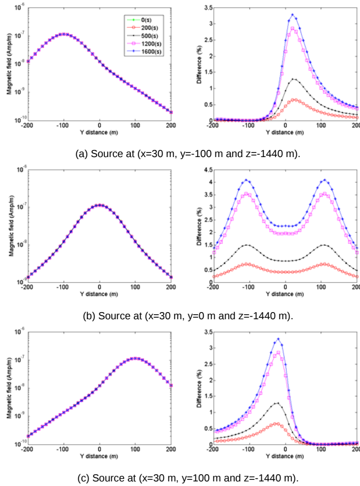
Fig. 16 Magnetic field amplitudes (the left column) and their relative difference (the right column) with respect to the background magnetic field when the horizontal crosswell configuration is applied to the conductivity model shown in the fourth column of Fig. 11. Receivers are placed along the axis that is parallel to the y-axis and passes through the point ( x=130 m and z=-1440 m).
