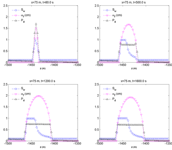
Fig. 9 Distributions of water saturation, aperture, dimensionless pressure ( p_d ) at x=75\text{m} . p_d = \frac{p - p_L}{p_U - p_L} , where p_U=40\text{MPa} and p_L=17.1\text{MPa} . The aperture is continuous along the fracture, while gas saturation is somewhat discontinuous. At early times, water fills almost all parts of the fracture, whereas gas takes up a considerable volume within the fracture at late times.
