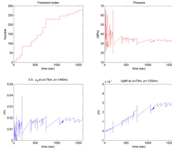
Fig. 7 Evolution of geomechanics and flow variables: (a) number of fractured nodes, (b) pressure at the injection point, (c) aperture of the fracture at the injection point, (d) displacement at (x=75m, z=-1350m). Fracturing events are discontinuous, which results in fluctuation in pressure and the aperture. The oscillation is more dominant at early times due to small volume of the fracture.
