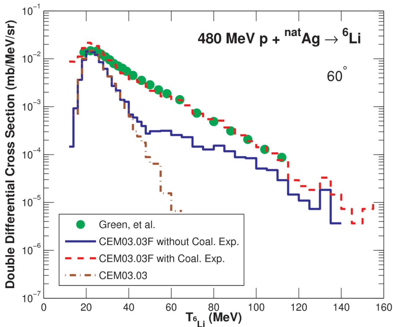
Fig. 3. Comparison of experimental results of the reaction 480 MeV p + nat Ag → 6 Li at 60° by Green et al. [17] (green circles), with simulations from the original CEM03.03 (brown dashed-dotted lines), CEM03.03F without coalescence expansion (blue solid lines) and the CEM03.03F with coalescence expansion (red dashed lines).
