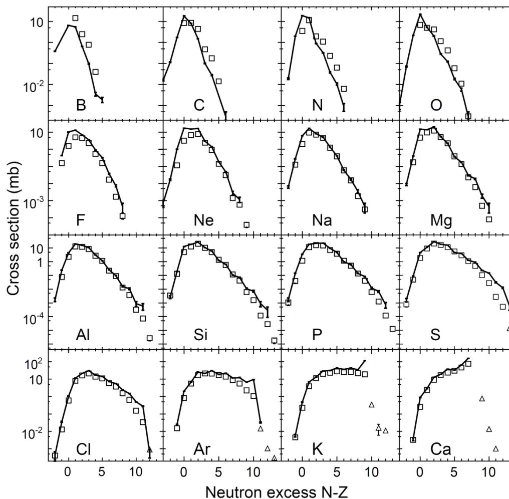
Figure 12: Measured cross sections for ^{48}\text{Ca} fragmentation on ^9\text{Be} at 140 MeV/nucleon [49,50] compared with LAQGSM03.03 predictions.
