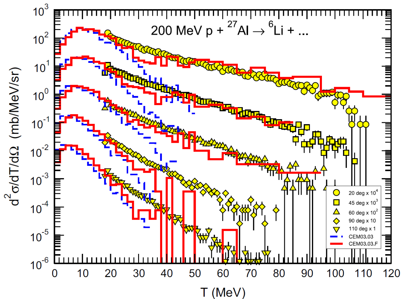
Fig. 27. Comparison of experimental {}^6\text{Li} spectra at 20, 45, 60, 90, and 110° by Machner et al. [61] (symbols) with calculations by the unmodified CEM03.03 (dashed histograms) and preliminary results with the modified MEM in CEM03.03.F (solid histograms), as indicated.
