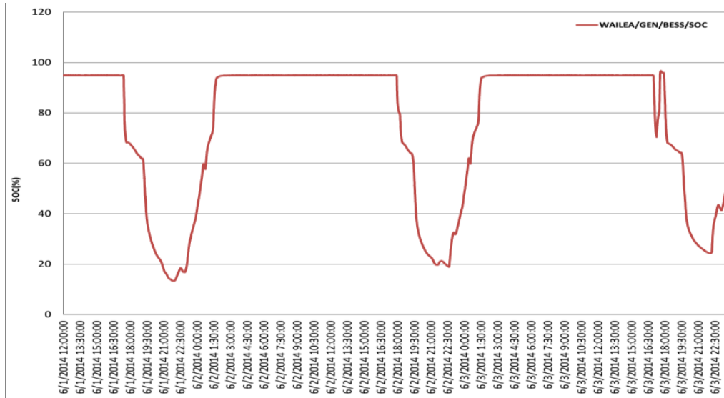
Figure 6-70: BESS SOC for manual peak shaving mode
