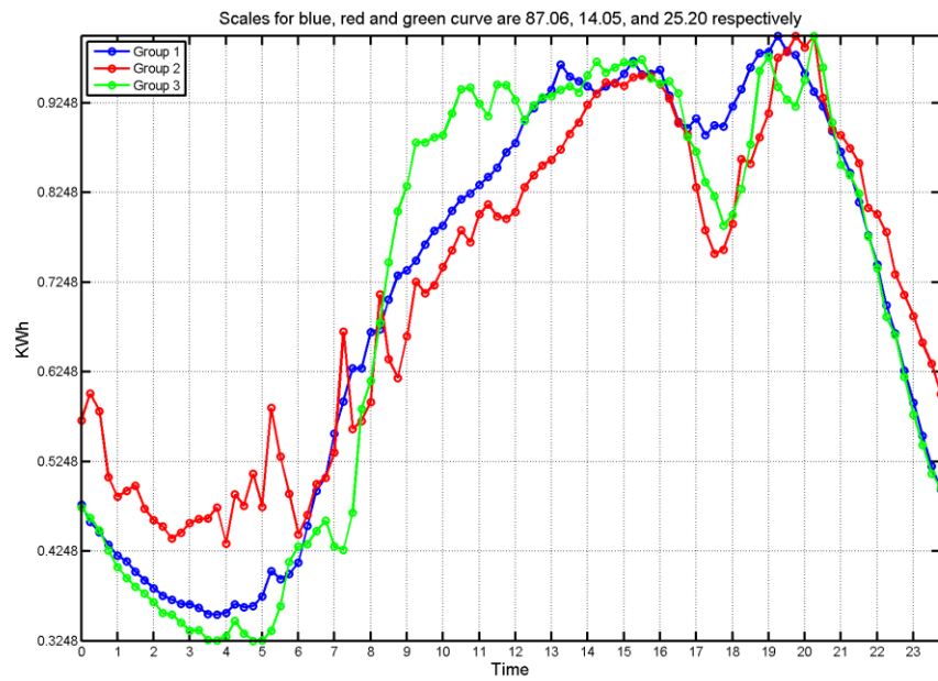
Figure 6-14: Average daily load profile for participant homes by group
