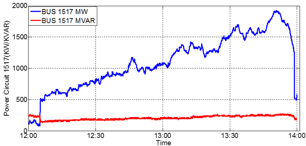
Figure 6-50: The voltage profile for active power absorption
