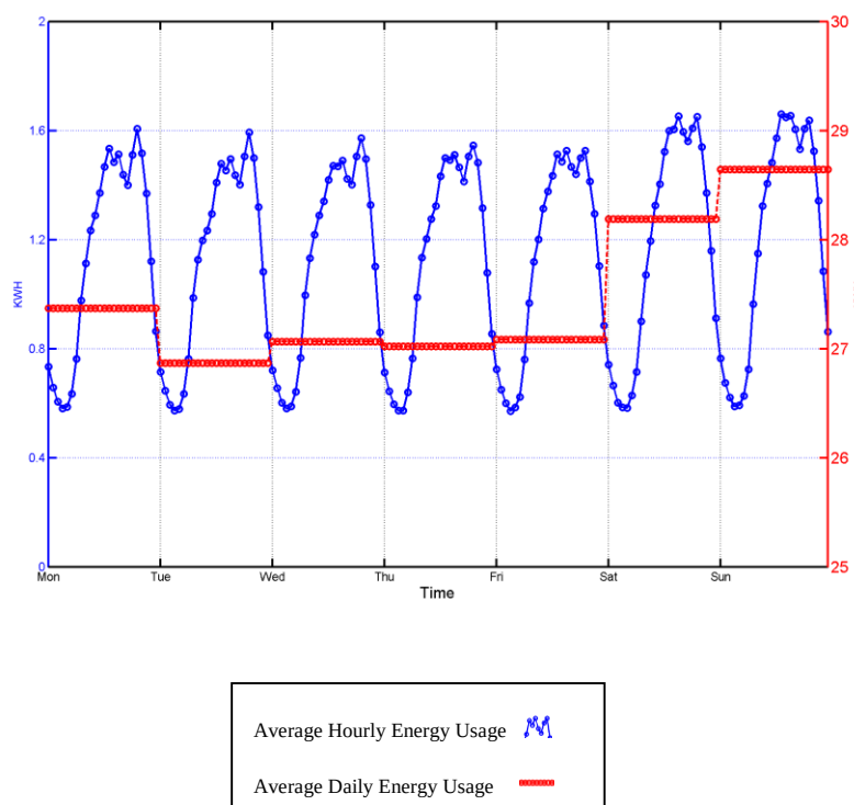
Figure 6-16: Average weekly household load profile for participant homes in group 1
