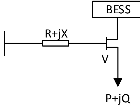
Figure 6-66: System schematic
