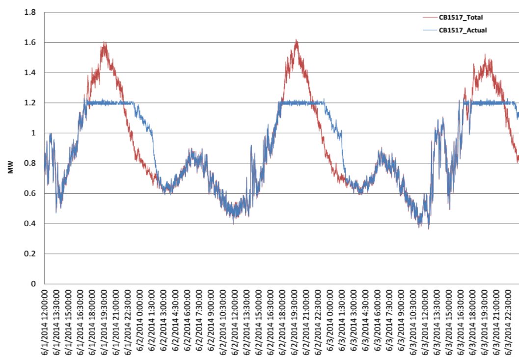
Figure 6-69: Bus 1517 – active power
