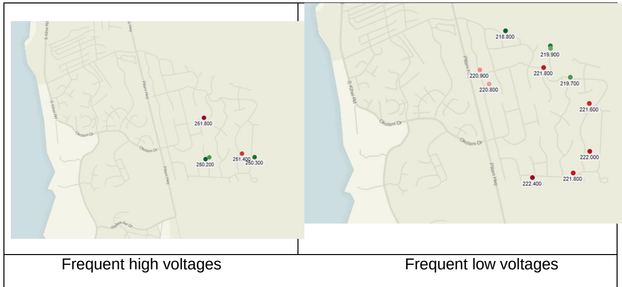
Figure 6-17: Observed out of limit voltages on Feeder 1517
