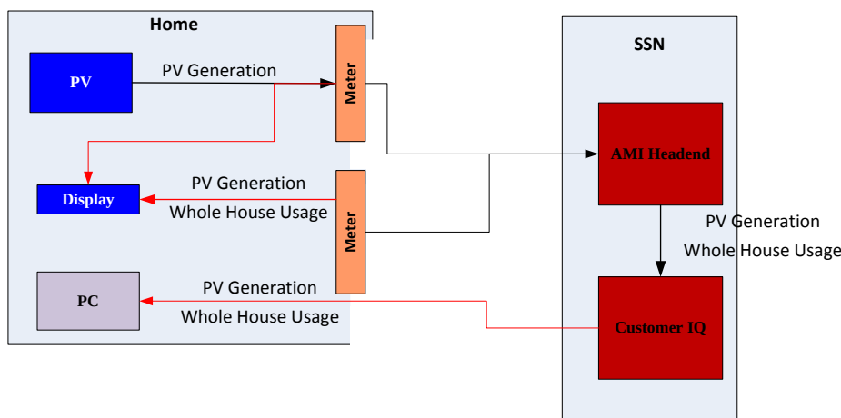
Figure 3-7: PV Monitoring Data Flow
