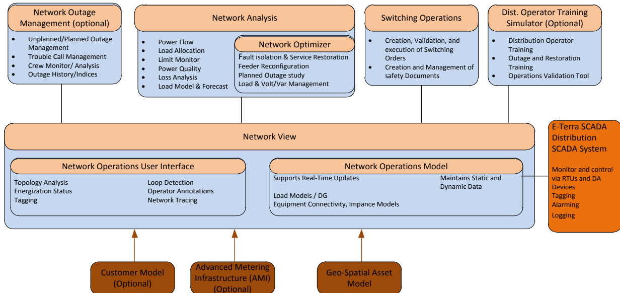
Figure 3-11: Alstom System Modules
