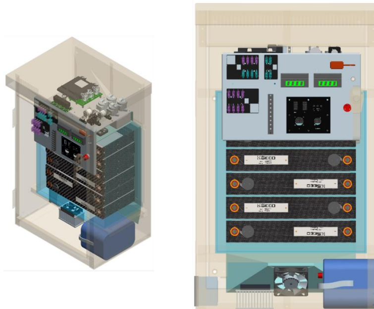
Figure 14: Architecture of Seeo 10 kWh Energy Storage System
