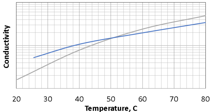
Figure 10: Conductivity comparison of a material developed under this program to that of the conventional polymer electrolyte.
