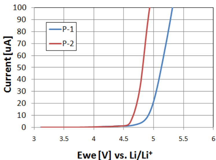
Figure 13: Cyclic voltammetry results of two of Seeo's catholyte polymers.
