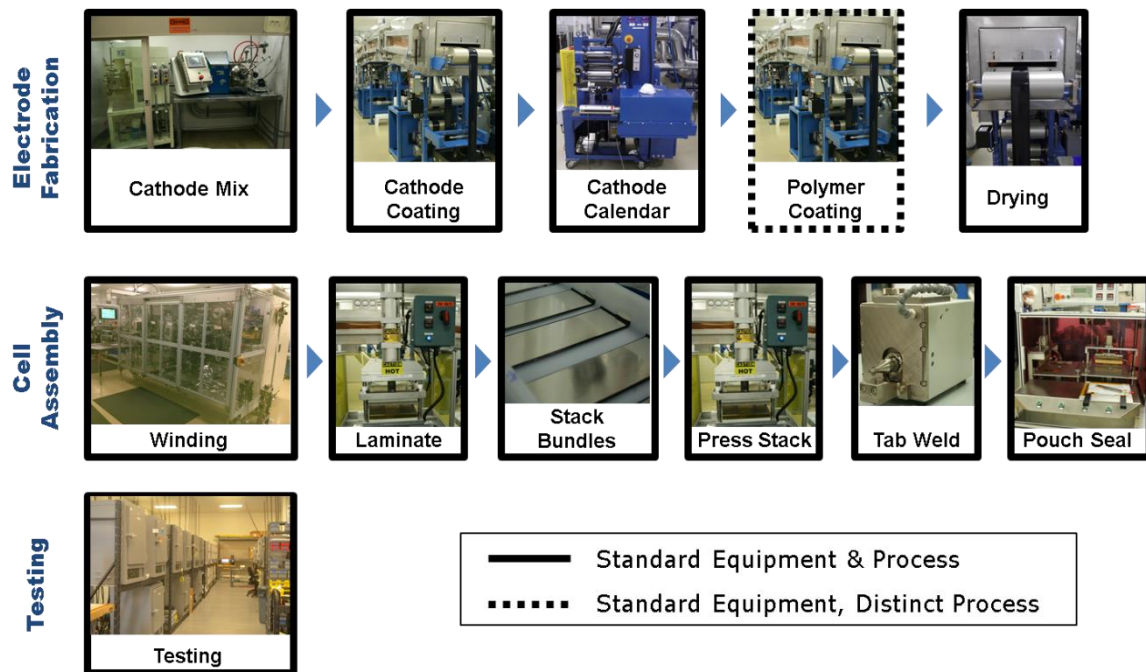
Figure 6: Process Flow – Seeo Pilot Manufacturing Line
