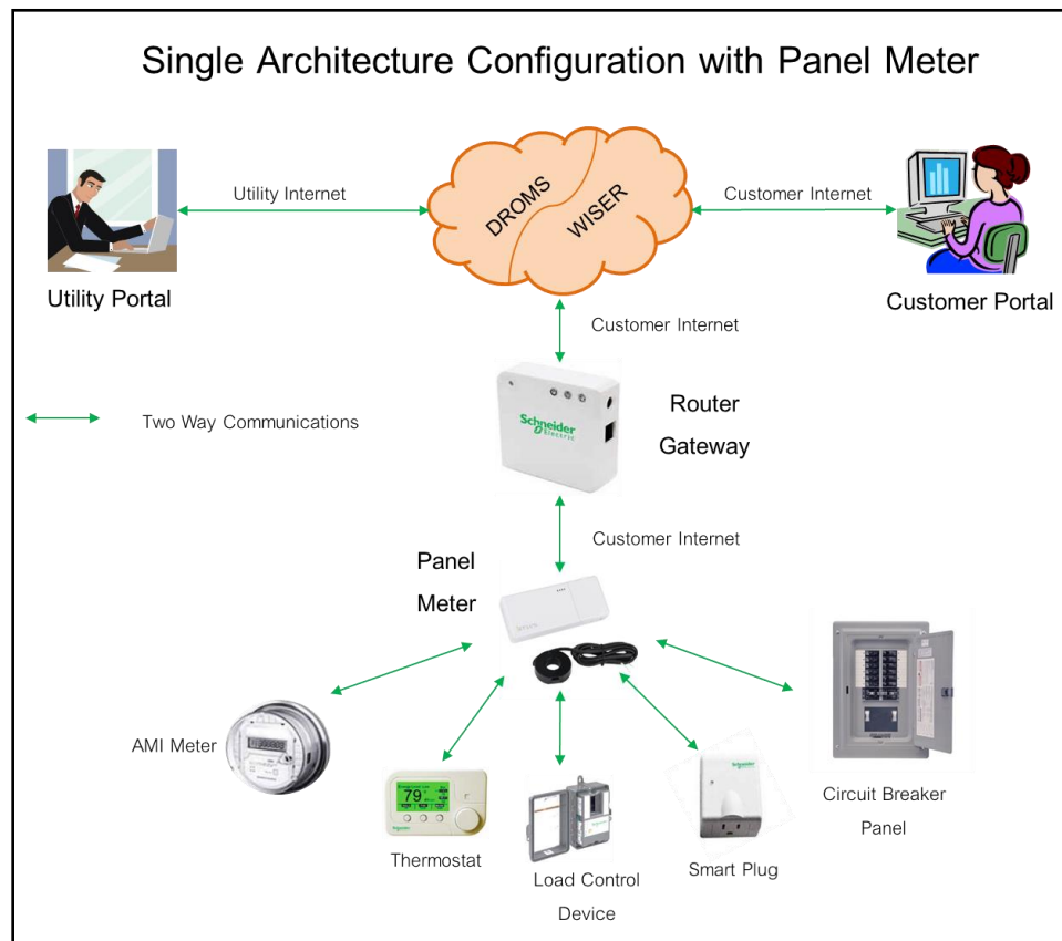
Figure 16 – PSEG Long Island DLC System Single Architecture with Panel Meter
