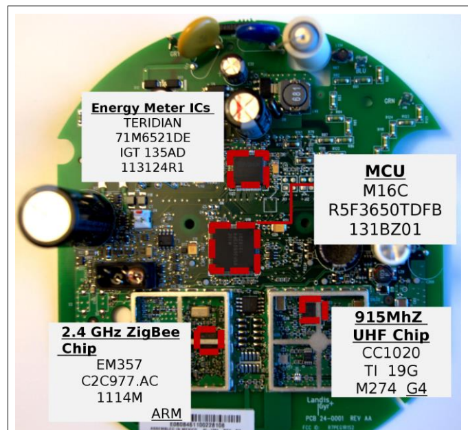
Figure 36 - L+G Gridstream Smart Meter
