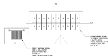
(c) Solar Panel Layout
