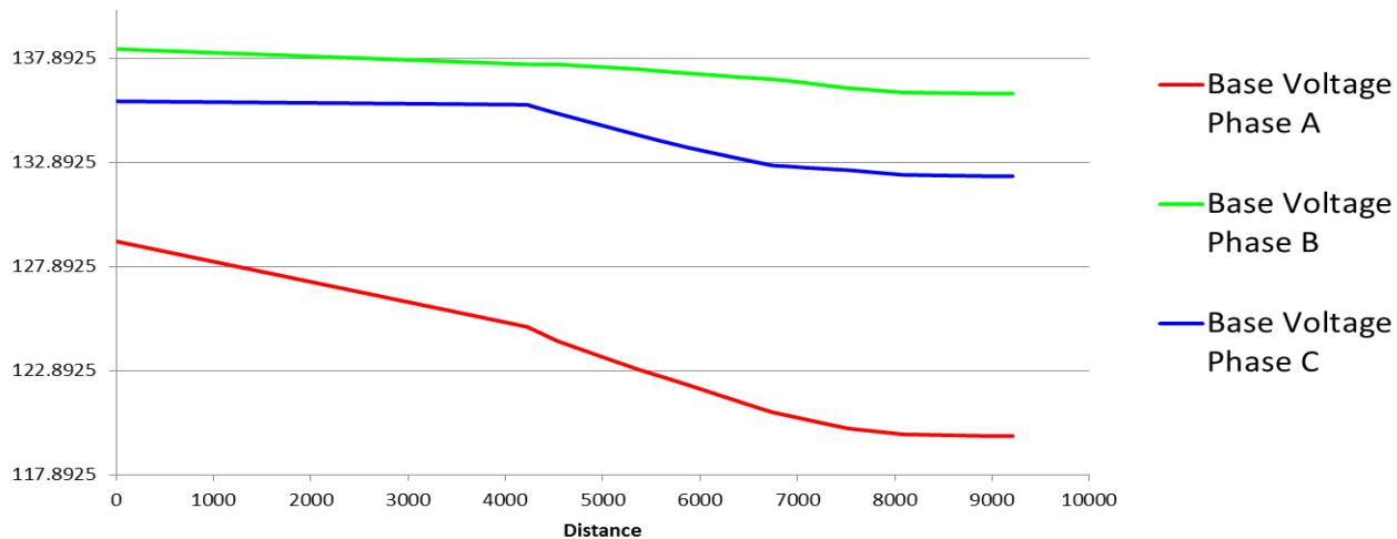
Figure 35 - Voltage Profile with the Spot Load Model
