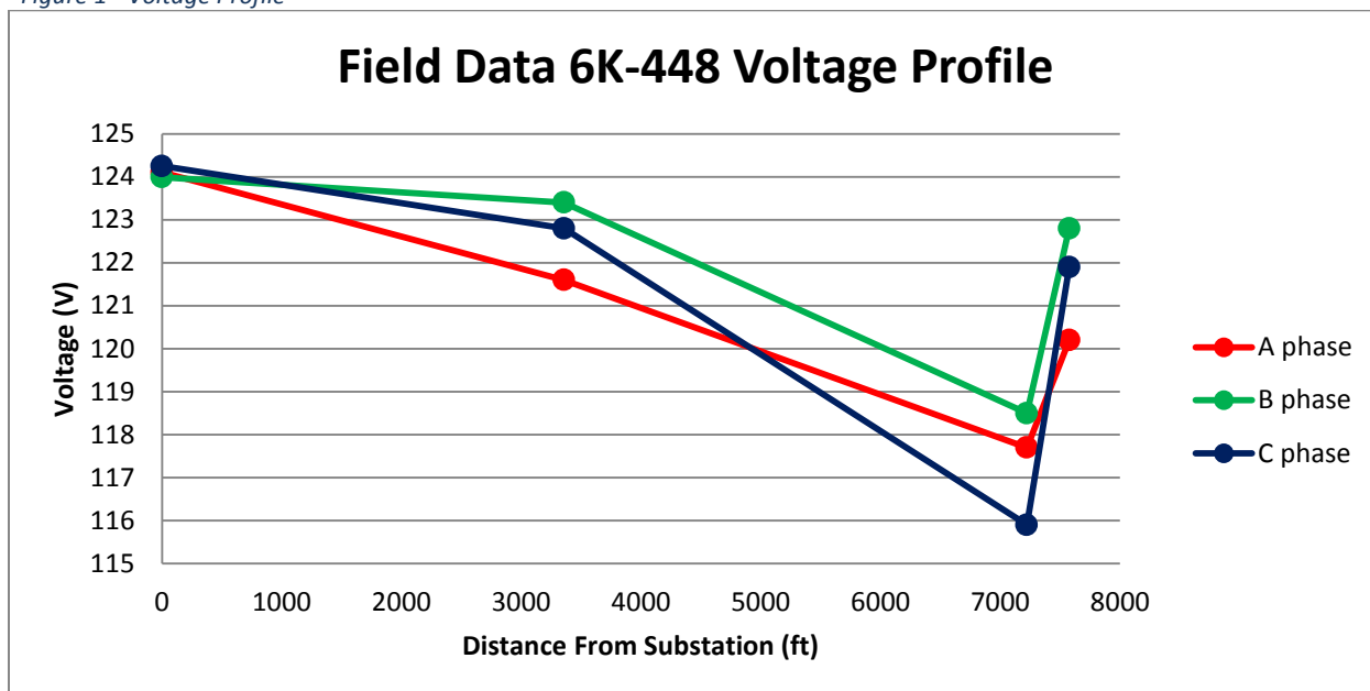
Figure 2 – Voltage Profile
