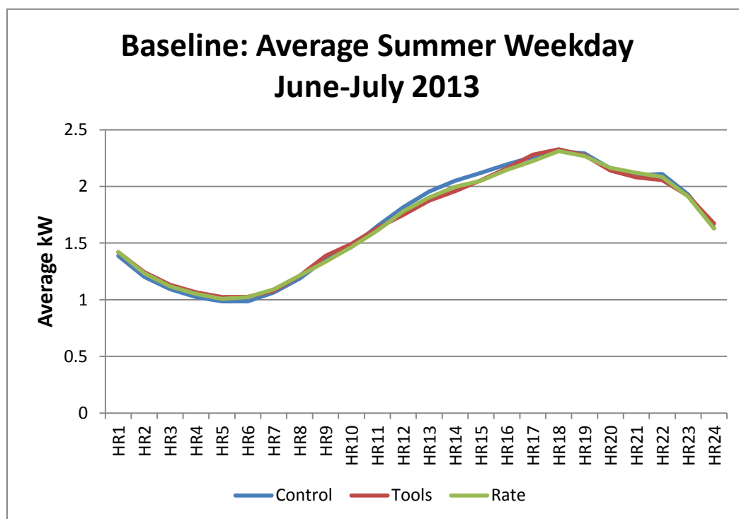
Figure 13 - Baseline Study of Customer Load by Group
