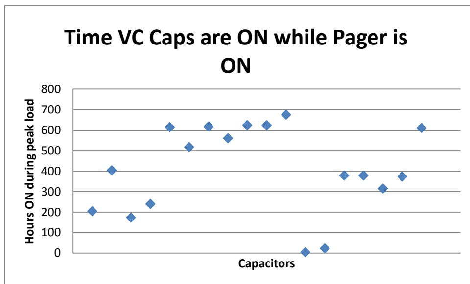
Figure 7 - Time VC Caps On while Pager is On
