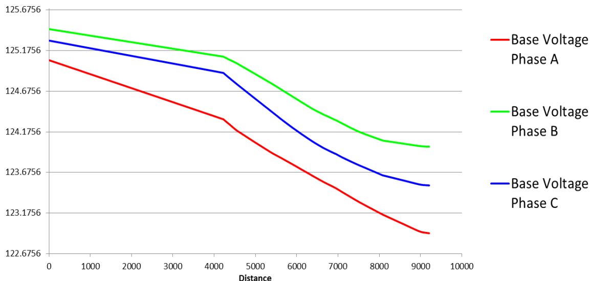
Figure 34 - Voltage Profile with the Traditional Method
