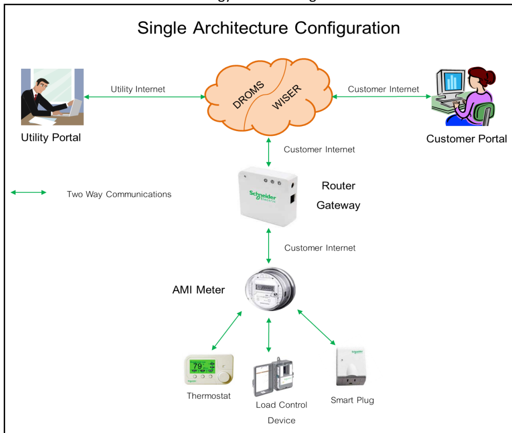
Figure 15 – PSEG Long Island DLC System Single Architecture
