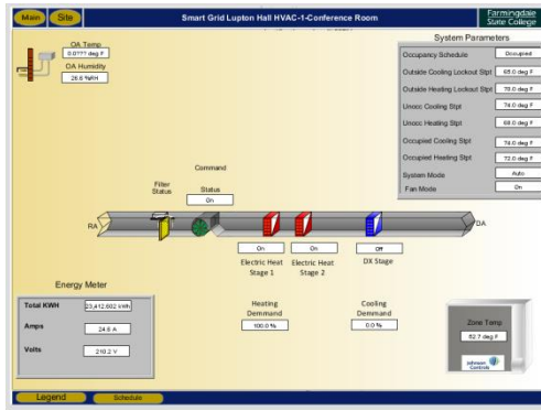
(a) Johnson Controls Screenshot: HVAC Status and Energy Monitoring Screen
