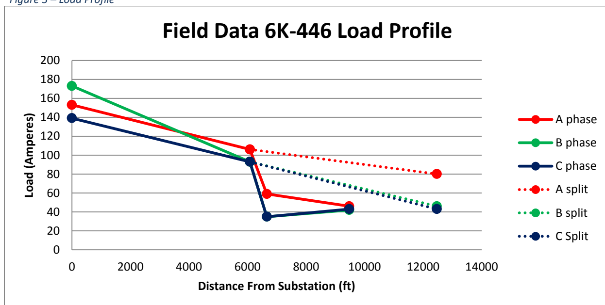
Figure 4 – Load Profile
