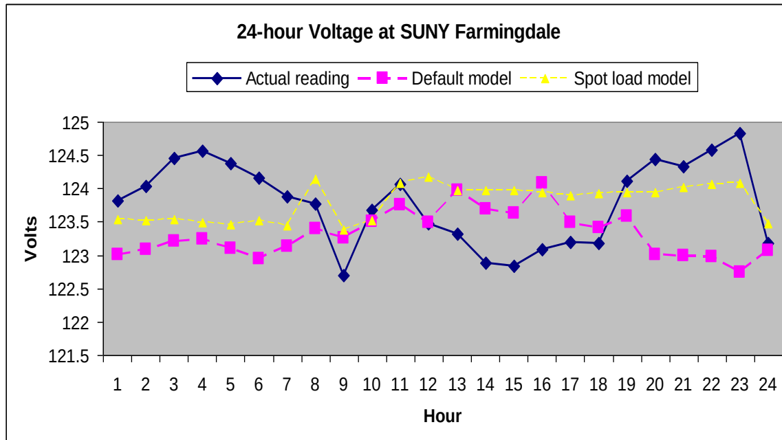
Figure 29 - 24-Hour Voltage at SUNY Farmingdale
