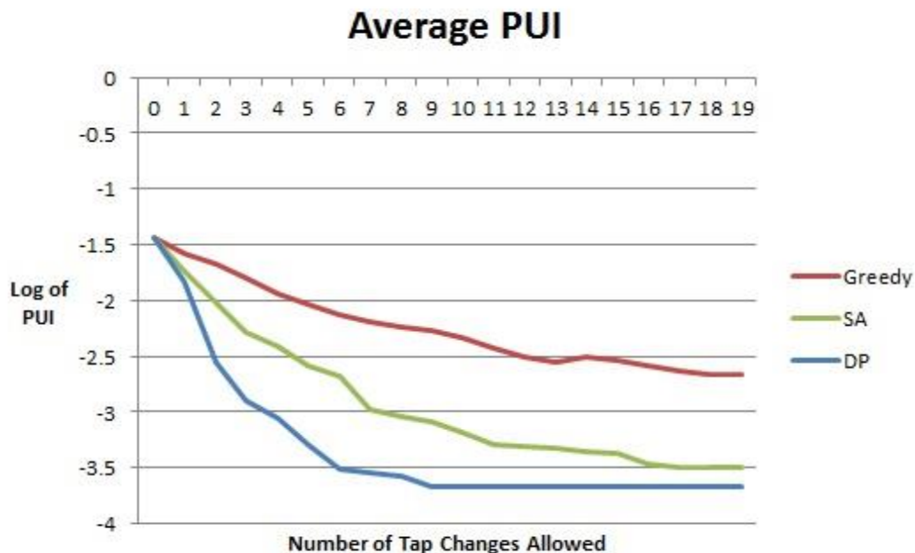
Figure 33 - Average PUI as the Number of Tap Changes Allowed is Varied
