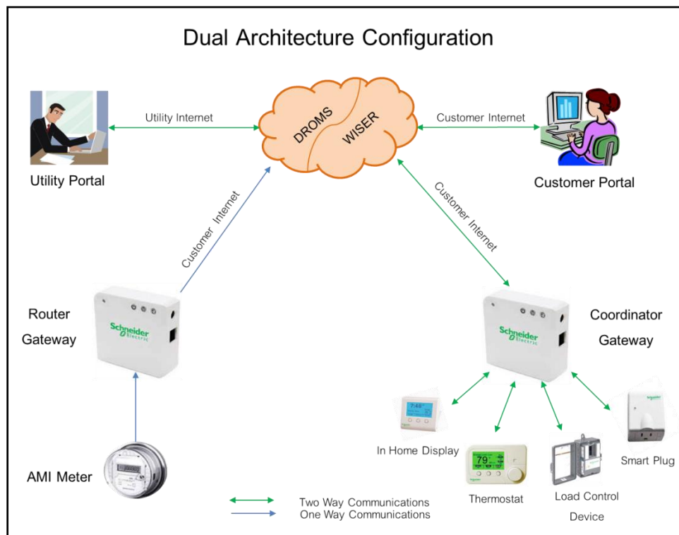
Figure 17 – PSEG Long Island DLC Dual System Architecture
