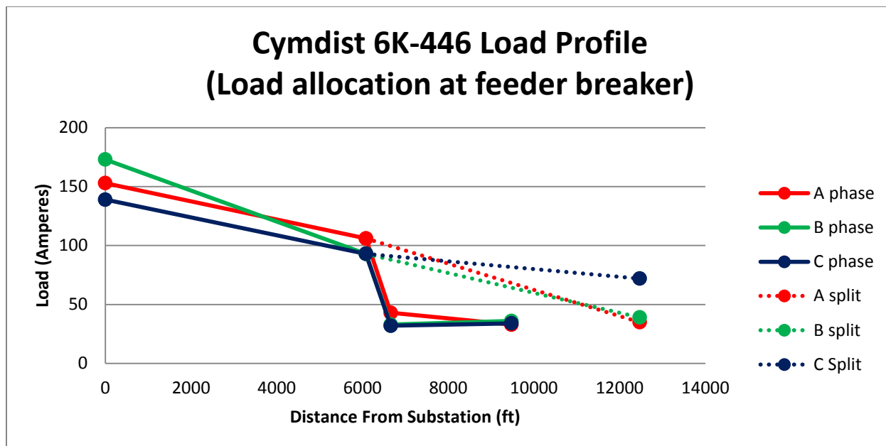
Figure 3 – Load Profile
