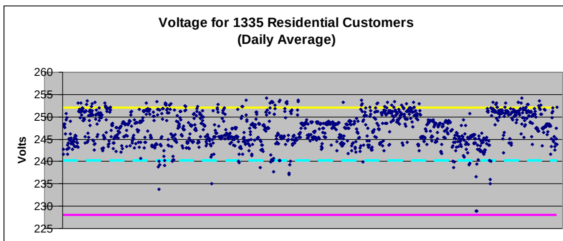
Figure 30 - Voltage for 1335 Residential Customer (Daily Average)
