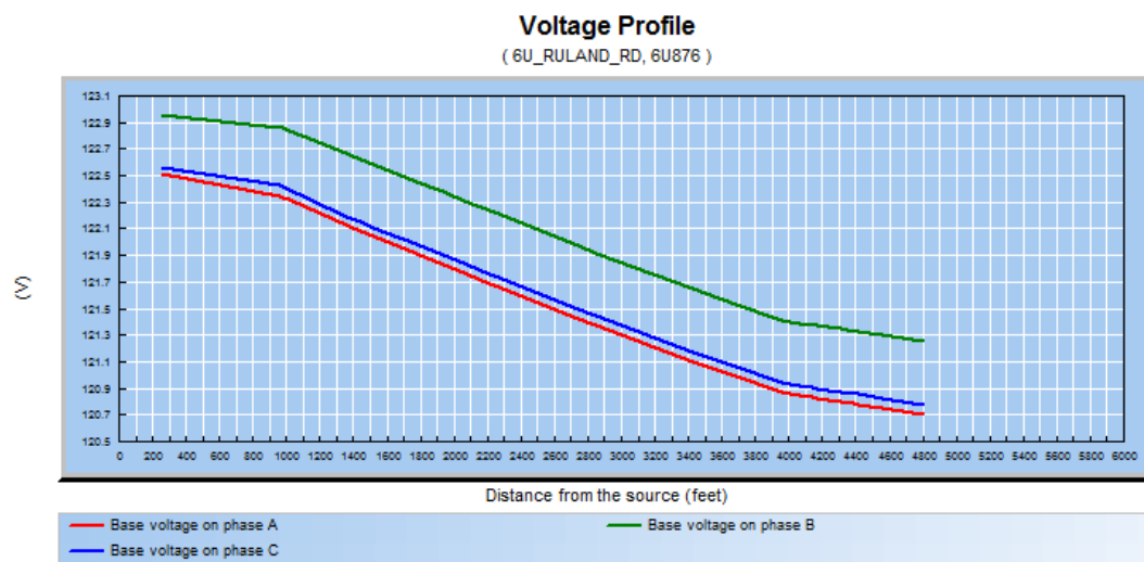
Figure 25 - Voltage Profile When Capacitor Banks Are Switched On
