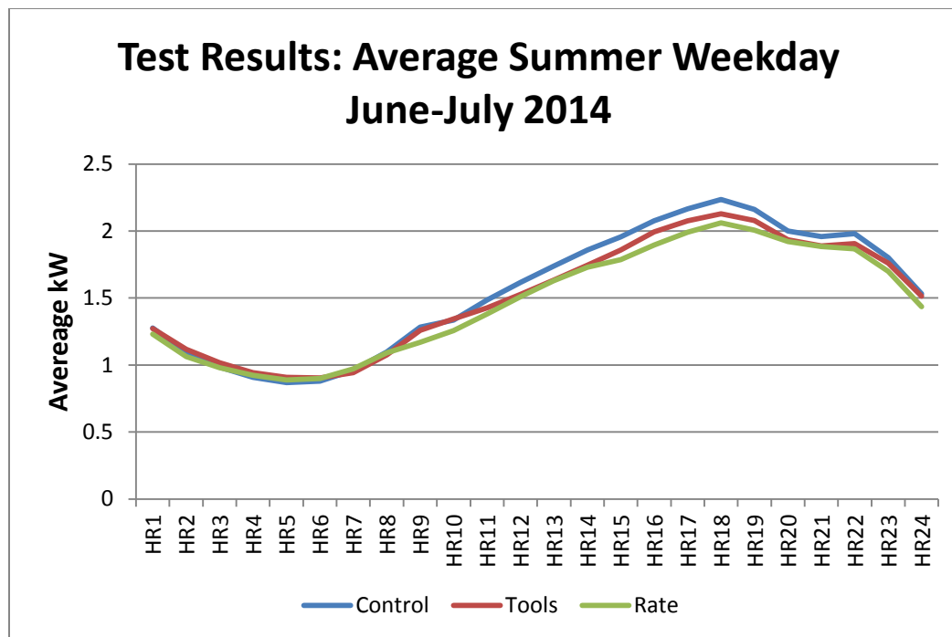
Figure 14 - Results Study of Customer Load by Group
