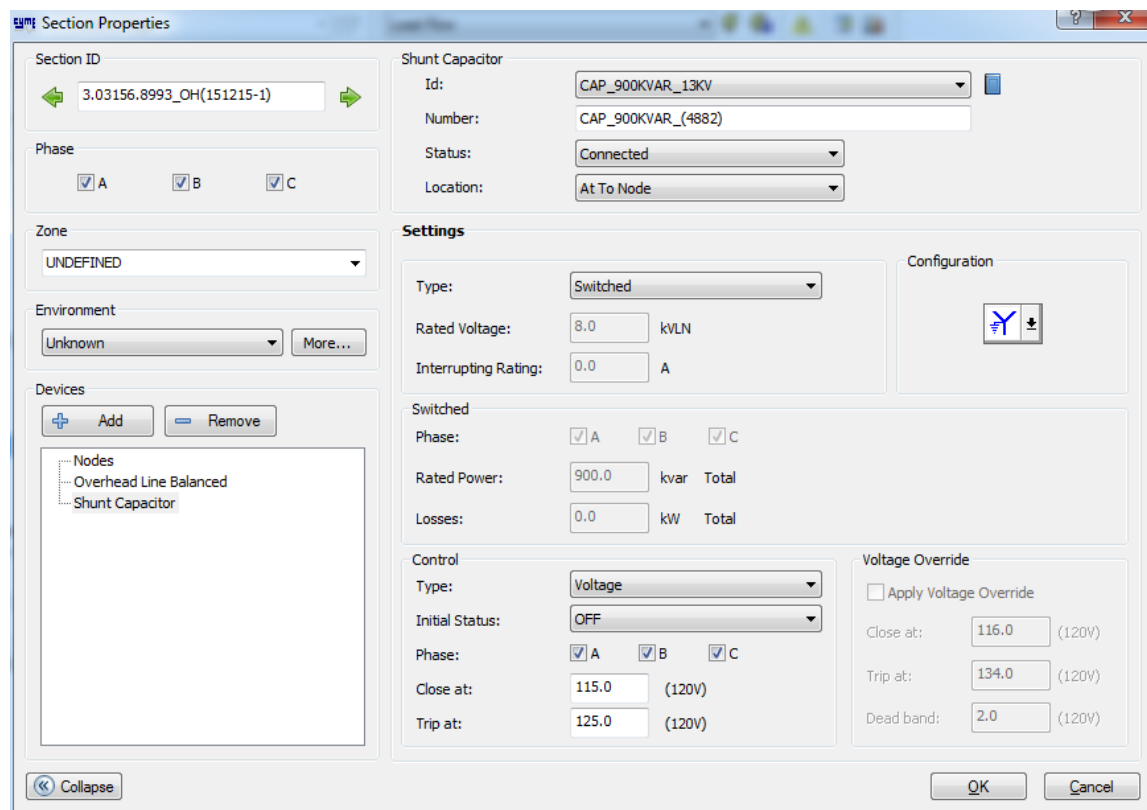
Figure 23 - Screenshot in CYME to Control Capacitor Banks
