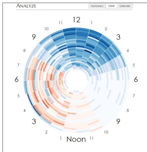
Figure 44 - Radial Heat-Map of Smart Meter Data to Identify Periodical Patterns. Here, Darker Shades Represent Greater Energy Consumption. This House in Particular Shows Significantly More Night Time Consumption Than Days – A Pattern Not Evident from Traditional Line Plots
