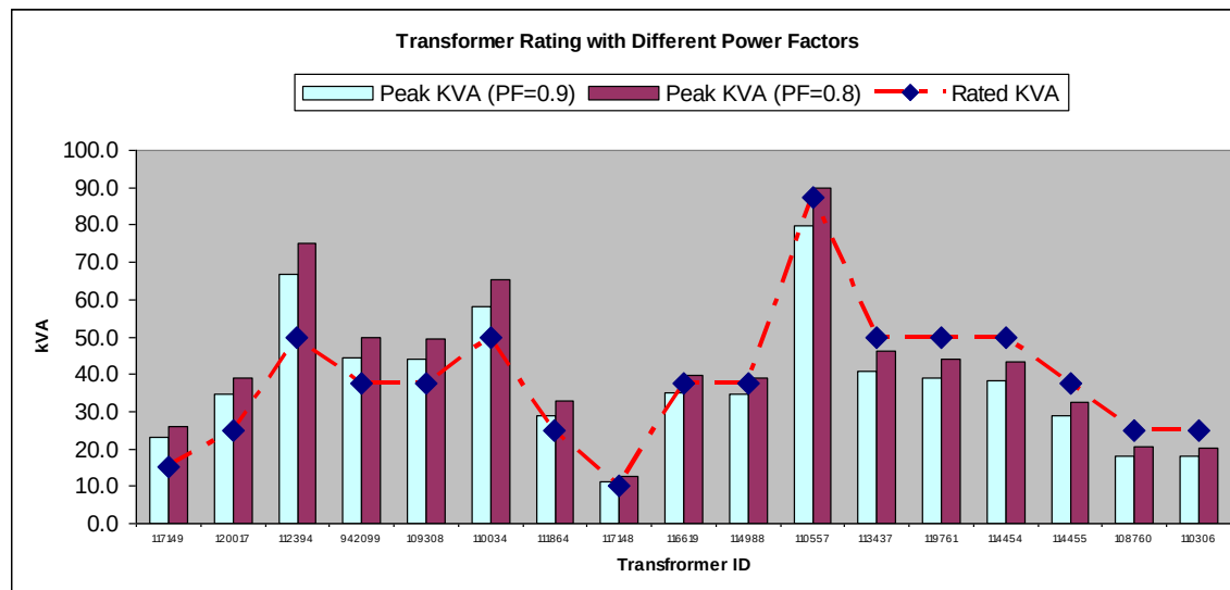
Figure 28 - Transformer Rating with Different Power Factors
