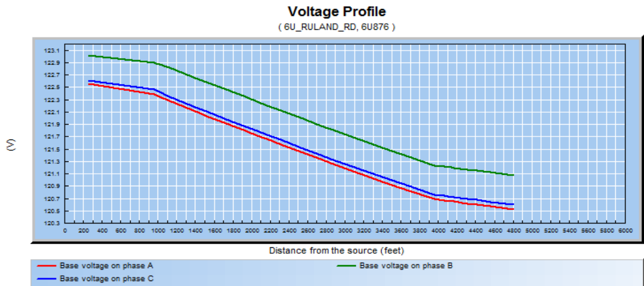
Figure 24 - Voltage Profile When Capacitor Banks Are Switched Off
