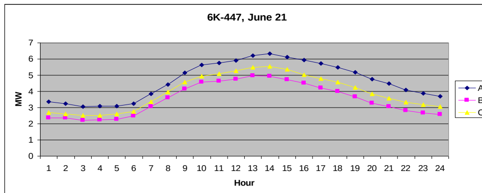
Figure 26 - Load Shape of 6K-447 on June 21, 2012
