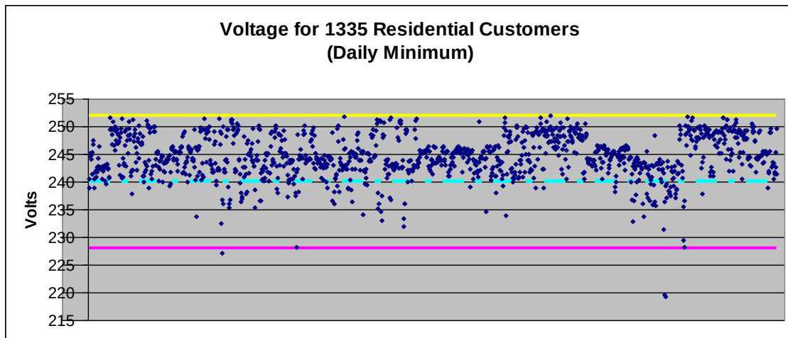
Figure 31 - Voltage for 1335 Residential Customer (Daily Minimum)
