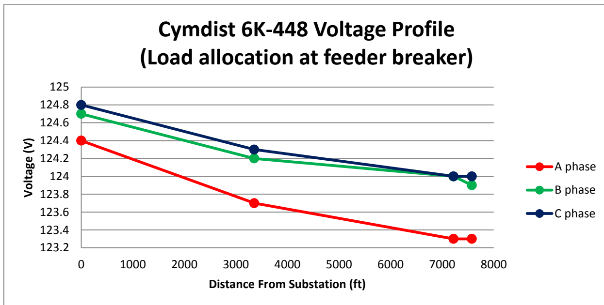
Figure 1 - Voltage Profile
