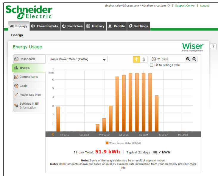
Figure 19 - Wiser Usage Dashboard
