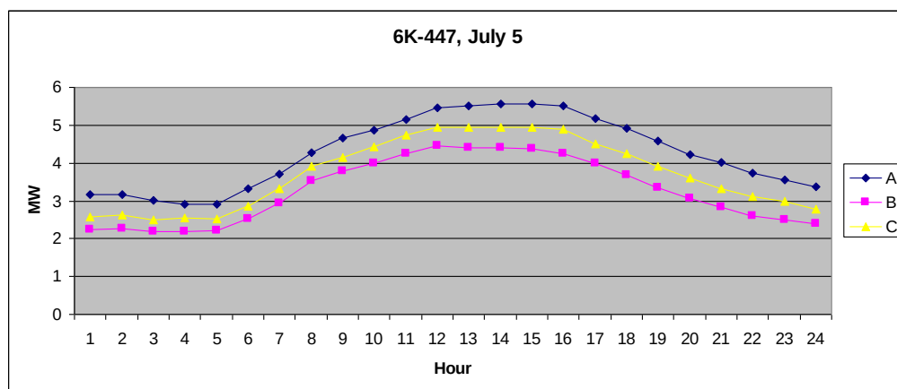
Figure 27 - Load Shape of 6K-447 on July 5, 2012
