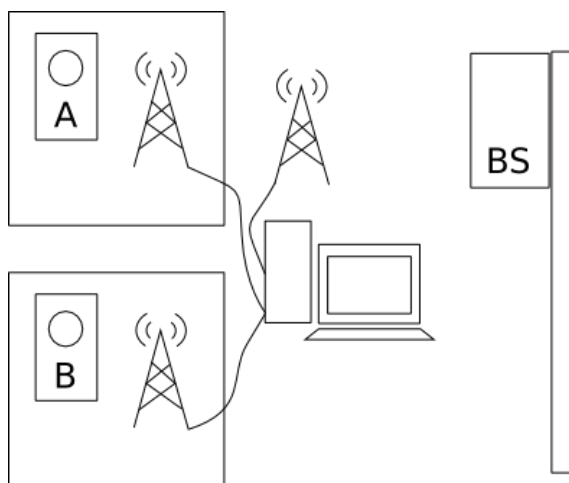
Figure 37 – isolation Chambers
