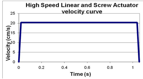
Figure 2: Velocity Profile
