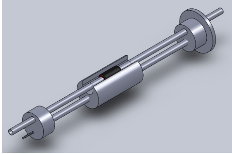
Figure 3: Original Pilot Rod Design
