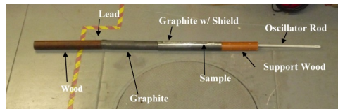
Figure 5: Oscillator Pieces
