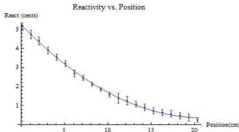
Figure 8: Calibration of Pilot Rod
