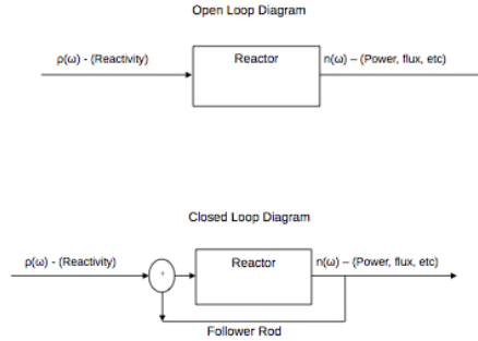
Figure 1: Open Loop and Closed Loop Schematic
