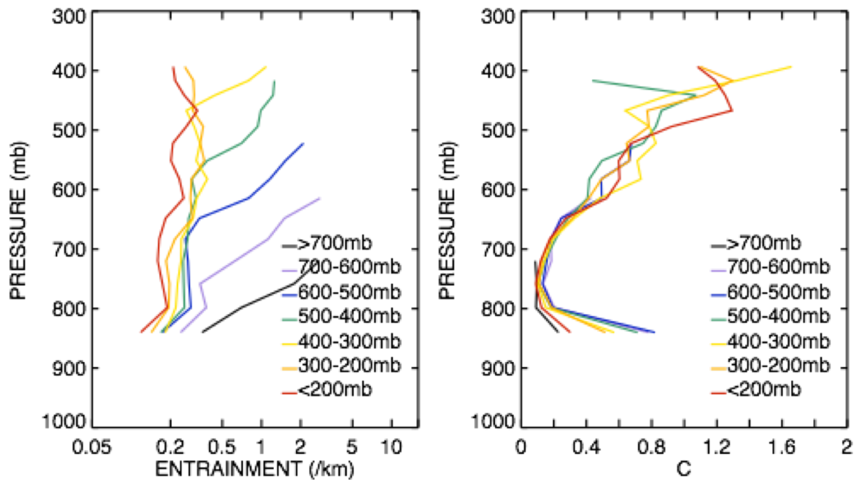
Fig. 2. Left panel: Entrainment rates inferred from the moist static energy profile within convective columns penetrating to different pressure levels as simulated by the WRF model for the TWP-ICE break period (Del Genio and Wu, 2010). Right panel: Parameterization test from the same simulation showing that a single vertical profile of the proportionality constant in the Gregory (2001) entrainment parameterization works generally for all types of convection.
