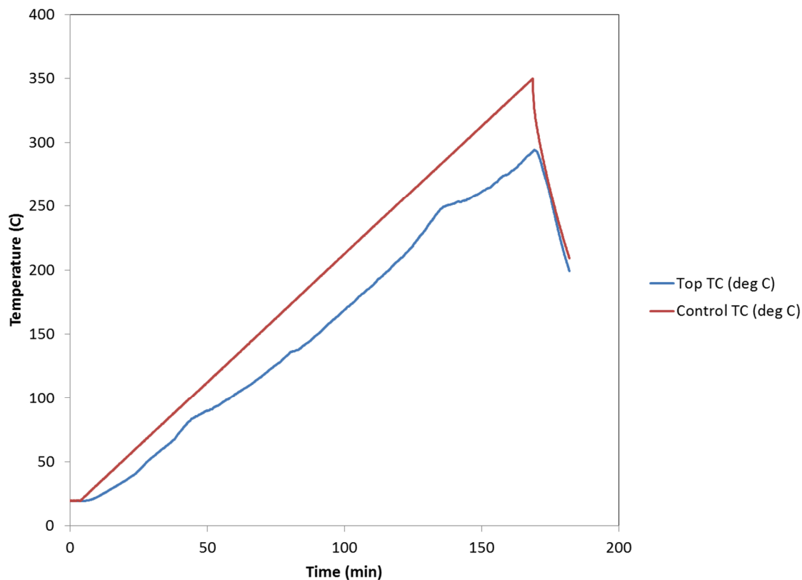
Figure 48. Temperature data from Exp405. The contents were the same as Exp404 (LANL WB-4 mixture without Pb or Cr) and the test was open.
