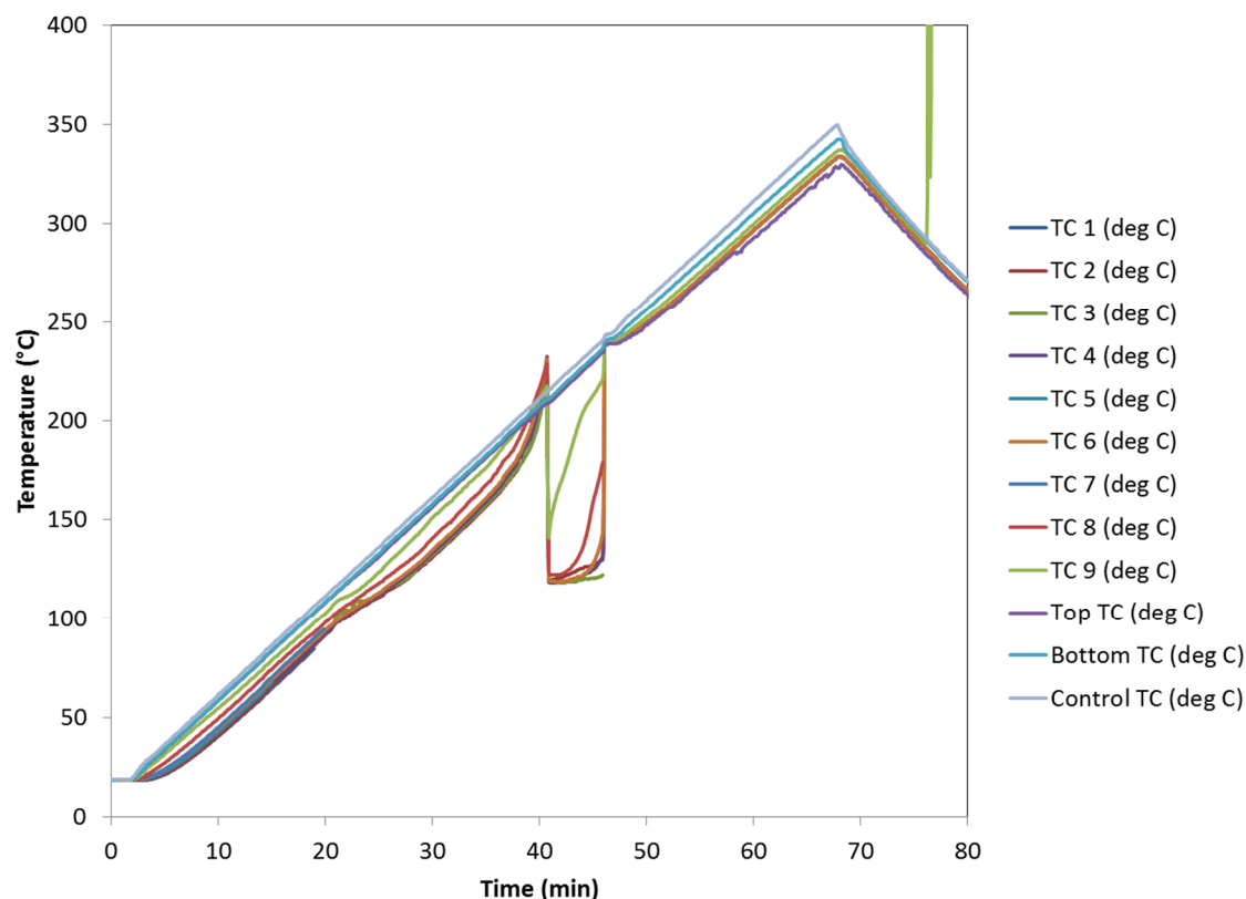
Figure 19. Exp394 temperature data. Contents were over-neutralized acid, Swheat, magnesium nitrate hexahydrate, and sodium nitrate. The amount of nitrate salts was about three times more than should have been.
