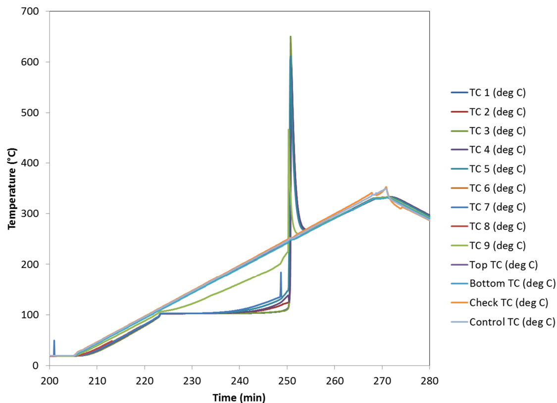
Figure 33. Temperature data from Exp399. Contents were Swheat, over-neutralized acid, Na nitrate, and Mg nitrate.
