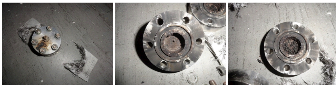
Figure 58. Post-test debris from Exp408.
