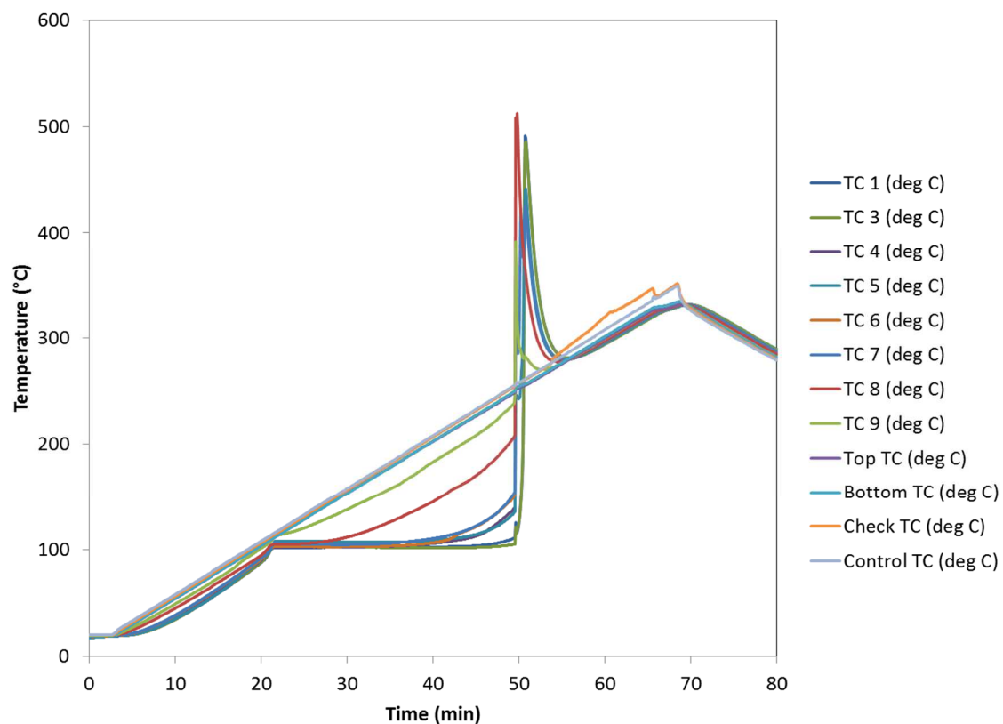
Figure 25. Exp396 temperature data. Contents were over-neutralized acid, Swheat, magnesium nitrate hexahydrate, and sodium nitrate.
