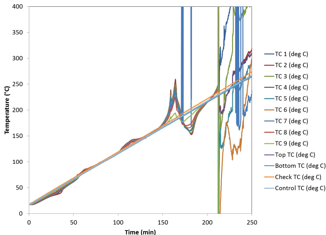
Figure 65. Temperature data from Exp411. Contents were the LANL WB-4 mix without water, Pb, or Cr. Heating rate was 1°C/min.
