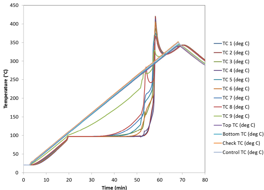
Figure 6. Exp388 temperature data. Contents were neutralized acid and Swheat.
