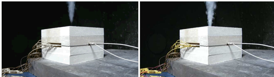
Figure 7. Frames from Exp388 video showing two jets.
