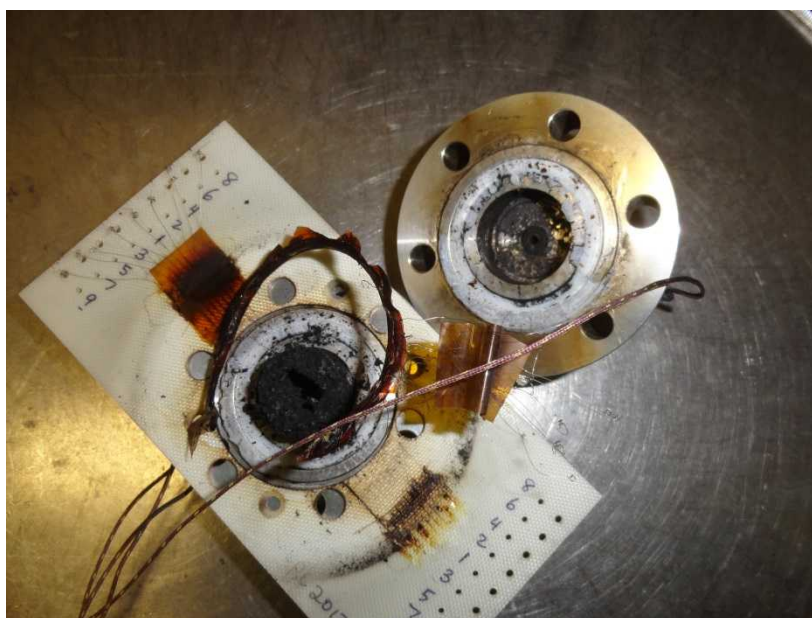
Figure 24. Post-test debris from Exp395. The Teflon O-rings appear to be intact, indicating that the violent release that launched the top insulation block occurred only through the top vent.
