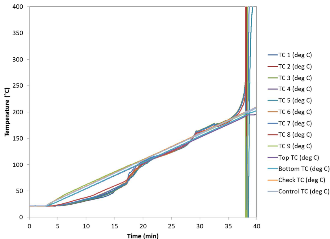
Figure 42. Temperature data from Exp403. Contents were based on the LANL WB-4 mix: Ca nitrate, Cr nitrate, Fe nitrate, Mg nitrate, Na nitrate, Pb nitrate, oxalic acid, and Swheat. No liquids were added.
