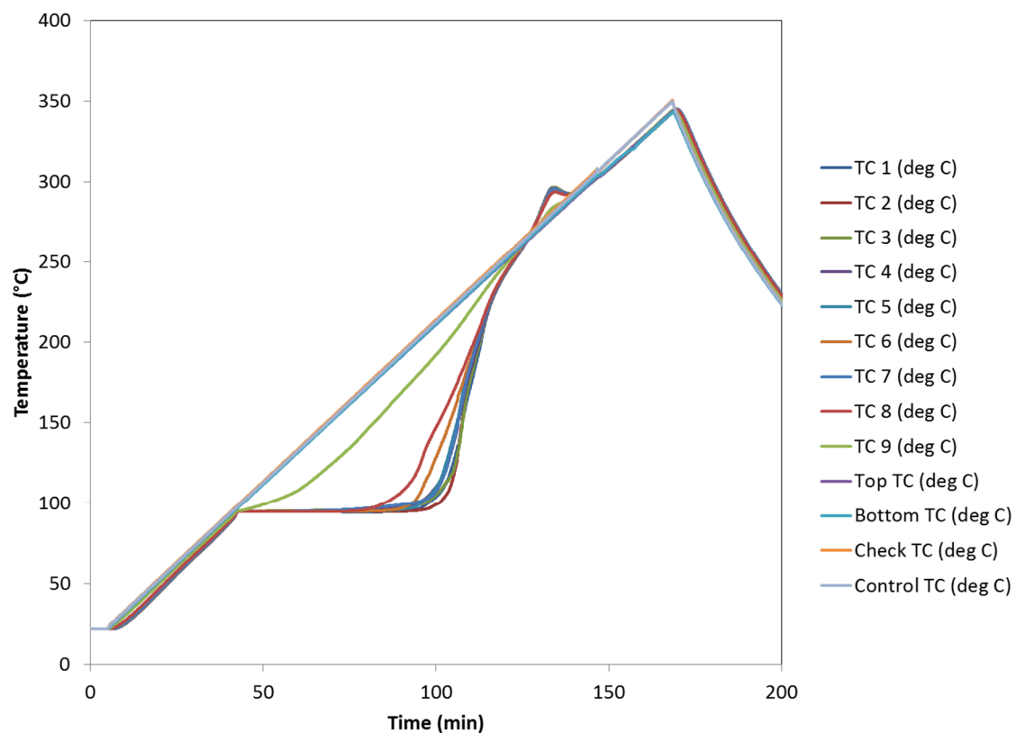
Figure 4. Exp387 temperature data. Contents were Swheat and DI water. The heating rate was 2°C/min.
