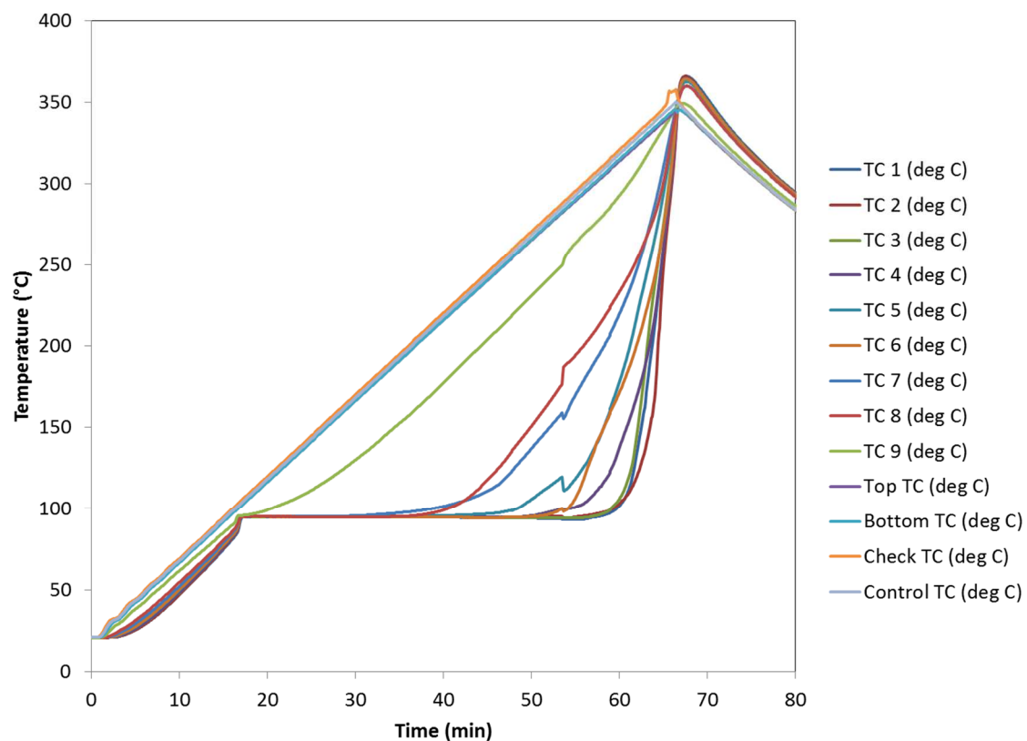
Figure 9. Exp389 temperature data. Contents were water and Swheat.
