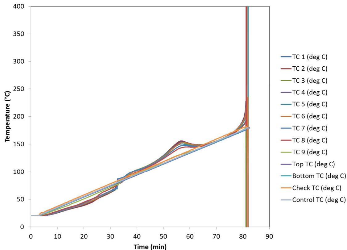
Figure 62. Temperature data from Exp410. Contents were the LANL WB-4 mix without water, Pb, or Cr. Heating rate was 2°C/min.
