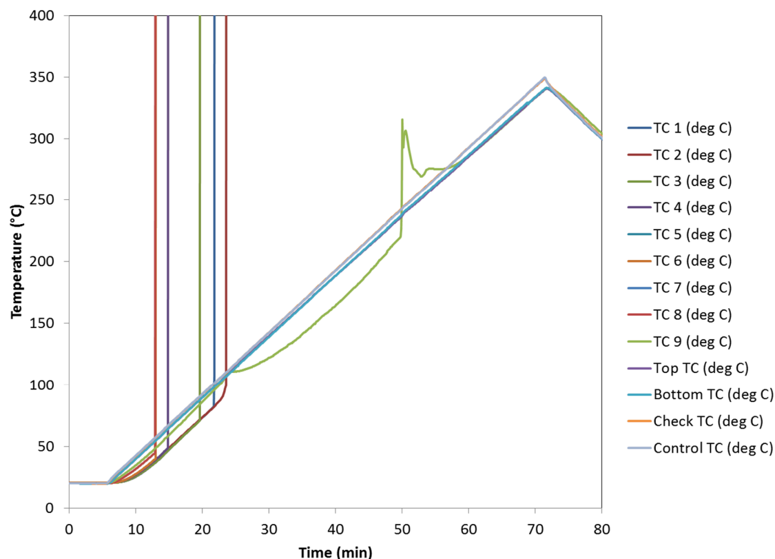
Figure 30. Exp398 temperature data. Contents were over-neutralized acid, Swheat, and the LANL SA mix.
