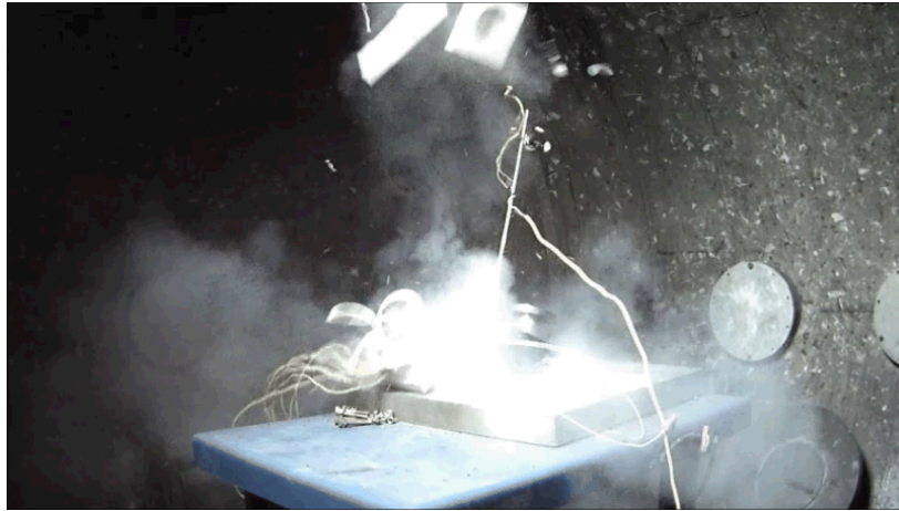
Figure 51. Image from video of Exp406 at ignition.
