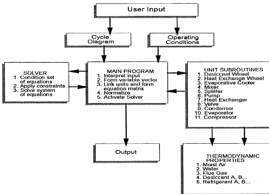
Fig. 4. Outline of desiccant cycle model.
