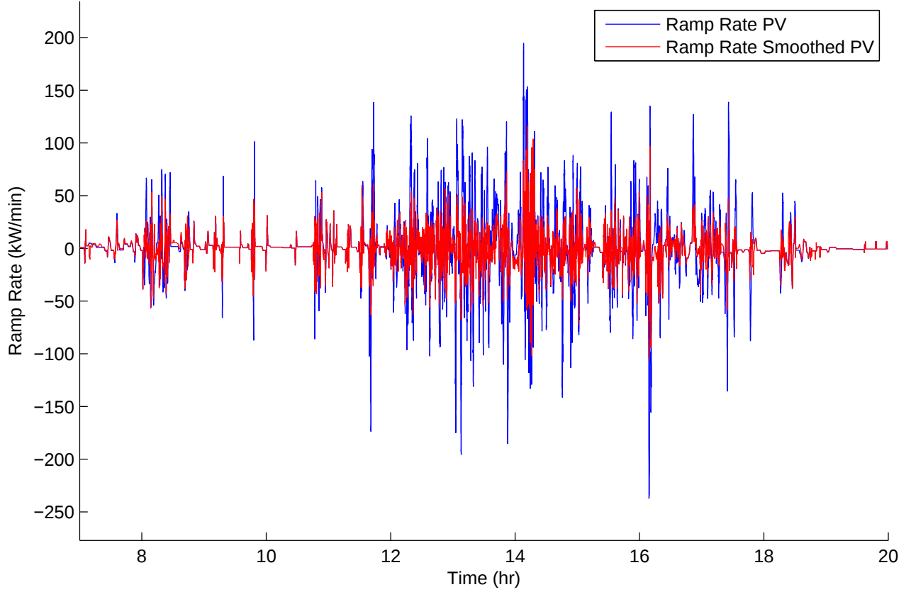
Figure 14: Residue R(n)
