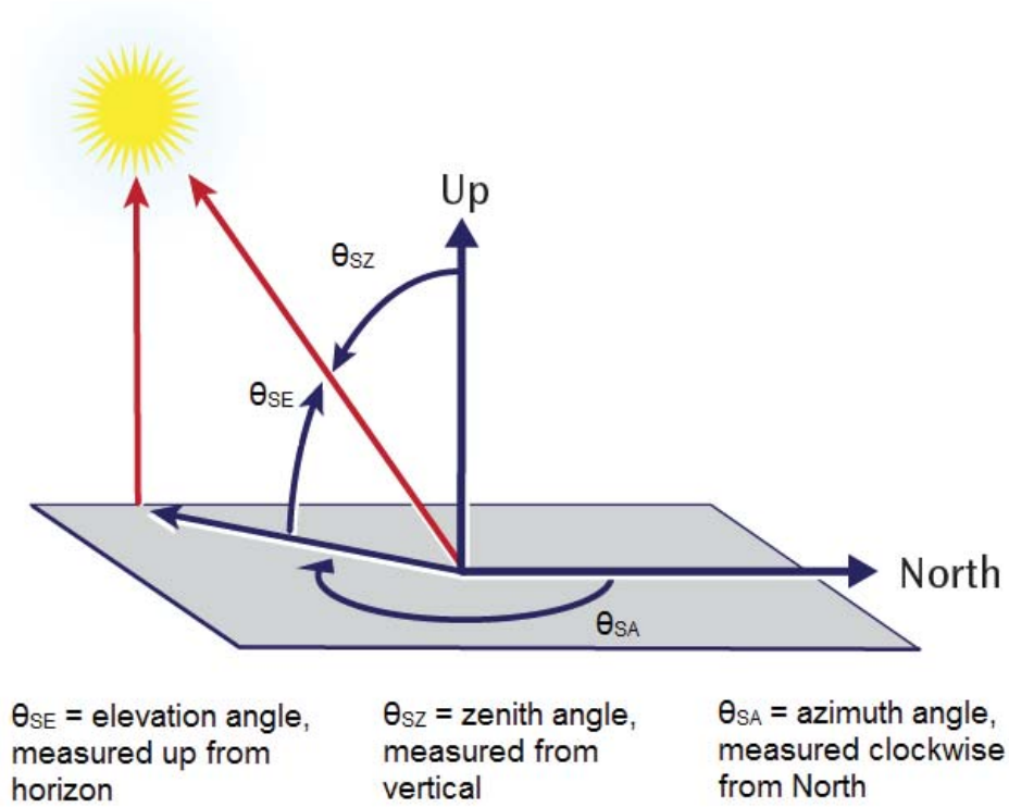
Figure 1: Description of solar position angles from an observer on Earth's surface
