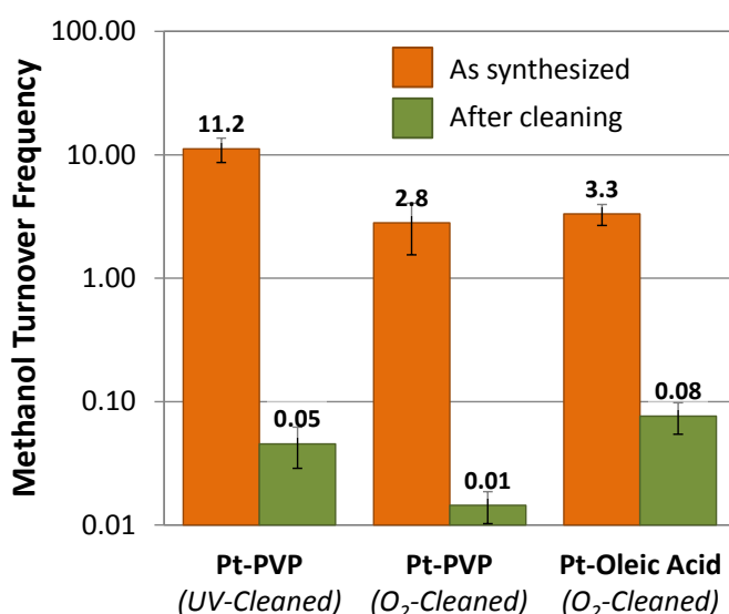
Fig. 6 Methanol oxidation turnover frequency (TOF) for Pt nanoparticle catalysts before and after cap removal. TOF is given as the number of methanol molecules converted per Pt site per s. The number of platinum sites was determined from the measured rate of ethylene hydrogenation using a known TOF. Consequently, each bar shows the methanol oxidation rate relative to the ethylene hydrogenation rate on the same catalyst. Data is shown for all three types of nanoparticles studied (i.e., UV-cleaned Pt–PVP, thermally-cleaned Pt–PVP, and thermally-cleaned Pt–OA). Noting that this graph is on a log-scale, the Pt activity for methanol oxidation is shown to decrease for each catalyst by a factor of between 50 and 250 following cap removal.
