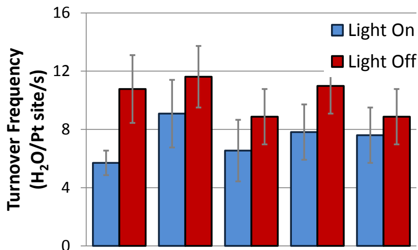
Fig. 1 Turnover frequency of hydrogen oxidation in 10 Torr \text{H}_2 , 30 Torr \text{O}_2 and 740 Torr He at 423 K. Turnover is calculated based on the rate of decrease of the hydrogen peak height in the chromatogram. In between each on/off cycle, the chamber was pumped down to 10^{-5} Torr. Error bars represent 95% confidence intervals.
