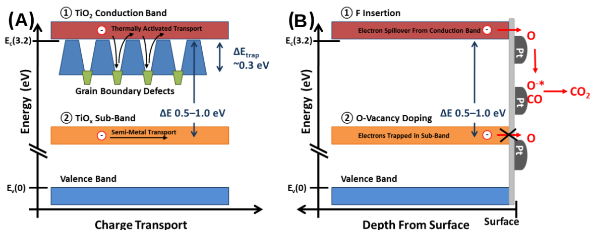
Fig. 3 (A) Band diagram depicting two types of transport in titanium oxide. Sub-band defect states in the reduced oxide provide a semi-metal transport channel. In stoichiometric TiO 2 , transport occurs in the actual conduction band. Due to grain boundary defects, conduction band transport is thermally activated as charges trap and de-trap at grain boundaries. (B) Schematic depicting why electronic activation is possible by F doping and not by O-vacancy doping. Although a high density of free charge carriers exist in the reduced oxide, these carriers reside in the sub-band located ~0.5–1.0 eV below the conduction band edge. At this low energy, the electrons cannot activate surface O for reaction with CO. However, in stoichiometric TiO 2 , electrons reside in the true conduction band. Charge transfer from the conduction band results in electronic activation of surface O for CO 2 formation.
