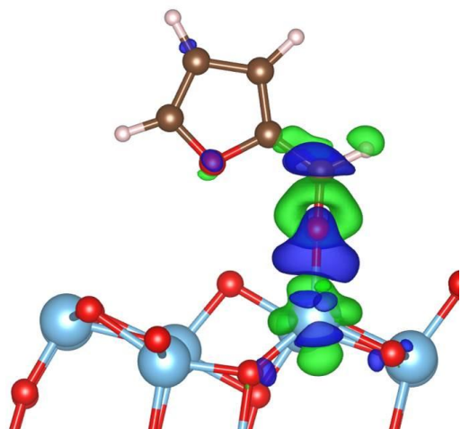
Fig. 8 The structure plot of a furfuraldehyde molecule binding to a Ti cation at an O-vacancy site on anatase \text{TiO}_2 , and the charge transfer induced by the surface binding interaction. The filled cyan, red, brown and white circles show the Ti, O, C and H atoms, respectively. The hollow green circles show the site of the O-vacancy (without the vacancy, there should be two O atoms inside the circle). The green contour shows the electron charge loss, and the blue contour shows the electron charge gain induced by the surface binding. In this charge transfer interaction, the Ti atom changes from a 3+ to a 4+ oxidation state, and the furfuraldehyde molecule acquires a negative charge. This negative charge localizes around the carbonyl C, activating it for H addition.
