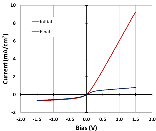
Fig. 4 Current-voltage curves of the device initially and after extended time in reaction conditions.
