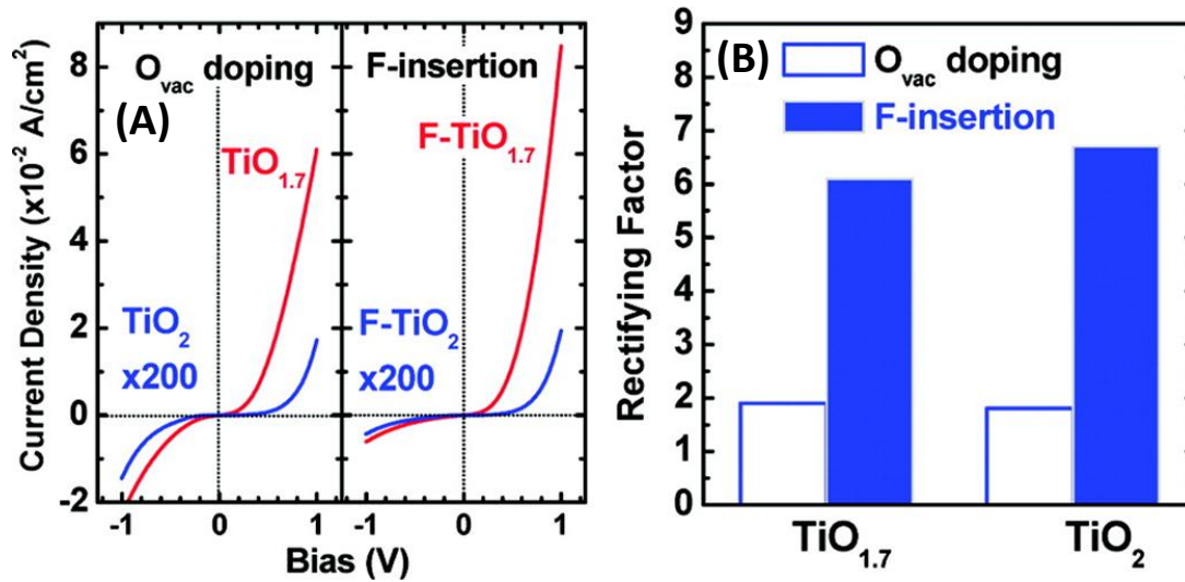
Fig. 5 (A) Current-voltage (IV) curves for \sim 10 nm \text{TiO}_x on highly doped ( 0.01 \Omega \text{ cm} ) p -Si. Red lines show \text{TiO}_{1.7} samples, and blue lines show \text{TiO}_2 . The current density values of all \text{TiO}_2 diodes were multiplied by a factor of 200. (B) Rectifying factor for \text{TiO}_2 and \text{TiO}_{1.7} before and after F doping. Rectifying factors are the ratio of forward to reverse bias current. For \text{O} vacancy doped \text{TiO}_x , low rectifying factors are the result of a high concentration of defect states and low Fermi level ( E_F ). By passivating defects and raising E_F , F doping increases the rectifying factor for each precondition by more than a factor of 3.
