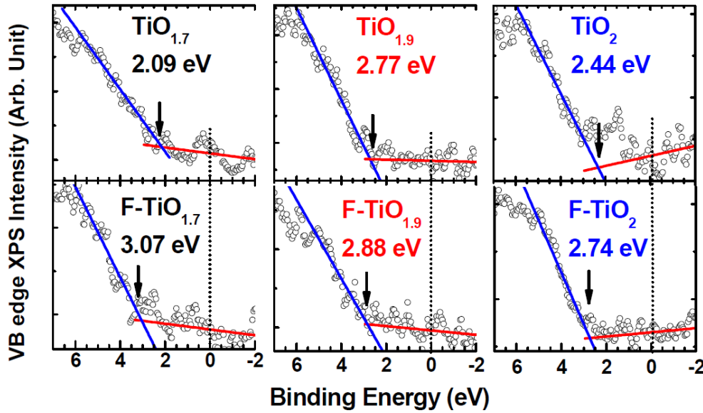
Fig. 7 VB edge XPS spectra for undoped and F-doped \text{TiO}_{1.7} , \text{TiO}_{1.9} , \text{TiO}_2 . Open circles show raw data, and lines show fitting used to determine Fermi level.
