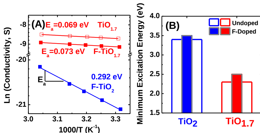
Fig. 2 (A) Arrhenius plots showing the activation energy for charge transport in TiO 1.7 and TiO 2 . Because TiO 2 without F is highly insulating, the Arrhenius curve could not be accurately measured for this sample. The different activation energies for conduction in TiO 1.7 and TiO 2 confirm different transport channels as depicted in Fig. 3A. (B) Minimum excitation energy having a fixed absorption coefficient of 2 \times 10^4 \text{ cm}^{-1} . This measurement reflects the decrease in bandgap energy for the reduced oxide and shows the difference in the energy of free electrons in the two supports.
