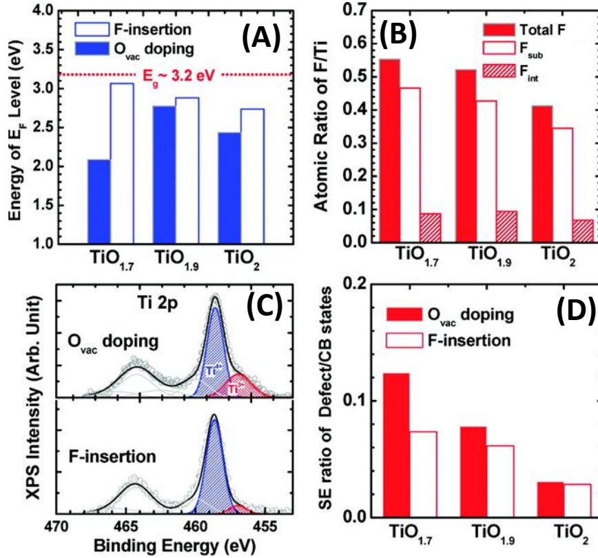
Fig. 6 (A) Fermi level ( E_F ) before and after F insertion for each \text{TiO}_x precondition determined by fits to the valance band edge XPS spectra (see Fig. 8). (B) The atomic ratio of F to Ti after 3 min. plasma treatment for each \text{TiO}_x precondition. Atomic ratios are shown for two different binding states identified by XPS (see Fig. 8B) and for total F. We assign these two binding states as F substituted for O and as interstitial F. Substitutional F concentration depends strongly on the initial O vacancy concentration before plasma treatment and appears to determine E_F after F insertion. (C) Ti 2p XPS spectrum of \text{TiO}_{1.7} before and after F insertion. Open circles show the raw data, and lines show the results of a Gaussian deconvolution. The peak state at 458.5 eV is the \text{Ti}^{4+} state in stoichiometric \text{TiO}_2 . The lower binding energy peak at 456.9 eV is the \text{Ti}^{3+} state and is a marker for O vacancy induced defect states. The decrease in \text{Ti}^{3+} state concentration with F insertion indicates that F passivates defects by binding to \text{Ti}^{3+} at O vacancies. (D) Ratio of defect state to CB absorption measured by spectroscopic ellipsometry before and after F insertion for \text{TiO}_{1.7} , \text{TiO}_{1.9} , and \text{TiO}_2 . Defect state/CB absorption was taken as the maximum absorption coefficient below/above 3.2 eV. The trend shows that F passivates O vacancies that give rise to defect states.
