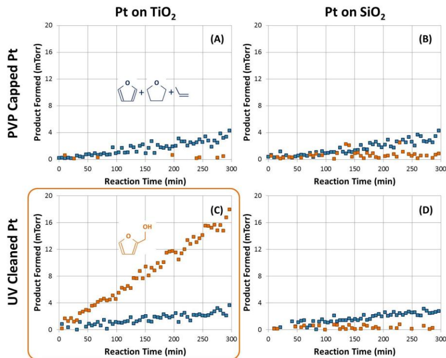
Fig. 2 Formation of reaction products as a function of time on four Pt nanoparticle catalysts. Parts (A) and (B) show results for PVP-capped Pt nanoparticles supported on TiO 2 and SiO 2 , respectively. Parts (C) and (D) show results for identical catalysts following 3 h UV cleaning to remove the PVP cap. Furfuryl alcohol is shown in orange, and decarbonylation products (i.e. furan, THF, and propylene) are shown in blue. The support has no effect on the activity or selectivity of the capped particles. However, following UV cleaning, the formation of furfuryl alcohol is selectively enhanced on the Pt/TiO 2 catalyst.
