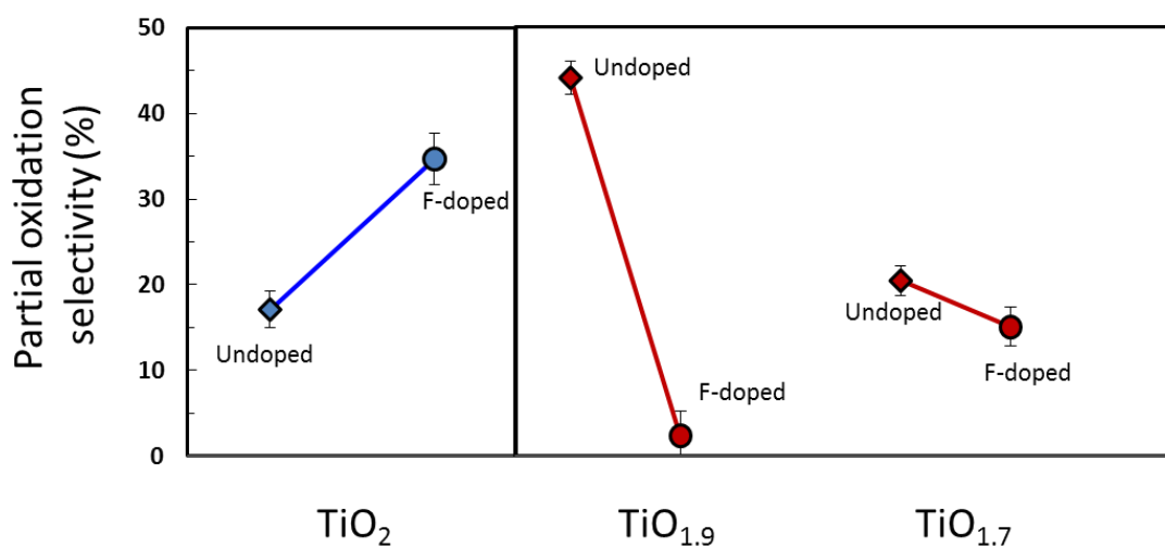
Fig. 3 Selectivity toward partial methanol oxidation of F-doped and undoped Pt/TiO x catalysts. Partial oxidation products refer to formaldehyde and methyl formate, as opposed to total oxidation that produces CO 2 .
