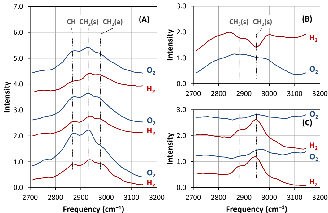
Fig. 1 SFG spectra of the PVP-capped Pt nanoparticles before UV cleaning (A) and after UV cleaning for 10 min (B and C). Spectra were obtained in 100 Torr of H 2 or O 2 in a background of Ar at 60 °C. A boxcar average over 5 data points improved signal-to-noise. In (A) and (C) the spectra are arbitrarily offset for clarity and were obtained sequentially from bottom to top. (B) shows the raw spectra with no offset of UV-cleaned nanoparticles first in H 2 then in O 2 . The spectrum obtained in H 2 shows a much higher nonresonant intensity with resonant features appearing as dips in the high background. This is a result of the phase mismatch between the resonant and nonresonant contributions of the spectrum. By subtracting the raw spectra from a baseline obtained in Ar, the negative features are inverted to appear positive for clarity (shown in C). Analysis of the resonant features in these spectra shows that before UV cleaning the PVP has a conformation that does not significantly change depending on the gas environment. However, following UV cleaning, carbonaceous fragments are found on the surface that are dynamic and reversibly restructure in H 2 and O 2 .
