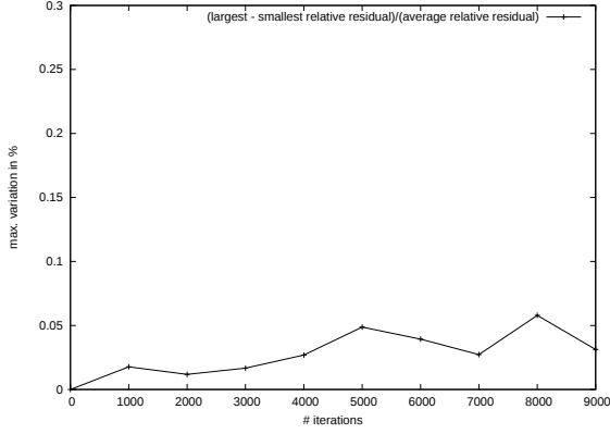
Figure 3: Statistic convergence behaviour of asynchronous iteration method.
