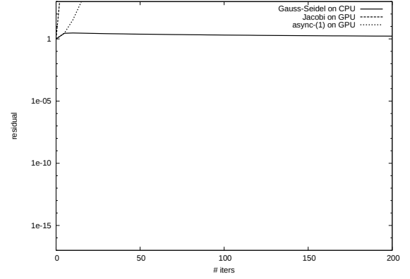
Figure 8: Convergence behavior of test matrix S1RMT3M1
