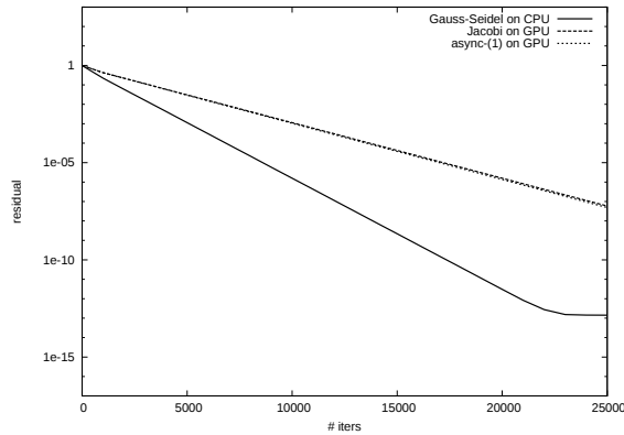
Figure 7: Convergence behavior of test matrix FV3
