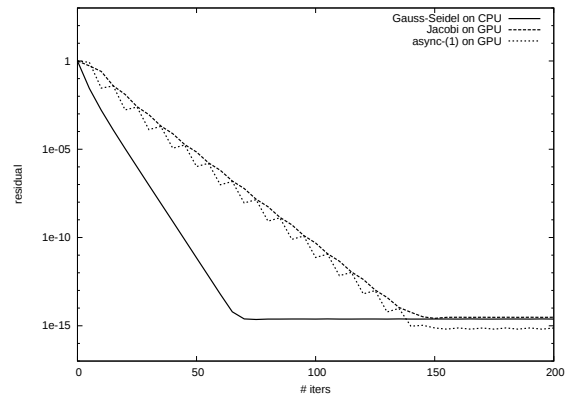
Figure 4: Convergence behavior of test matrix CHEM97ZTZ
