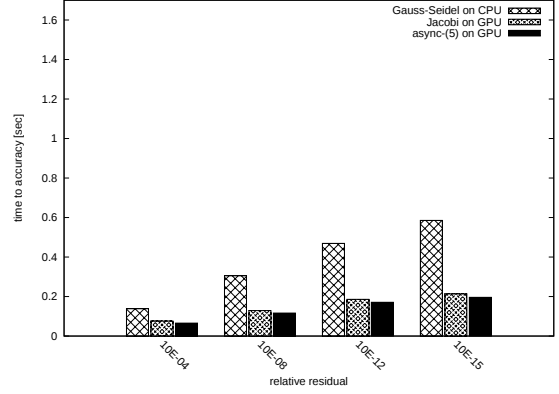
Figure 17: Time to solution for CHEM97ZtZ.
