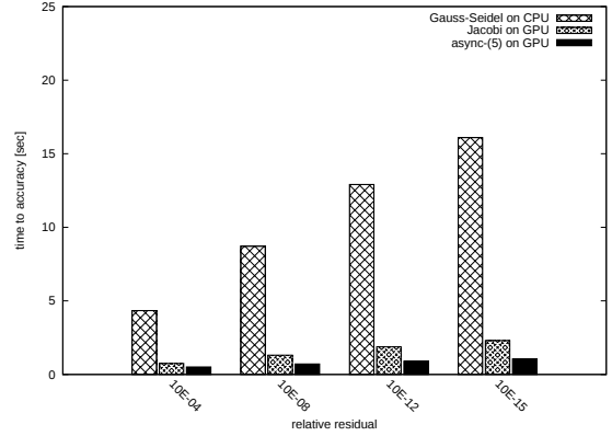
Figure 18: Time to solution for FV1.
