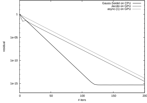
Figure 5: Convergence behavior of test matrix FV1
