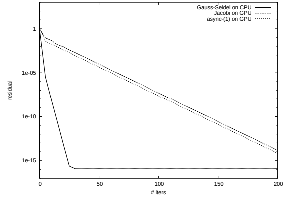
Figure 9: Convergence behavior of test matrix TREFETHEN_2000
