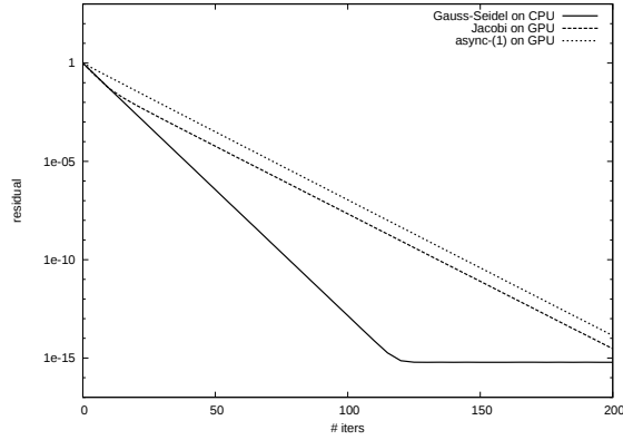
Figure 6: Convergence behaviour of test matrix FV2
