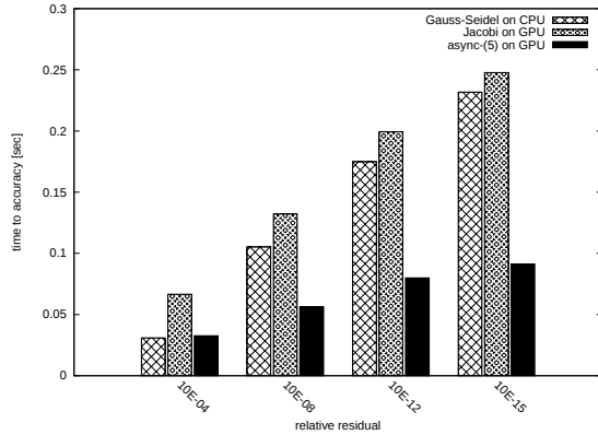
Figure 21: Time to solution for TREFETHEN_2000.
