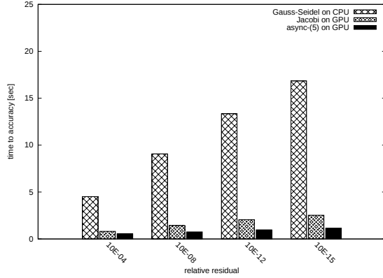
Figure 19: Time to solution for FV2.
