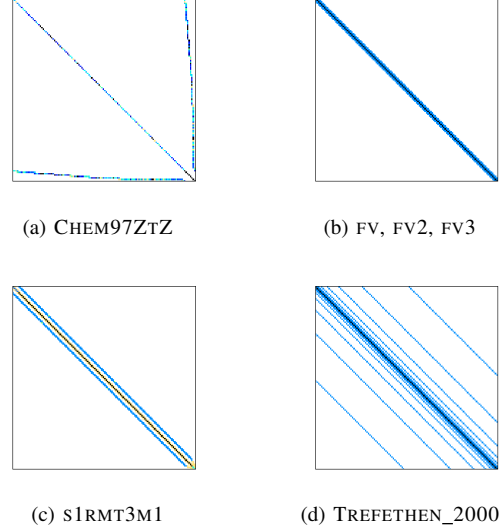
Figure 1: Sparsity plots of test matrices.
