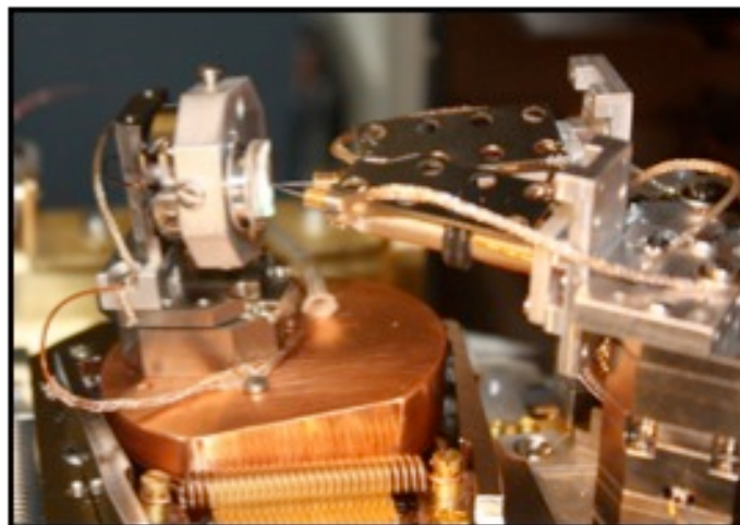
Figure 14. CINT's custom built nanomanipulator.
