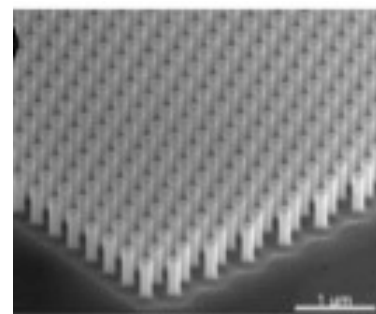
Figure 3. Nanowire arrays.
