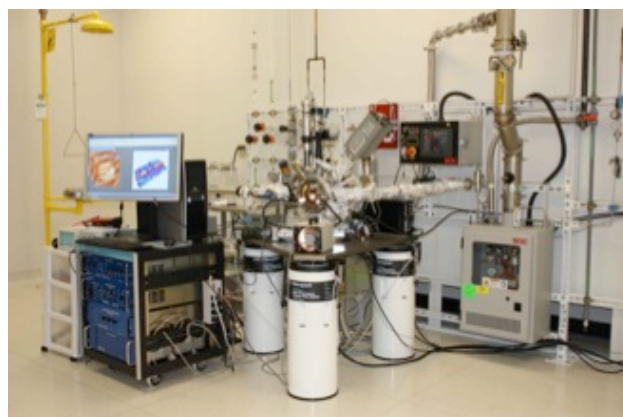
Figure 12. Atomic Precision Lithography
