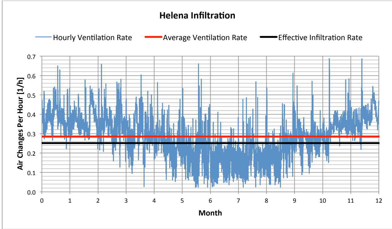
Figure 3: Hourly calculated infiltration rates for Helena, Montana. Note the higher variability in infiltration rates due to higher variability in weather conditions.
