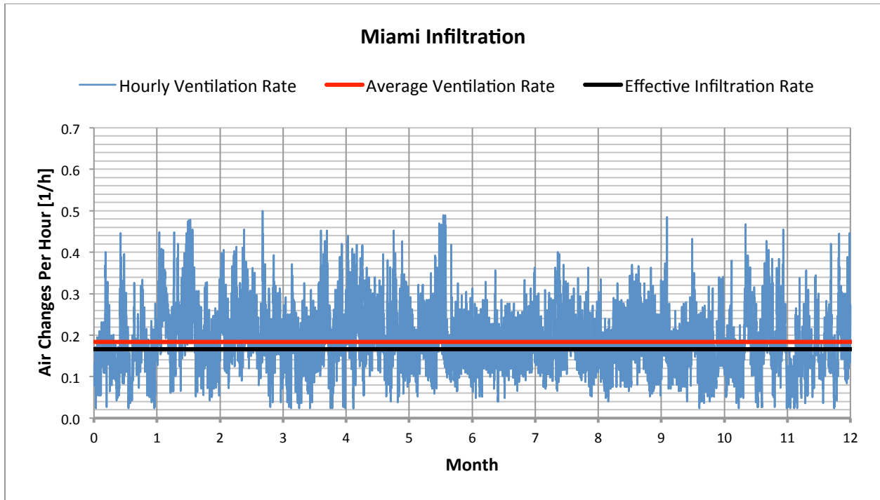
Figure 1: Hourly calculated infiltration rates for Miami, Florida with the average ACH and the effective ventilation calculated from the updated W -factor.
