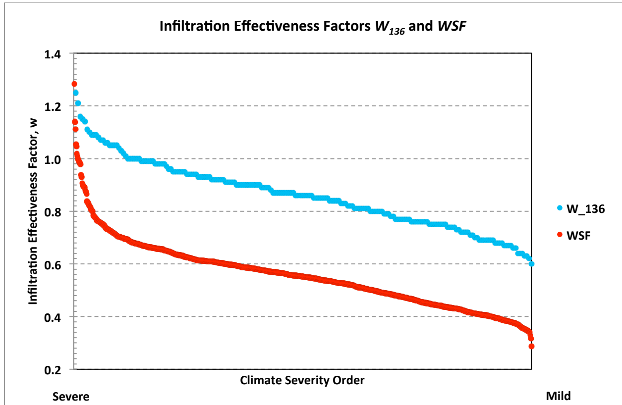
Figure 6: Current ( W_{136} ) and updated ( WSF ) values of W ranked by climate severity.
