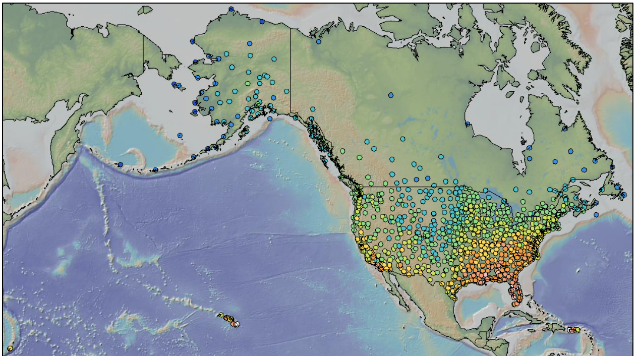
Figure 5: N_{62.2} factors for the United States, its territories and Canada. Maps from Ryan et al. (2009), data points plotted using GeoMapApp (Haxy, 2011).
