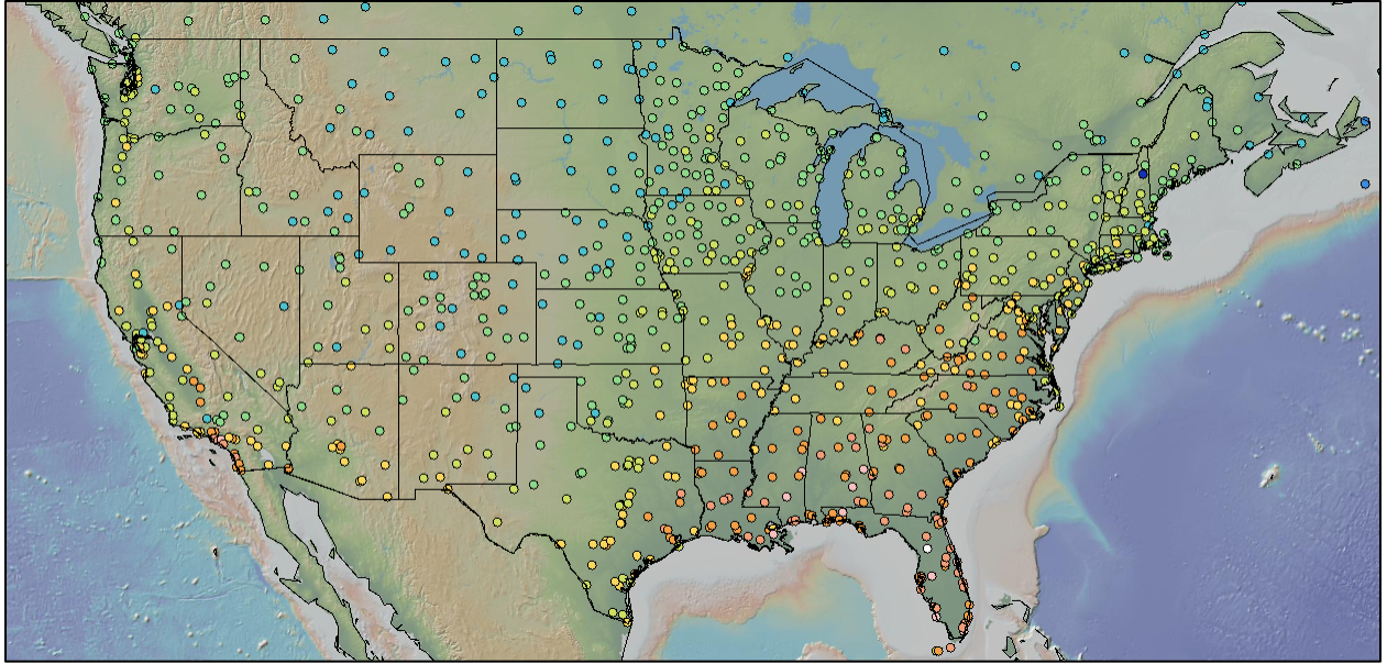
Figure 4: N_{62.2} factors for the continental United States.
