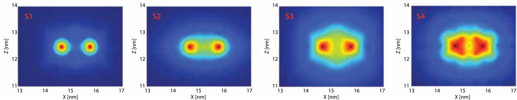
Atomistic tight-binding simulation of the four lowest electronic states of a P2+ donor molecule in Si (shown as 2D cuts).
