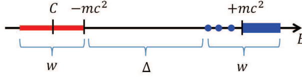
Figure 1: A sketch of the spectrum of the DKS operator. For explanations see the text.
