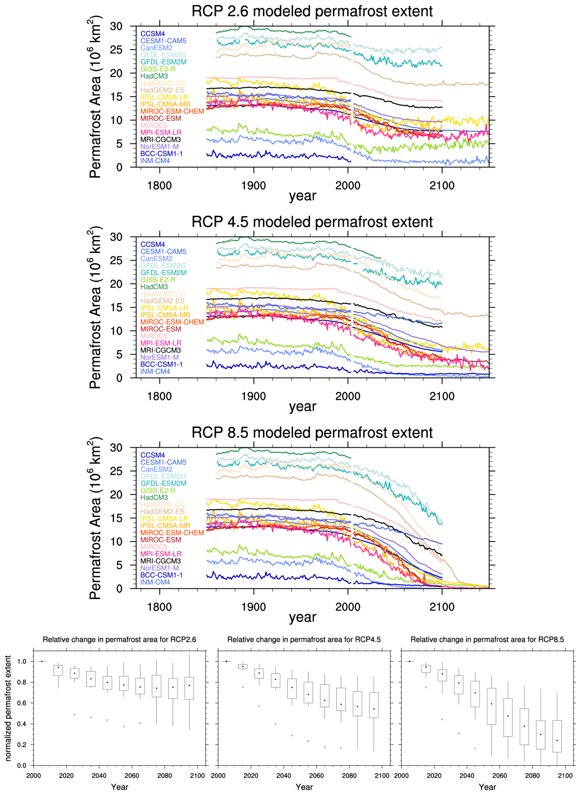
FIG. 11. Multi-model predictions of permafrost area under climate change scenarios: (a,d) RCP2.6, (b,e) RCP4.5, (c,f) RCP8.5. (a-c) Total permafrost extent for each model in CMIP5 analysis. A small gap is shown between historical experiment and RCP scenarios. (d-f) Box-whisker diagrams of fraction of permafrost at start of RCP scenarios remaining during 21st century.
