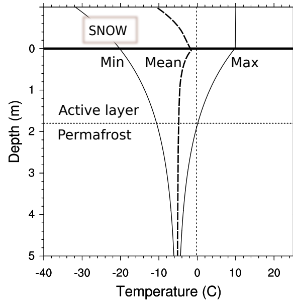
FIG. 1. Simplified schematic of permafrost thermal dynamics: Solid lines show vertical profiles of minimum and maximum annual temperatures across air-soil interface; dashed line shows mean annual temperature profile. Snow acts to insulate soils during winter, leading to steep gradient in wintertime and mean temperatures.
