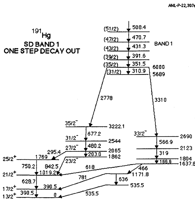
Figure 2. Partial level scheme, showing the one-step decay pathways connecting SD and ND levels.
