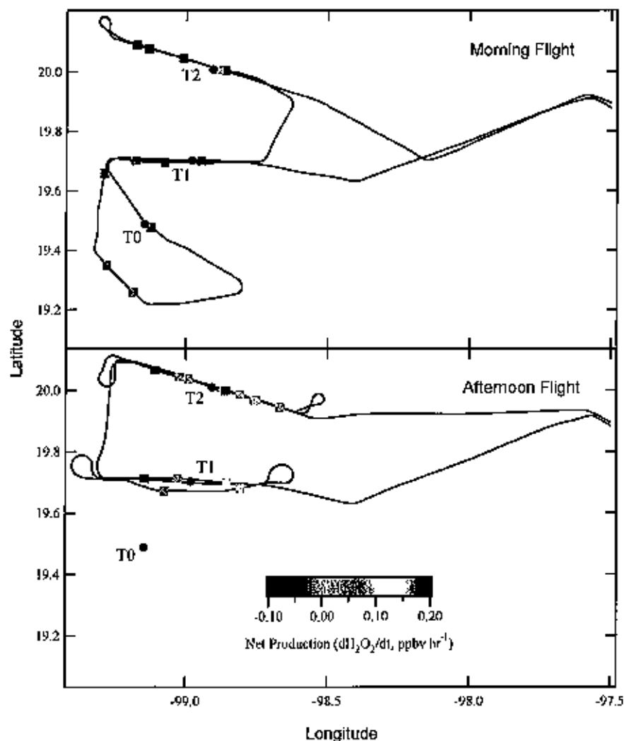
Fig. 16. Morning and afternoon net (i.e. production – loss) production rate of hydrogen peroxide ( \text{ppbv hr}^{-1} ) on 20 March 2006 with each square indicating a hydrocarbon sampling location. Black circles indicate the location of surface sites T0, T1 and T2.
