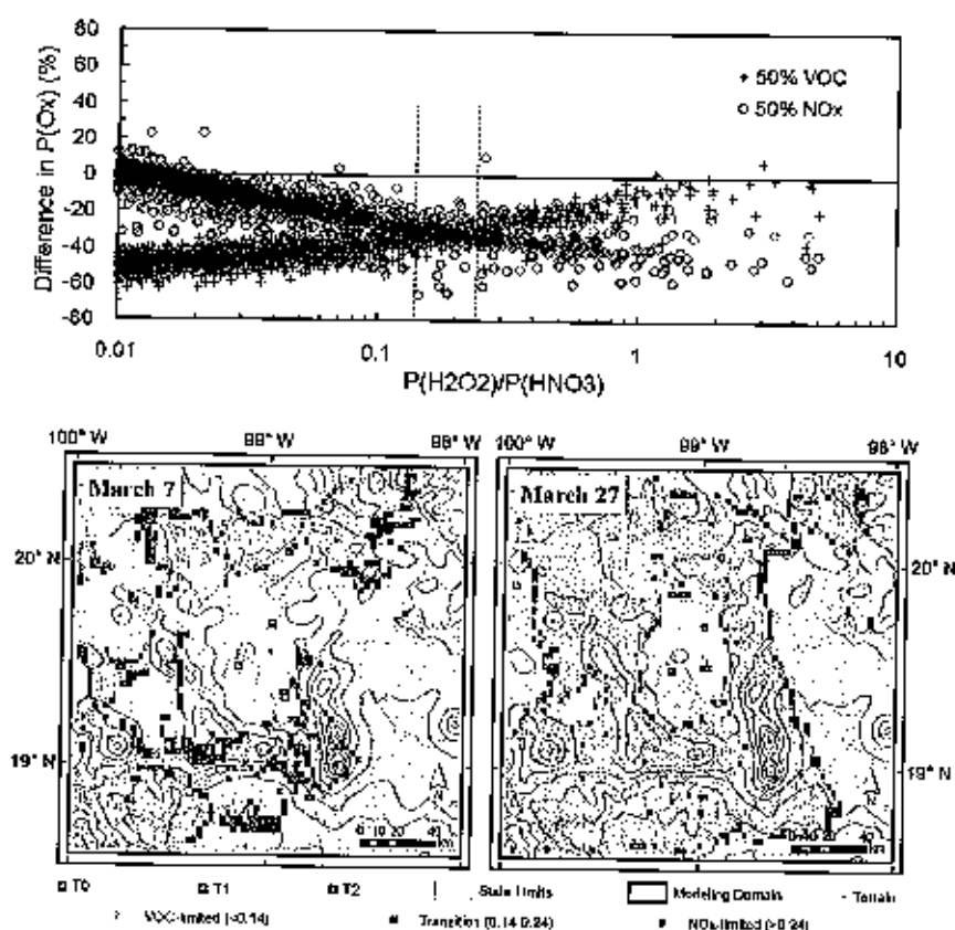
Fig. 11. Top panel: The percentage change in O_3 formation rate as a function of the indicator, ratio of H_2O_2 production rate to HNO_3 production rate at 12:00–17:00 LT during the episodes (weekends are shown in gray) within the urban area. The dashed bars envelop the transition regime. Bottom panel: Spatial distribution of the ratio at 14:00 LT on 7 and 27 March 2006 indicating the NO_x -VOC sensitivity (source: Song et al., 2010).
