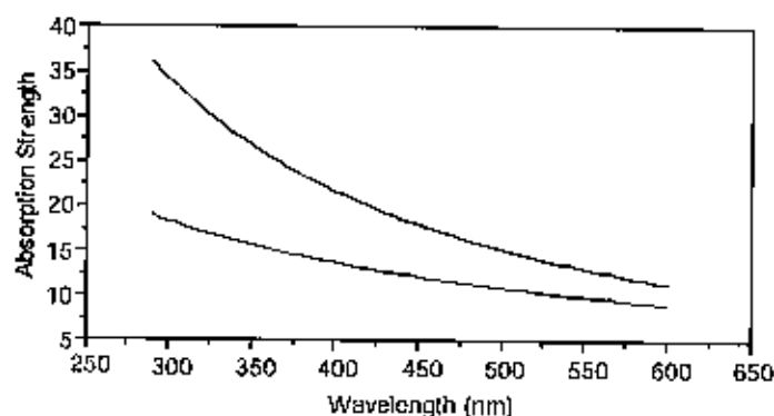
Figure 6. Absorption strengths ( \text{m}^2/\text{g} ) for a soot type BC aerosol (green) and a biomass type BC aerosol (blue).
