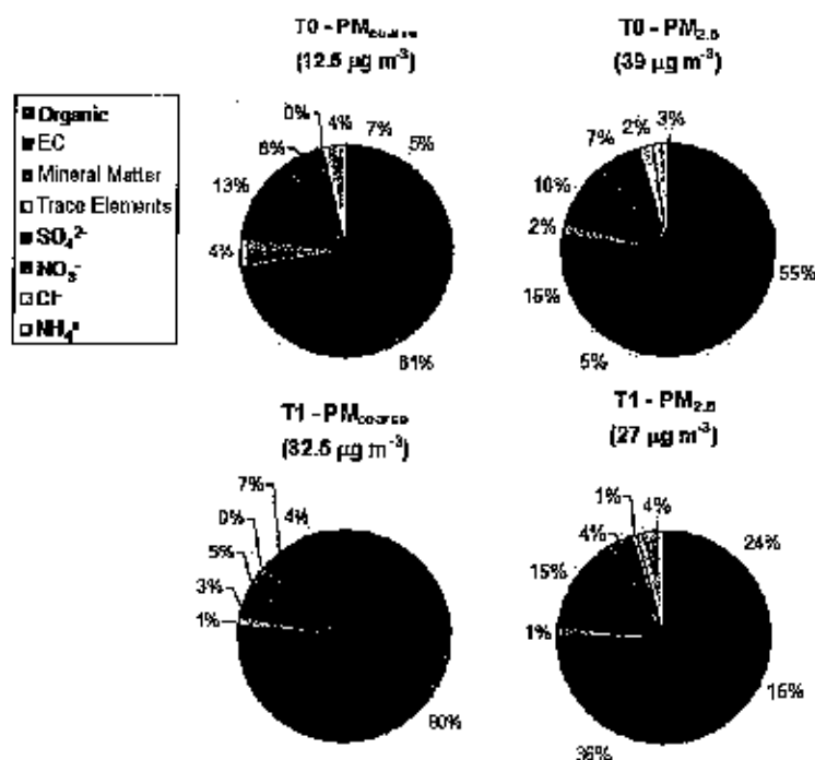
Fig. 12. Average composition of \text{PM}_{\text{coarse}}(\text{PM}_{10}-\text{PM}_{2.5}) and \text{PM}_{2.5} at the T0 and T1 supersites, based on the results of Querol et al. (2008). OA was calculated from the measured OC based on the average measured OA/OC ratio of 1.75 at T0 (Aiken et al., 2008). The T1 site was affected by local resuspension of dust, which explains the unusually large contribution of mineral matter at this site.
