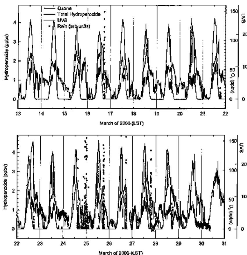
Fig. 8. Time series of total hydroperoxide (in black) for the period 13–30 March 2006 at Tecamac University. See text for peroxide species measured. Also shown are solar radiation (gray), ozone (red) and periods of measurable rainfall (blue) at this site.
