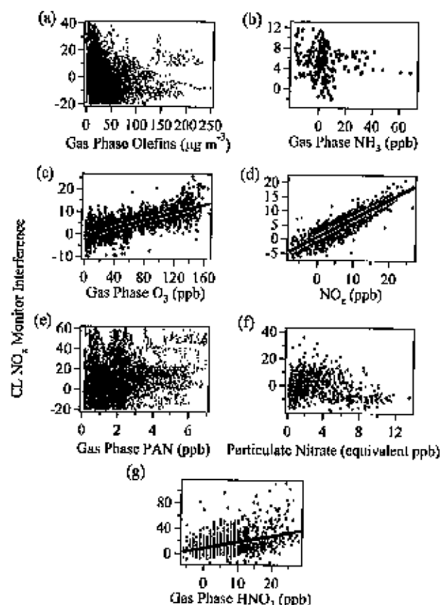
Fig. 2. Linear regression plots for the CL NO x monitor interference plotted versus (a) gas phase olefins (CENICA), (b) gas phase NH 3 (Santa Ana), (c) gas phase O 3 (Pedregal), (d) NO x (Pedregal), (e) gas phase PAN (CENICA), (f) particulate nitrate (La Merced), and (g) gas phase HNO 3 (La Merced). See text for description of measurements. Results of the linear regressions are listed in Table 1.
