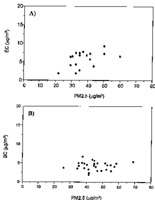
Fig. 4. (A) Elemental carbon content of \text{PM}_{2.5} particulate samples collected during the IMADA-AVER study, 1997 (Edgerton et al., 1999) and (B) black carbon and \text{PM}_{2.5} aerosol concentrations measured during the Mexico Megacity 2003 study.
