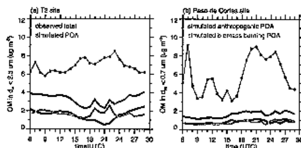
Fig. 13. Time series of observed and modeled average diurnal variations of organic matter at the (a) T2 site using Sunset Laboratory BC/OC data and the (b) Paso de Cortes site using Aerodyne Aerosol Mass Spectrometer (AMS) data. PMF components not currently available at the Paso de Cortes site.
