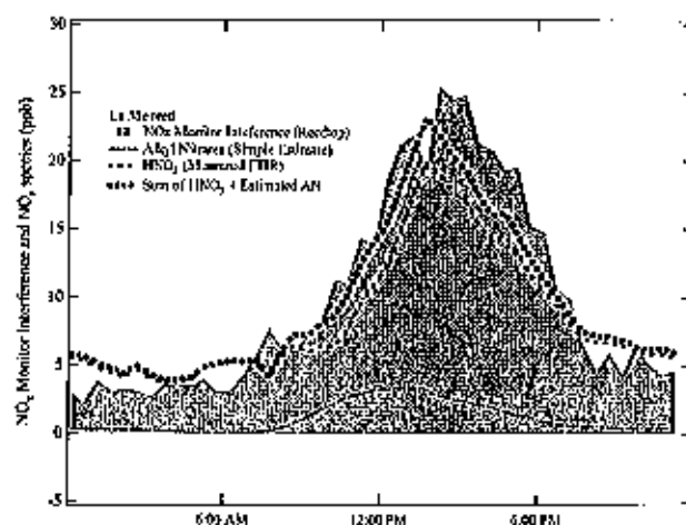
Fig. 4. Diurnally averaged profiles for measured CL \text{NO}_x monitor interference, measured \text{HNO}_3 concentrations and calculated alkyl nitrate concentrations at La Merced site. Profiles averaged over the entire MCMA-2003 campaign. Also included is a profile of the sum of the measured \text{HNO}_3 concentration plus the estimated alkyl nitrate concentration (see text). Time of day is for local time.
