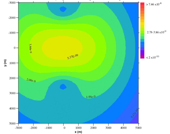
Figure 6: Surface anomalous horizontal magnetic field ( B_h ) for 2.5 kt \text{CO}_2 with 360 amp-m, 1 Hz downhole source.
