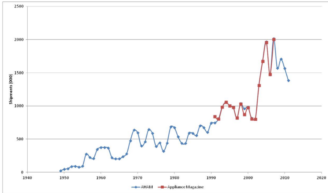
Figure 3-2 Dehumidifier Shipments, 1949–2011
