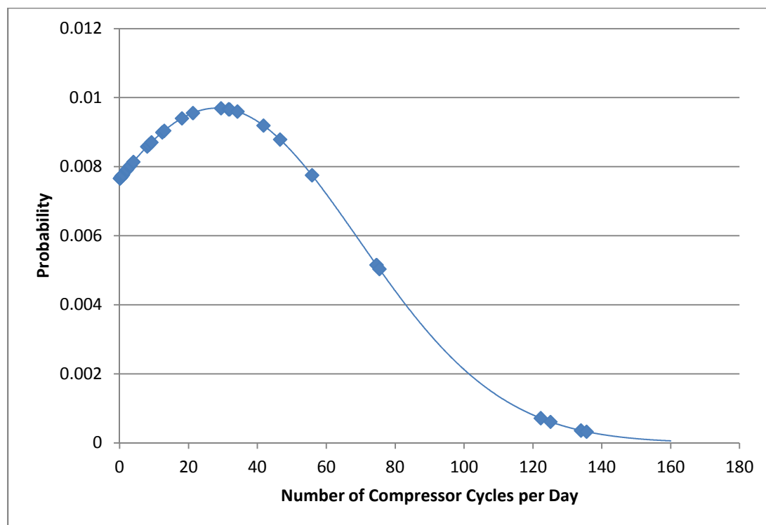
Figure 6-6 Distribution of Compressor Cycles per Day for Selected Dehumidifier Units
