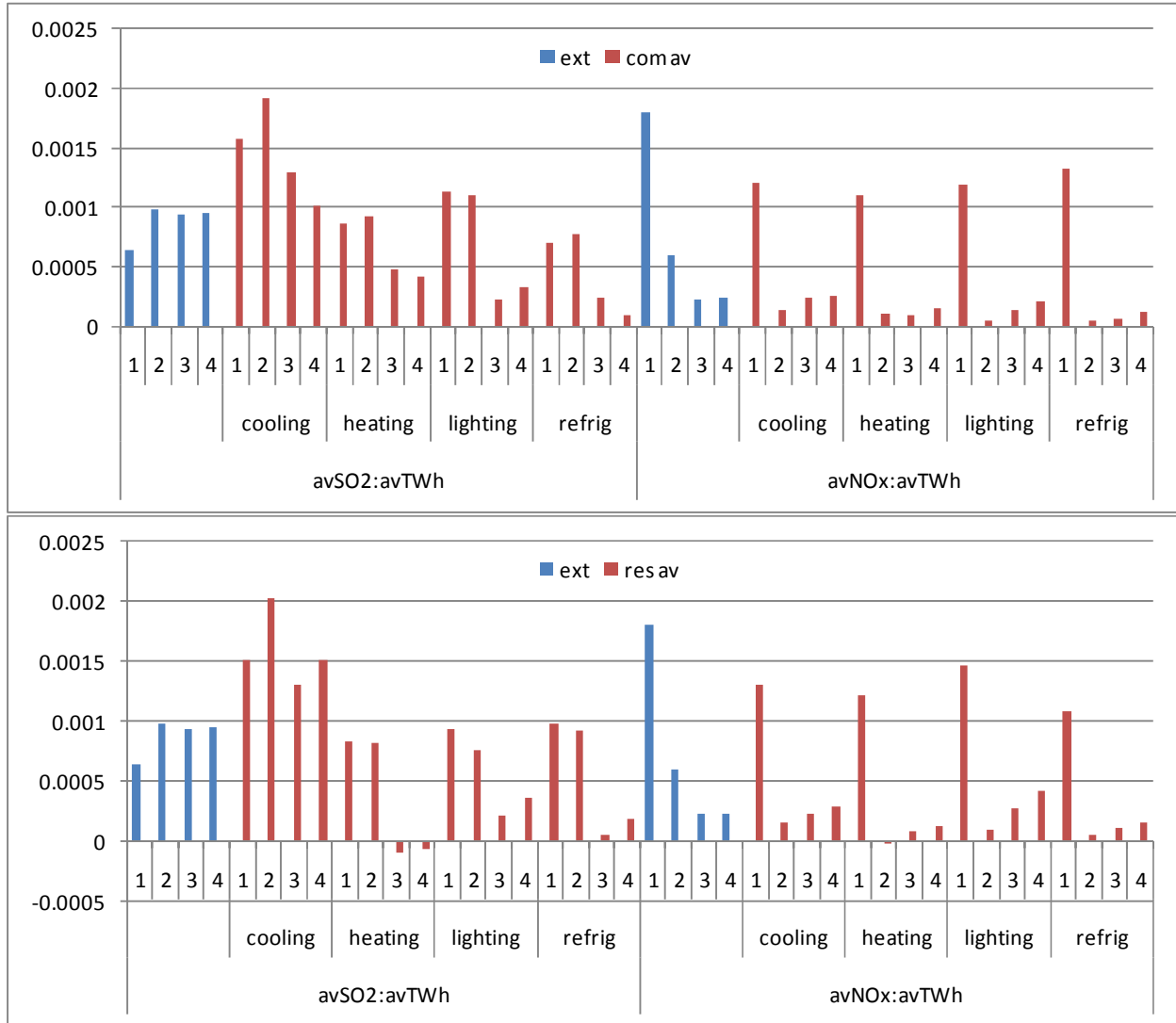
Figure 9 Response Coefficients for \text{SO}_2 and \text{NO}_x Emissions
