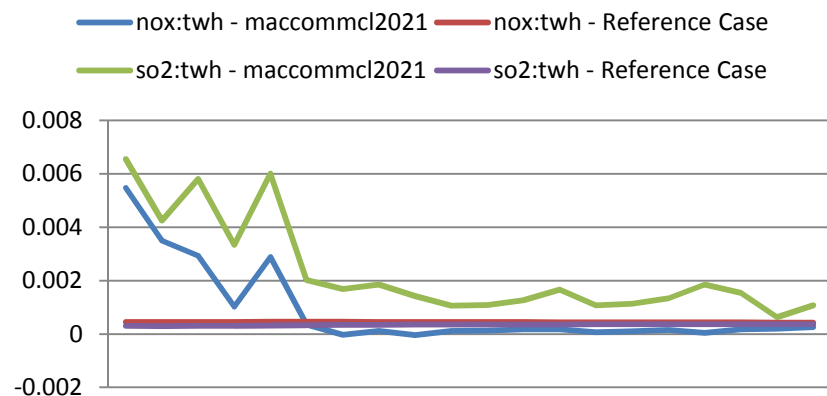
NO x and SO 2 Emissions Starting Year 2021
