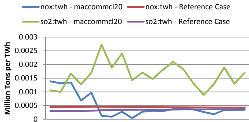
NO x and SO 2 Emissions Starting Year 2016
