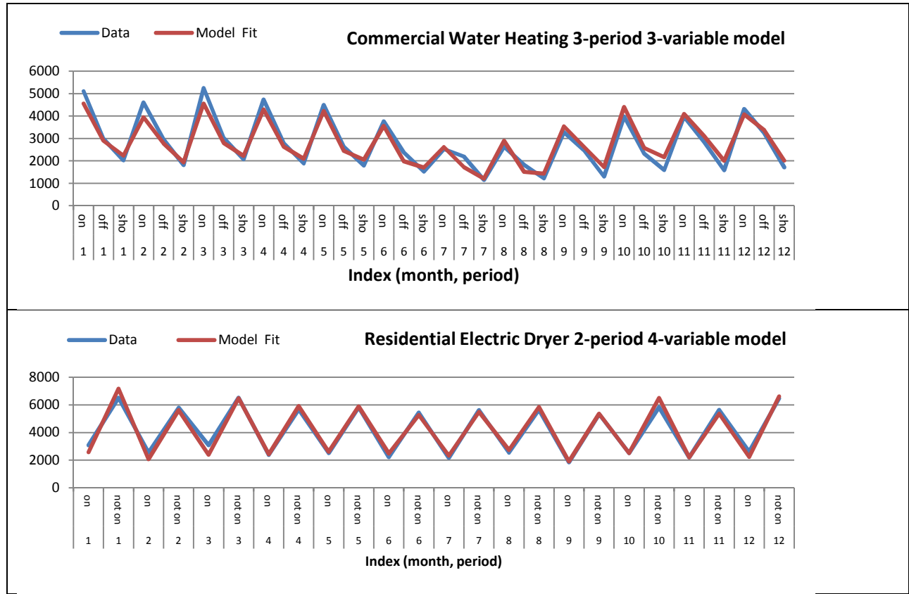
Figure 12 Comparison of original load shape data and model fits.
