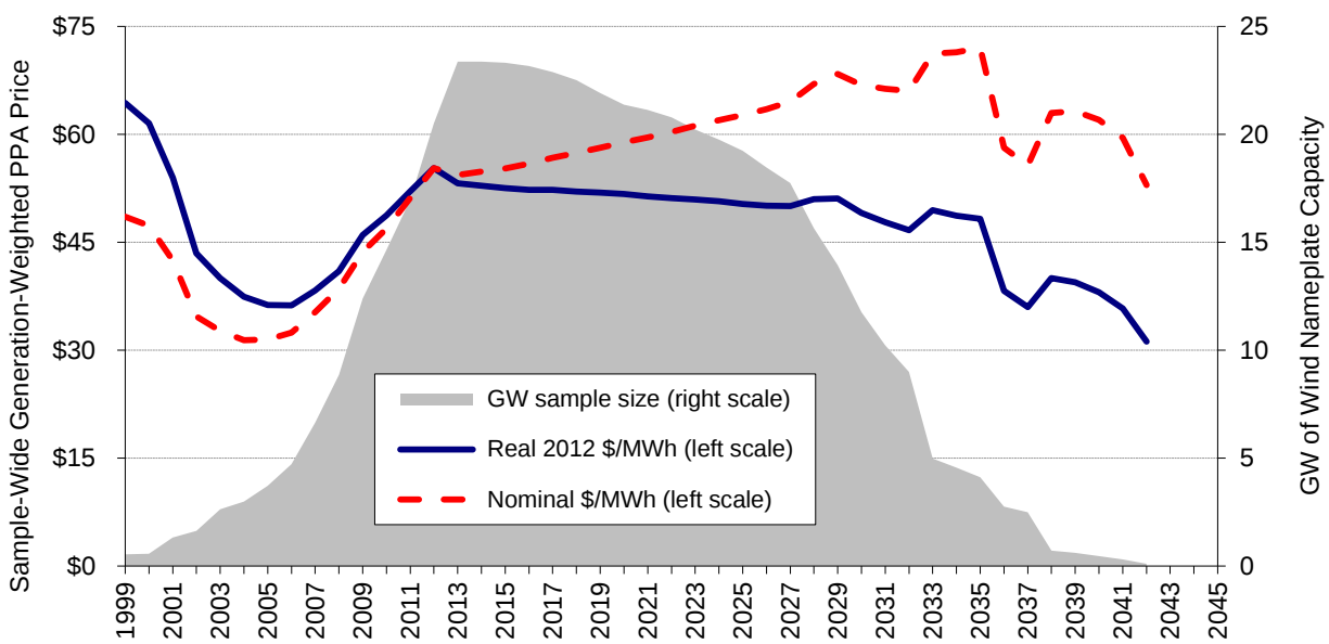
Figure 3. Generation-Weighted Average Wind PPA Price Over Time vs. Sample Size
