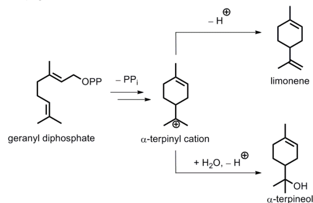
Scheme 1. Biosynthesis of limonene and \alpha -terpineol from geranyl diphosphate (PP i = diphosphate). While limonene is obtained through a deprotonation route, capture of the \alpha -terpinyl cation with water affords \alpha -terpineol. 4, 5-7
