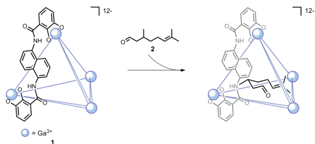
Scheme 2. Encapsulation of 2 by host 1; spheres represent a Ga 3+ center and bisbidentate ligands are depicted as lines.
