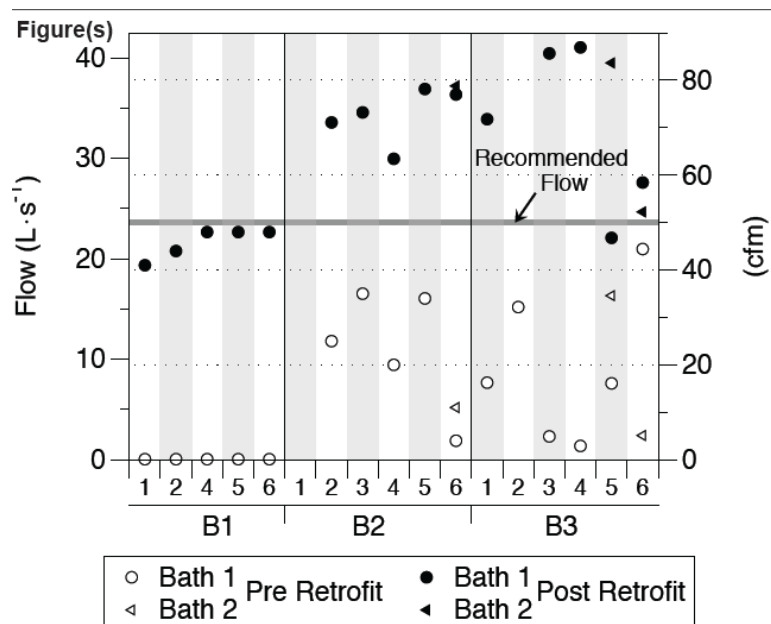
Figure 2. Bathroom exhaust fan airflows measured before and after the retrofit implementation.
