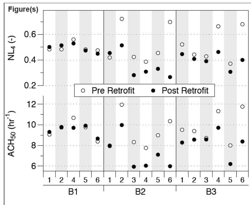
Figure 1. Air changes per hour at 50 Pa (ACH50) and normalized leakage at 4 Pa (NL4) measured before and after retrofits. No work was done to improve envelope airtightness in B1 and B2A1.
