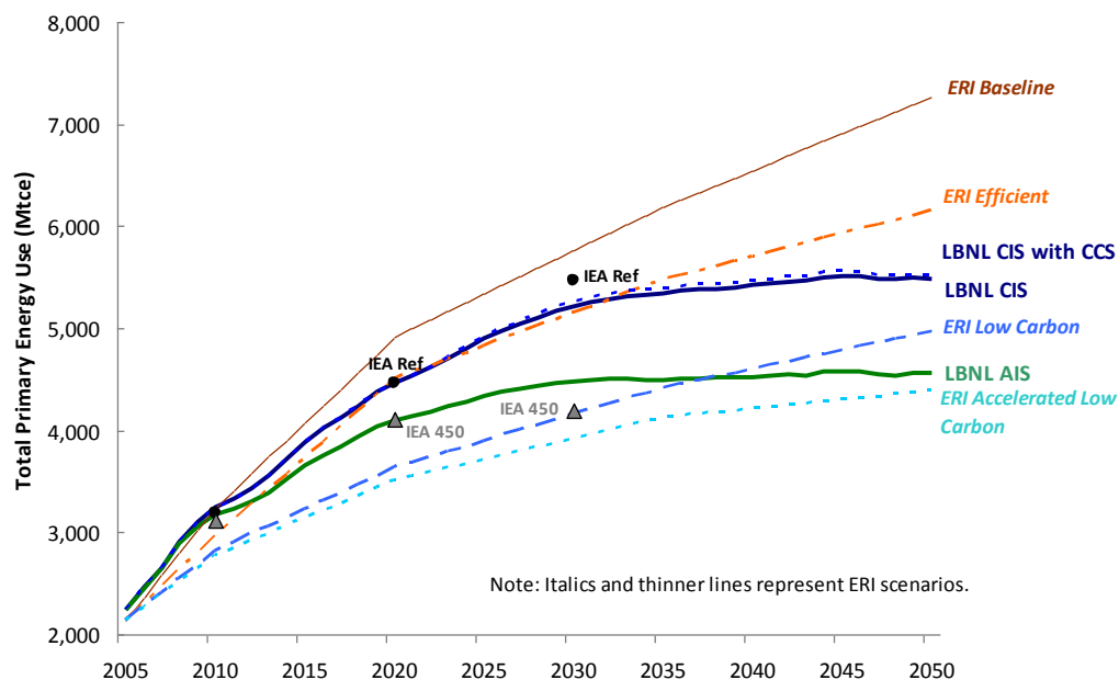
Figure 1. Primary energy consumption in different scenarios
