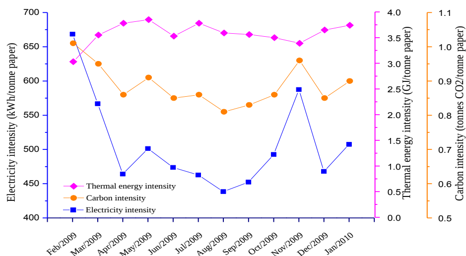
Figure 4. Energy and CO 2 intensity of the PM4
