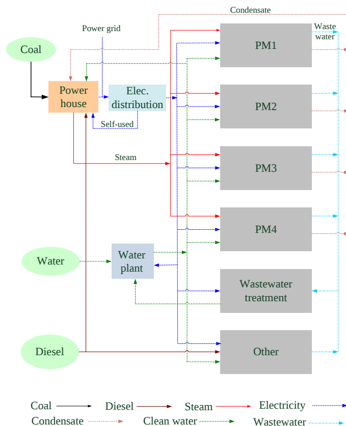
Figure 2. Energy flow at the paper mill
