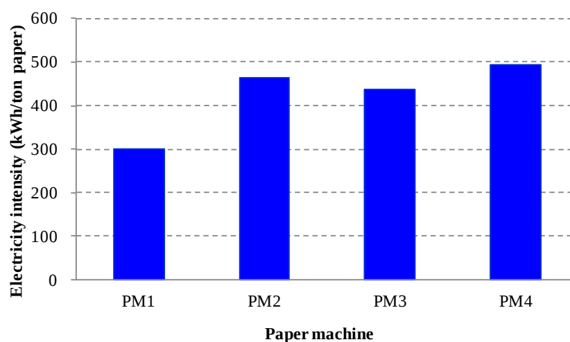
Figure 5. Electricity intensity of the paper machines during the audit period
