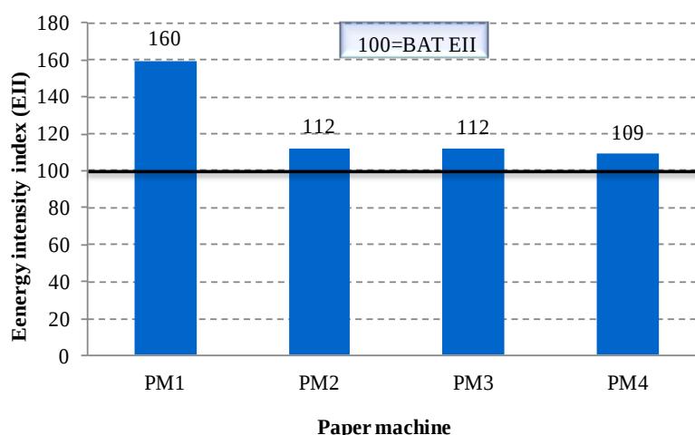
Figure 8. Energy intensity index (EII) of the paper machines
