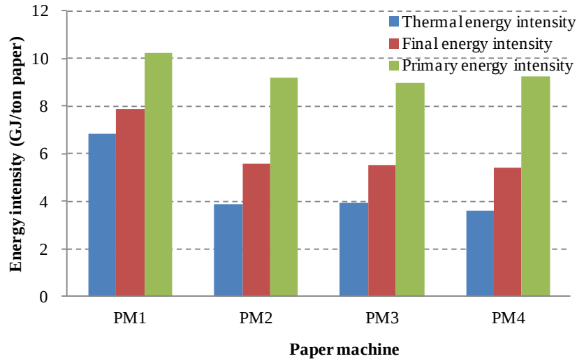
Figure 6. Energy intensity of the paper machines during the audit period
