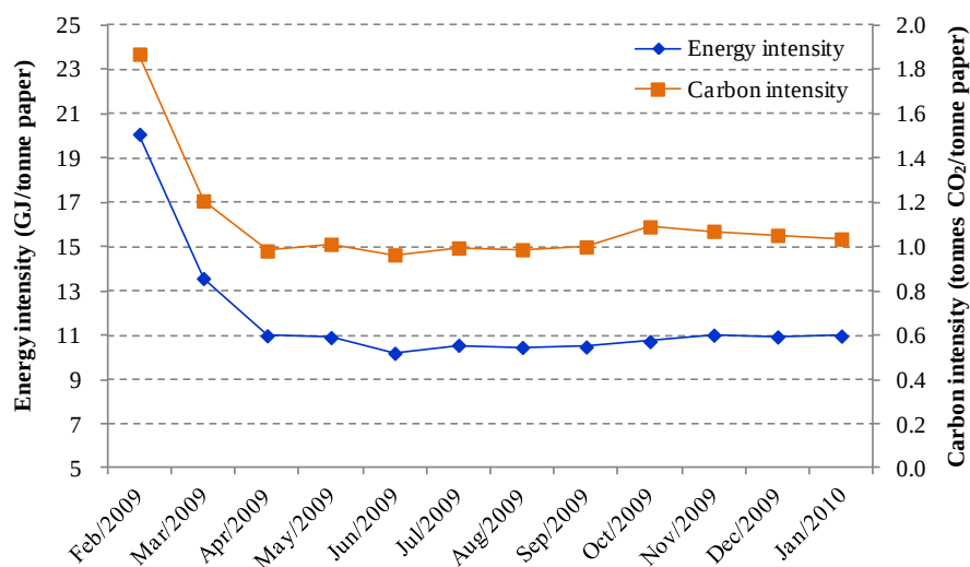
Figure 3. Primary energy and CO 2 intensity of the audited paper mill
