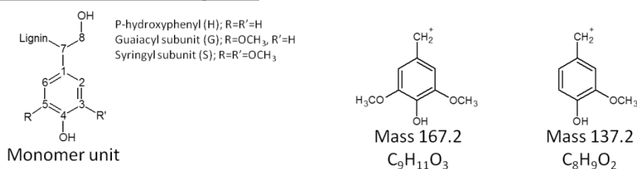
Figure 2. Proposed structures for lignin molecules observed in the lightest fraction ( 1.6 \text{ g cm}^{-3} ) of Susua soil.
