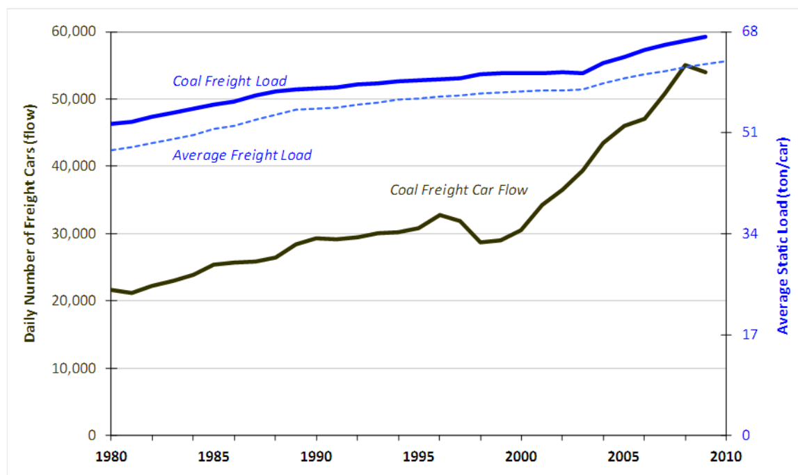
Figure 34. China Railway Daily Freight Flow and Average Loads, 1980 to 2010
