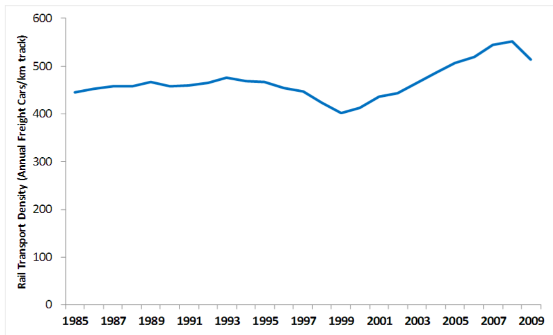
Figure 33. China Rail Freight Transport Density, 1985 to 2009
