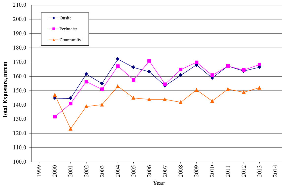
FIGURE 4-2. Tonopah Test Range TLD Exposure, 2000-2013
