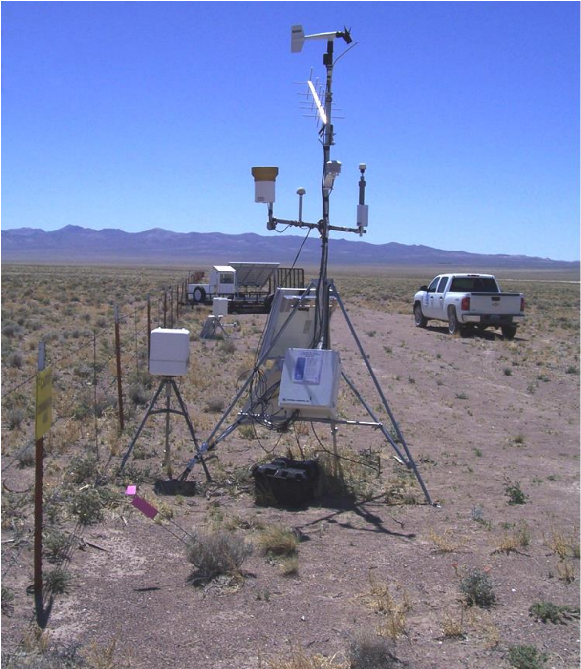
FIGURE 1-4. The solar powered air sampler, saltation sensor, and meteorological tower (background, center, and foreground, respectively) at Station 401 are located along the north fence that bounds the Clean Slate 3 contamination area.
