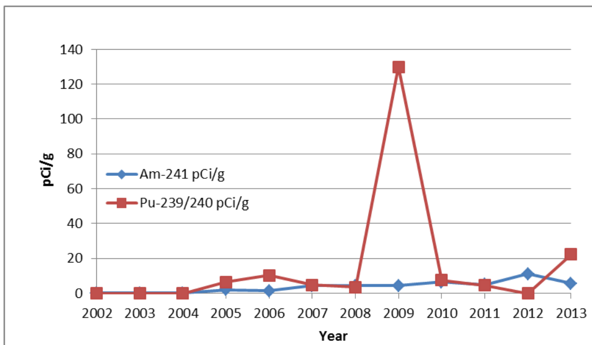
FIGURE 4-1. Historical Plutonium-239 and Americium-241 at TTR S-51
