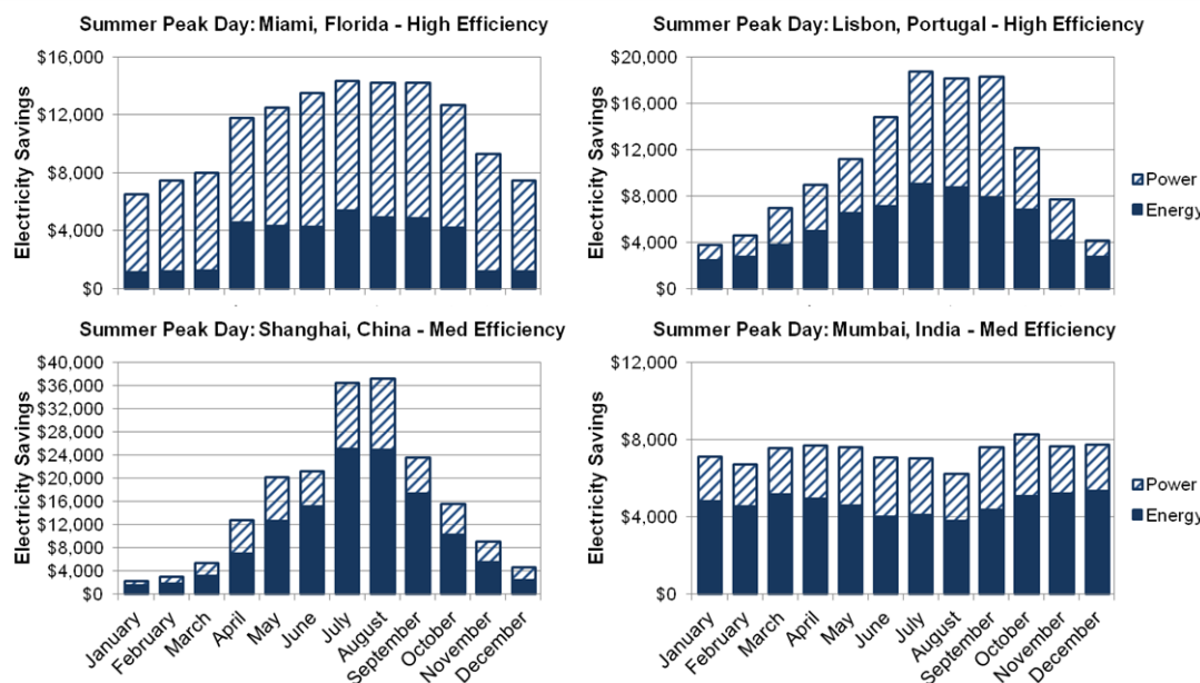
Figure 5. Monthly electricity cost savings. Savings from monthly electricity are broken down between energy and power charges. Shape and magnitude of savings depend on local tariff structure.
