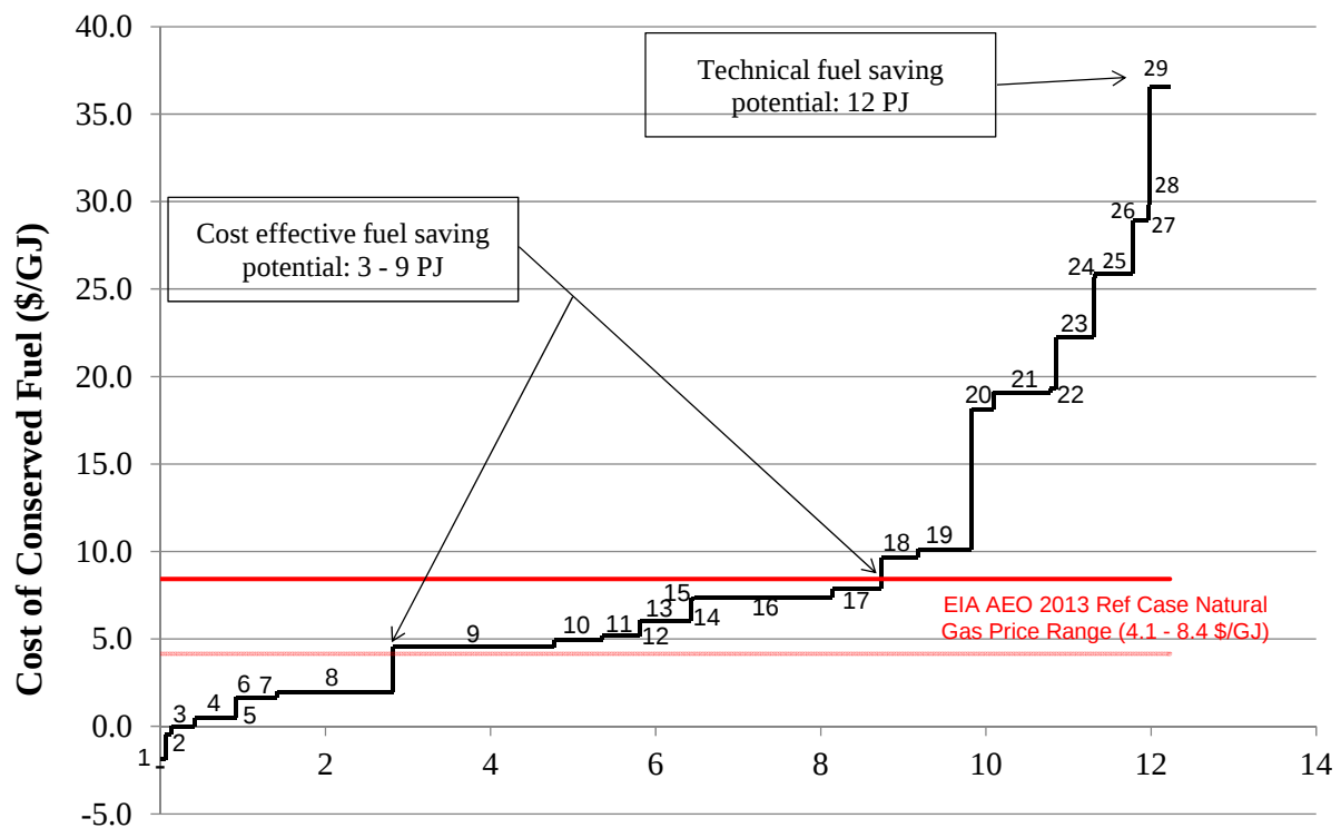
Figure 23 – ISU Cost-of-Conserved Combined Fuel and Associated Electricity Supply Curve
