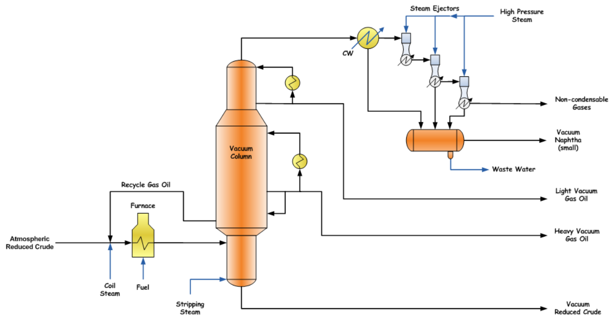
Figure 5 – Deslater & Atmospheric Crude Unite Process Flow Diagram
