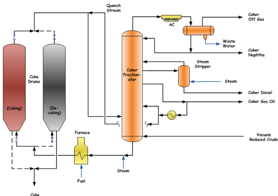
Figure 8 – Delayed Coking Unite (CKU) Process Flow Diagram
