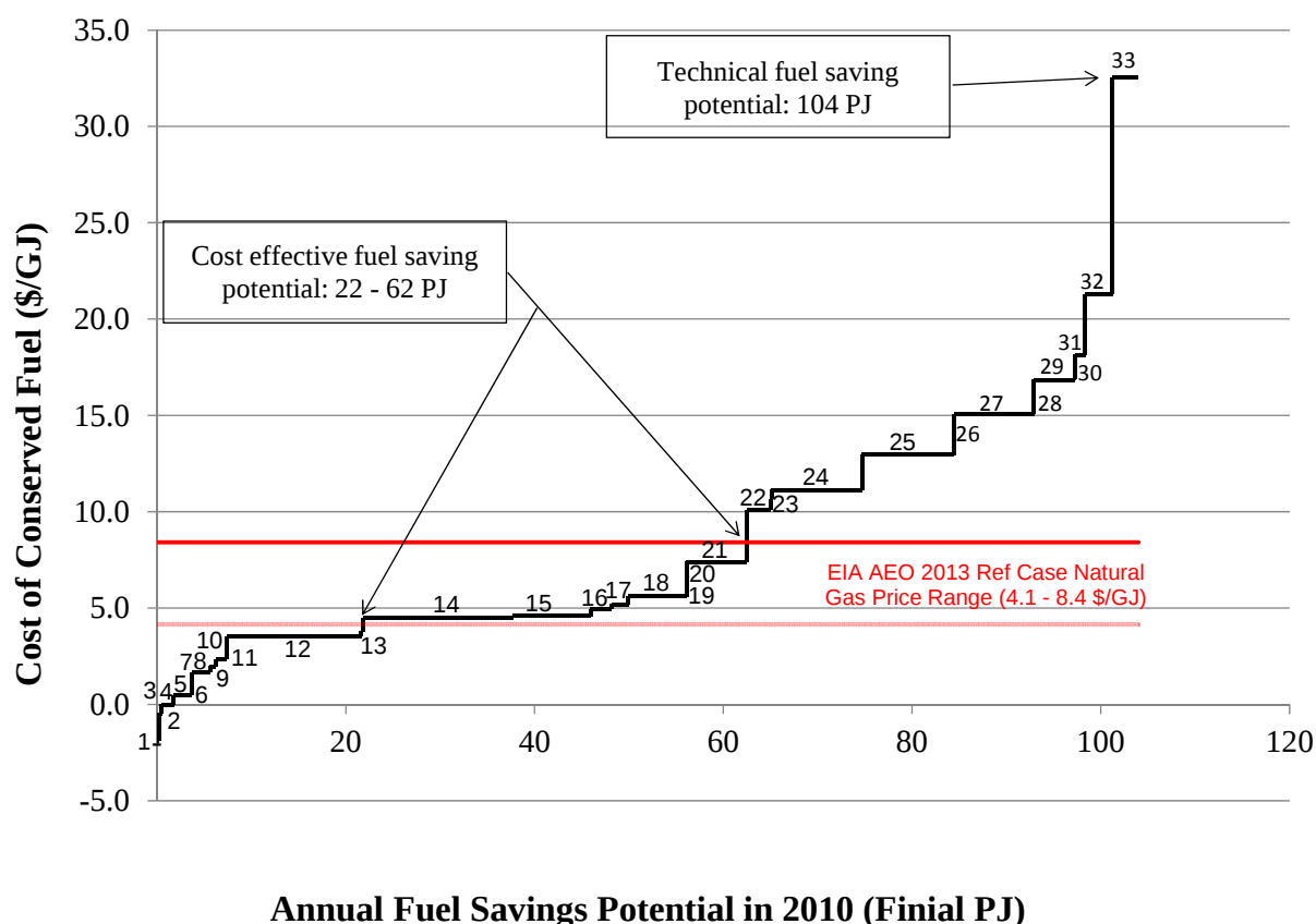
Figure 18 – NTU Cost-of-Conserved Combined Fuel and Associated Electricity Supply Curve
