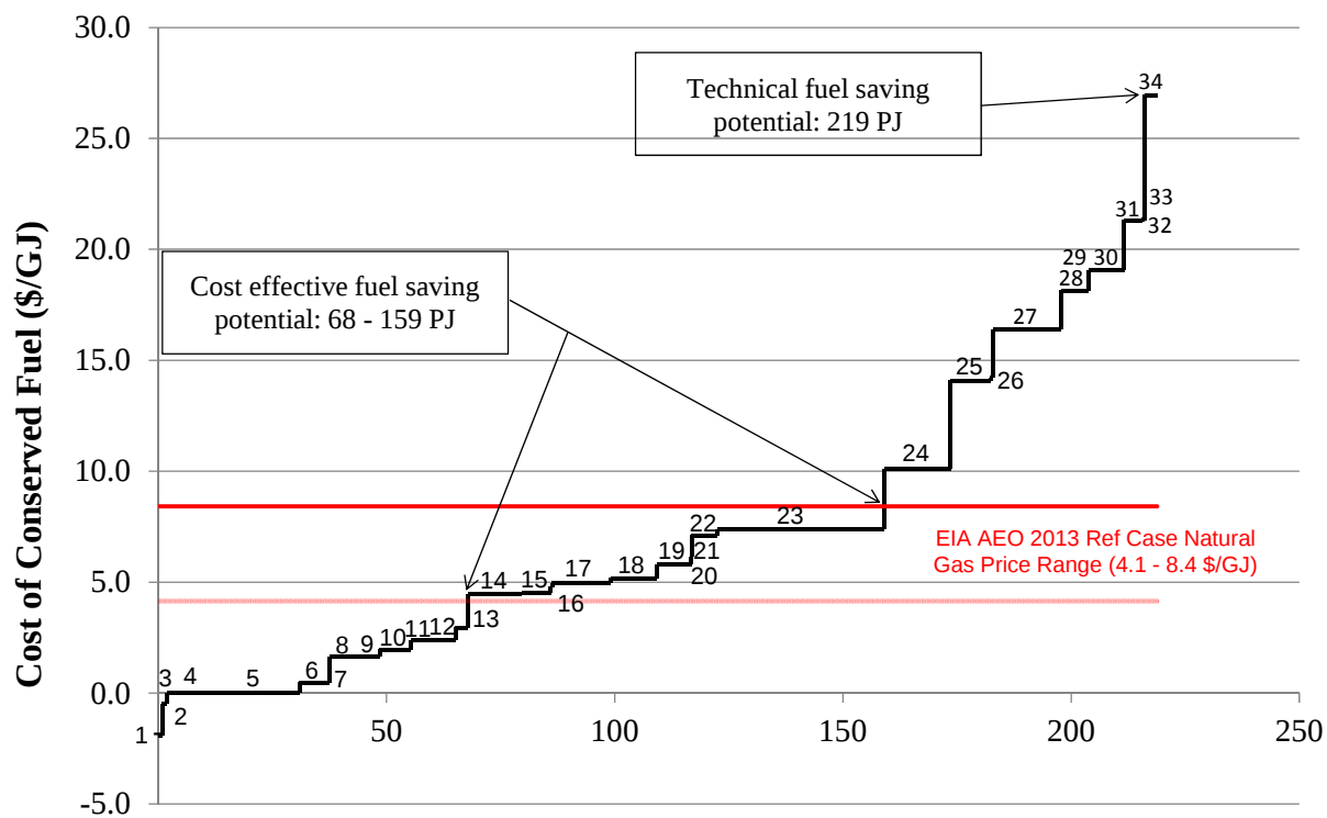
Annual Fuel Savings Potential in 2010 (Finial PJ)
