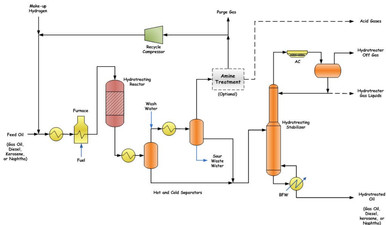
Figure 14 – Hydrotreating Unit (HTU) Process Flow Diagram
