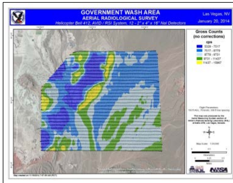
FIGURE 31 GROSS-COUNT CONTOUR OF THE NATURAL BACKGROUND AREA (GOVERNMENT WASH) CREATED USING THE AMS DETECTION SYSTEM AND AMS PROCESSING TECHNIQUES (2014-01-20 PM).
