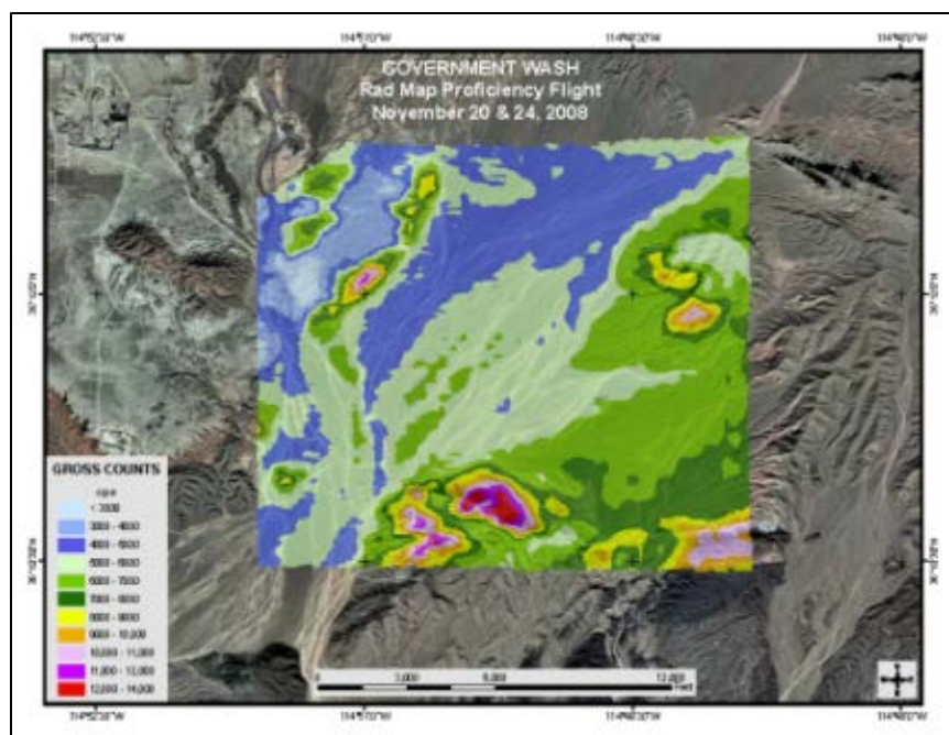
FIGURE 15 RADIATION GROSS COUNTS CONTOUR MAP OF NATURAL BACKGROUND AT GOVERNMENT WASH SITE FROM EARLIER AMS SURVEY DATA.
