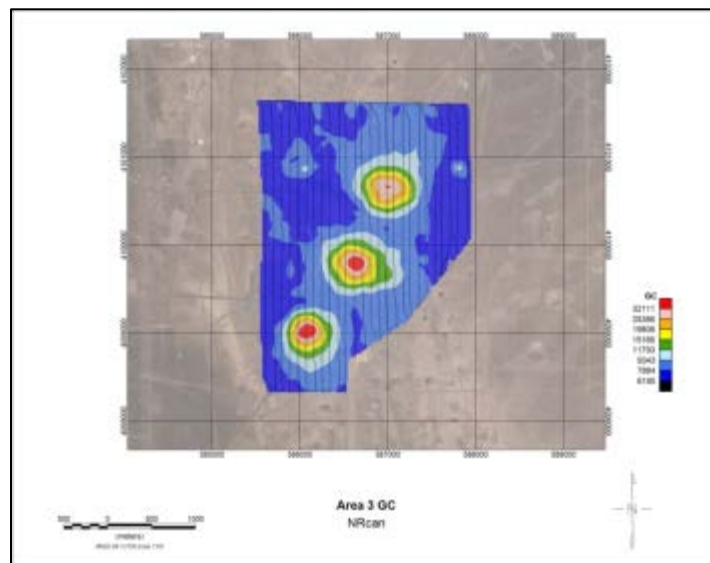
FIGURE 34 CONTOUR OF GROSS ACTIVITY FROM NNSS AREA 3 CREATED USING NRCAN DETECTION SYSTEM AND NRCAN DATA PROCESSING TECHNIQUES. FLIGHT LINES ARE SUPERIMPOSED ON THIS PICTURE. (2014-01-21 AM)
