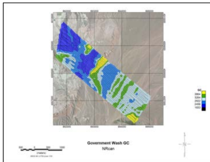
FIGURE 32 GROSS-COUNT CONTOUR OF THE NATURAL BACKGROUND AREA (GOVERNMENT WASH) CREATED USING NRcan DETECTION SYSTEM, FLIGHT PARAMETERS, AND NRcan DATA PROCESSING TECHNIQUES (2014-01-20 AM).
