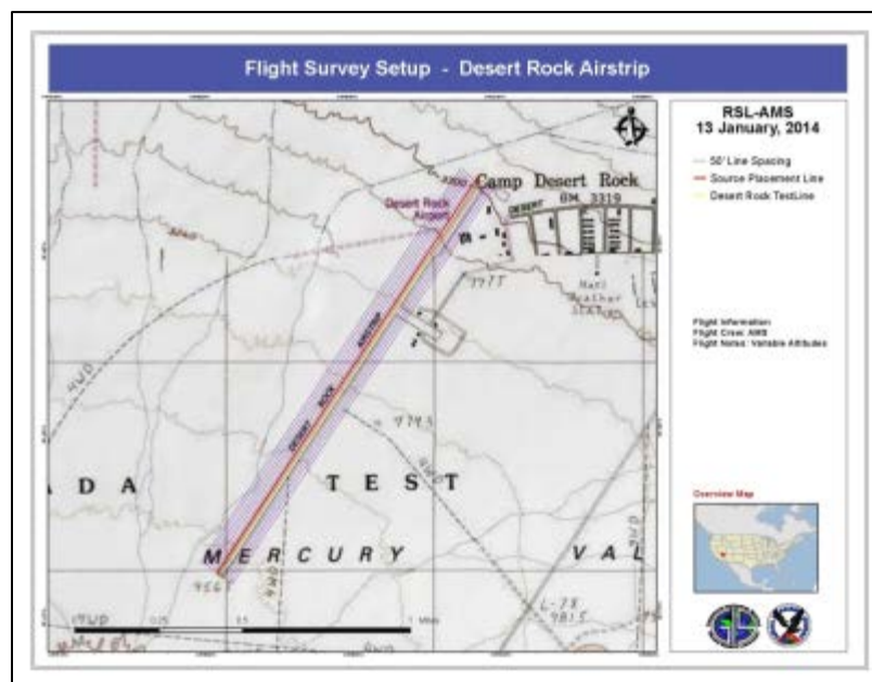
FIGURE 18 SETUP FOR SOURCE OVERFLIGHT AT DRA
