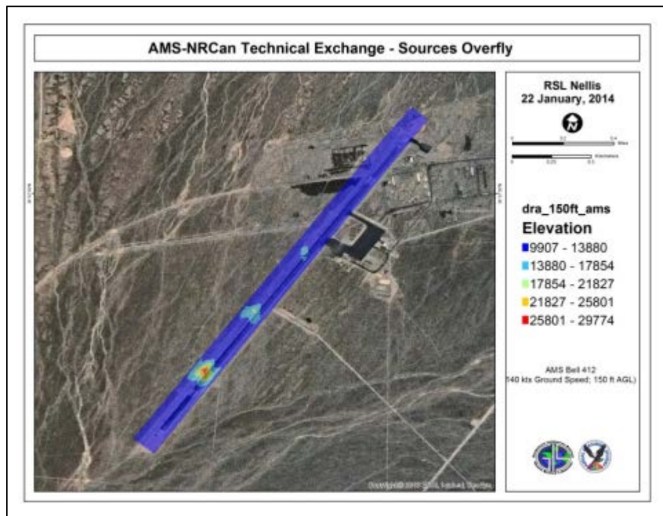
FIGURE 27 AMS RESULTS OF SOURCES OVERFLY AT DESERT ROCK AIRPORT AT 150 FT AGL.
