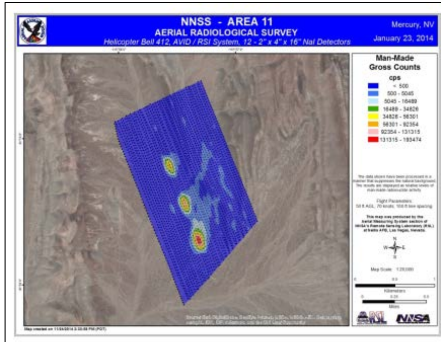
FIGURE 43 CONTOUR OF MAN-MADE ACTIVITY FROM NNSS AREA 11 CREATED USING AMS DETECTION SYSTEM AND AMS DATA PROCESSING TECHNIQUES.
