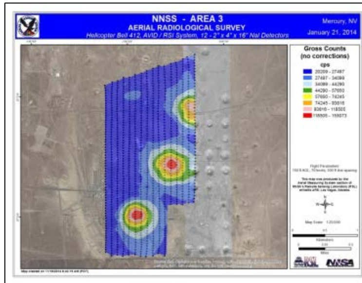
FIGURE 33 CONTOUR OF GROSS ACTIVITY FROM NNSS AREA 3 CREATED USING AMS DETECTION SYSTEM AND AMS DATA PROCESSING TECHNIQUES. FLIGHT LINES ARE SUPERIMPOSED ON THIS PICTURE. (2014-01-21 PM).
