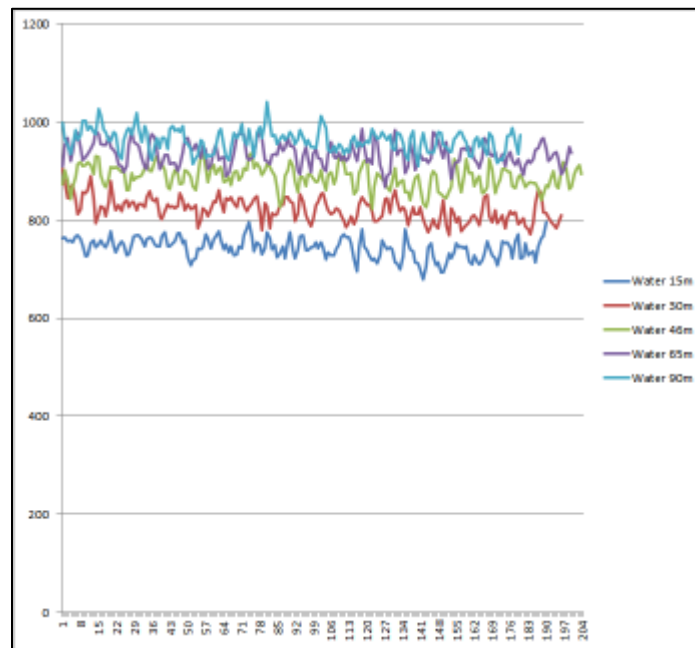
FIGURE 22 COUNT RATE TIME SERIES OVER THE WATER LINE FOR THE NRCAN SYSTEM. THE X AXIS SHOWS THE TIME ALONG THE SURVEY LINE IN SECONDS.
