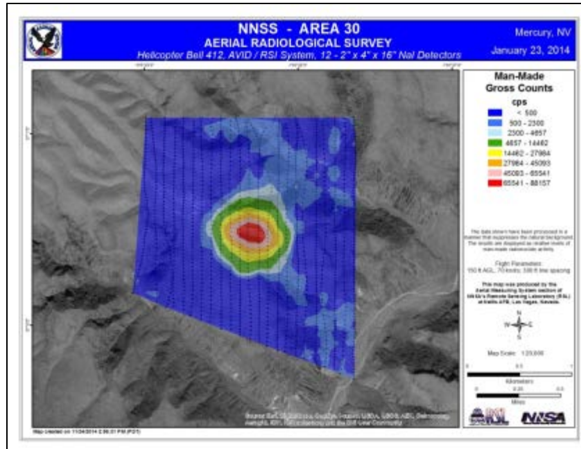
FIGURE 47 CONTOUR OF MAN-MADE ACTIVITY FROM NNSS AREA 30 CREATED USING AMS DETECTION SYSTEM AND AMS DATA PROCESSING TECHNIQUES.
