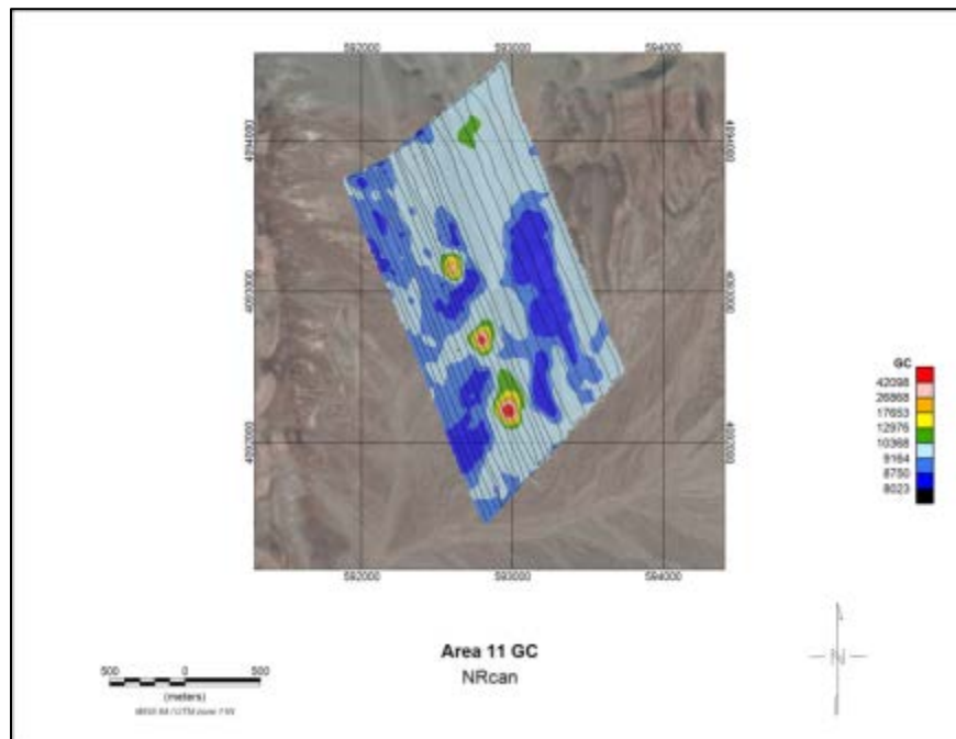
FIGURE 42 CONTOUR OF GROSS ACTIVITY FROM NNSS AREA 11 CREATED USING NRCAN DETECTION SYSTEM AND NRCAN DATA PROCESSING TECHNIQUES. (2014-01-23 AM)
