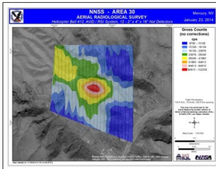
FIGURE 45 CONTOUR OF GROSS ACTIVITY FROM NNSS AREA 30 CREATED USING AMS DETECTION SYSTEM AND AMS DATA PROCESSING TECHNIQUES. (2014-01-23 AM)
