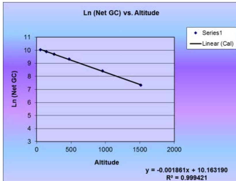
FIGURE 23 AMS RESULTS OF ALTITUDE SPIRAL OVER LAKE MOHAVE CALIBRATION RANGE. PLOTTED AS LOG OF NET GC.
