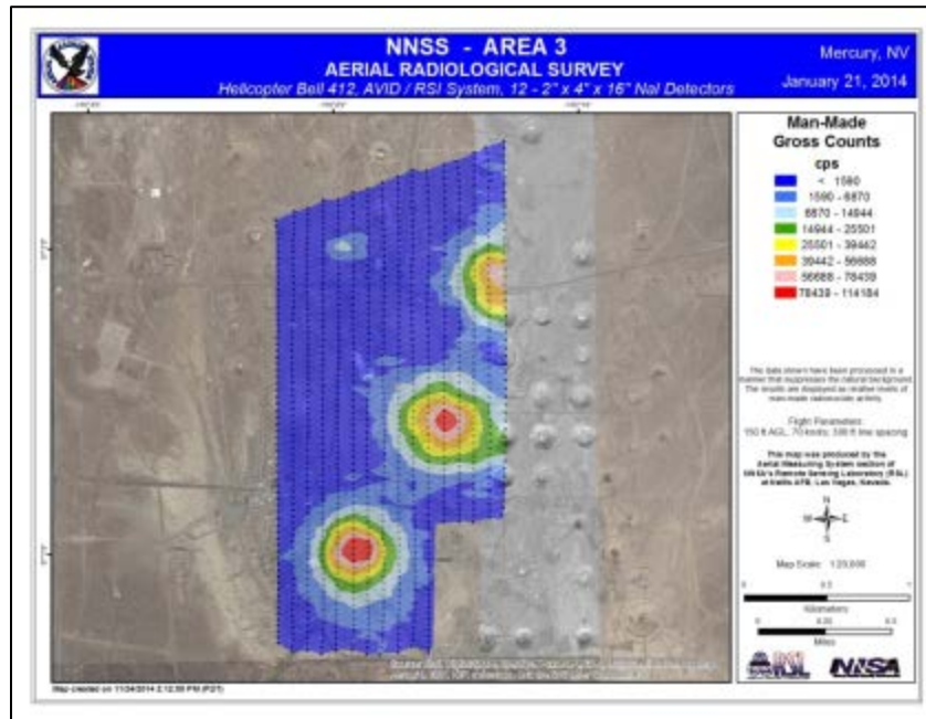
FIGURE 35 CONTOUR OF MAN-MADE ACTIVITY FROM AREA 3 CREATED USING AMS DETECTION SYSTEM AND AMS DATA PROCESSING TECHNIQUES.
