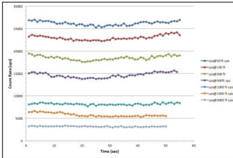
FIGURE 19 NET COUNT RATE TIME SERIES OVER THE LAND CALIBRATION LINE FOR THE AMS SYSTEM.
