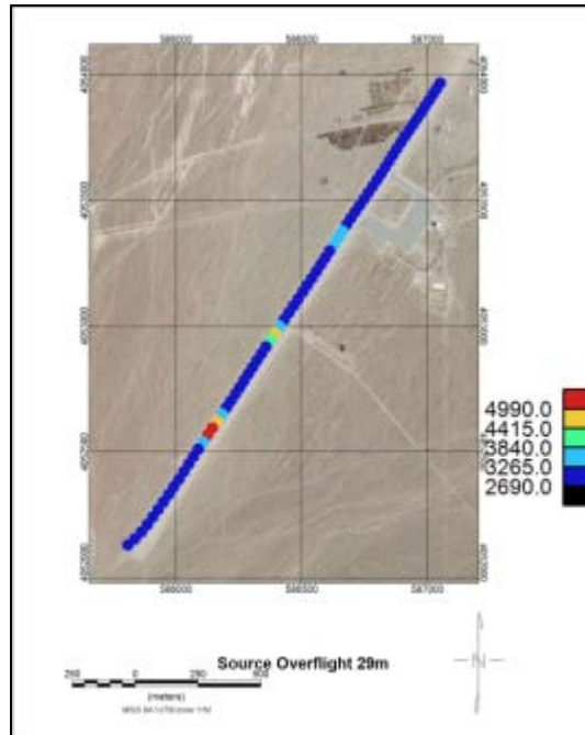
FIGURE 29 GROSS-COUNT RESULT FOR THE 30 M (~100FT) OVERFLIGHT.
