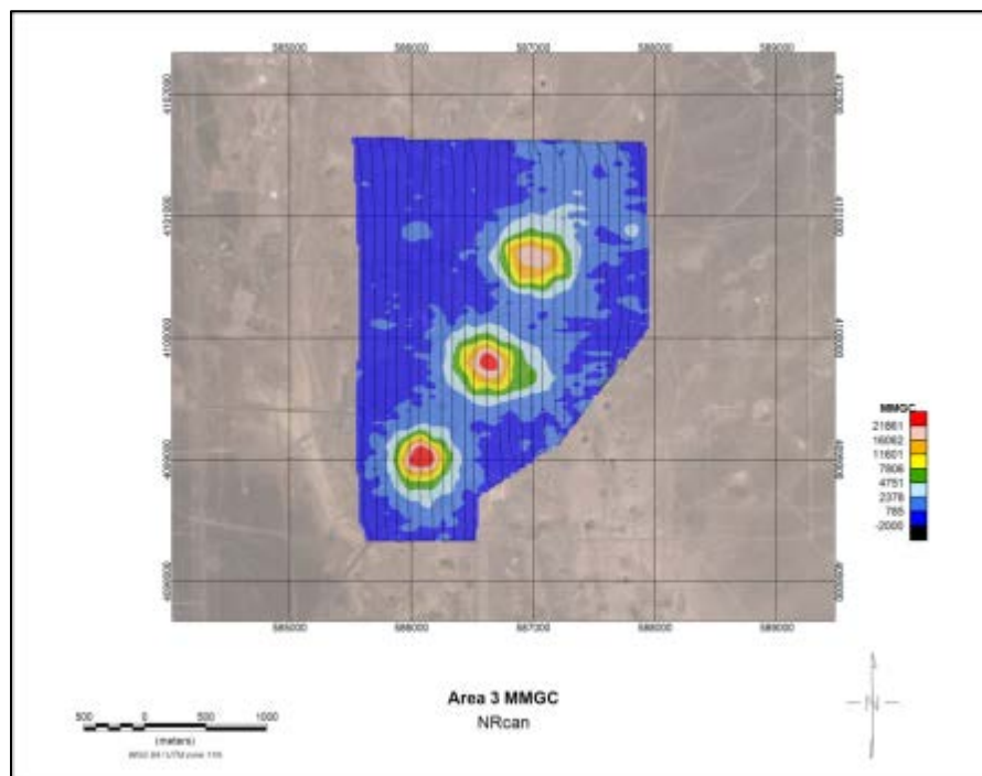
FIGURE 36 CONTOUR OF MAN-MADE ACTIVITY FROM NNSS AREA 3 CREATED USING NRCAN DETECTION SYSTEM AND NRCAN DATA PROCESSING TECHNIQUES
