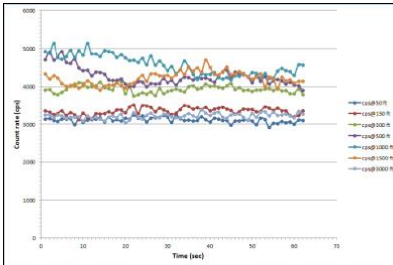
FIGURE 20 COUNT RATE TIME SERIES OVER THE WATER LINE FOR THE AMS SYSTEM.
