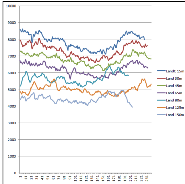
FIGURE 21 COUNT RATE TIME SERIES OVER THE LAND LINE FOR THE NRCAN SYSTEM. THE X AXIS SHOWS THE TIME ALONG THE SURVEY LINE IN SECONDS. THE LARGER VARIATION IN THE COUNT RATE FROM SAMPLE TO SAMPLE REFLECTS THE SMALLER ACTIVE DETECTOR VOLUME USED FOR THE NRCAN SYSTEM.
