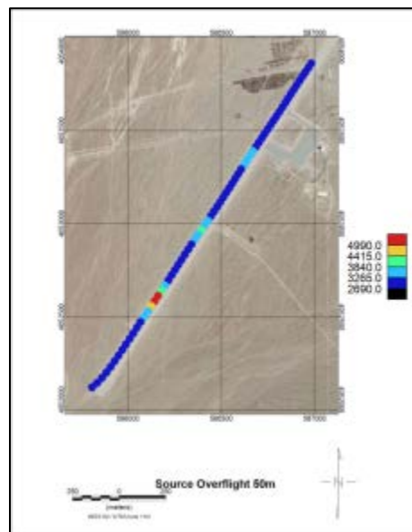
FIGURE 30 TOTAL COUNT RESULT FOR THE 50M (~150FT) OVERFLIGHT.
