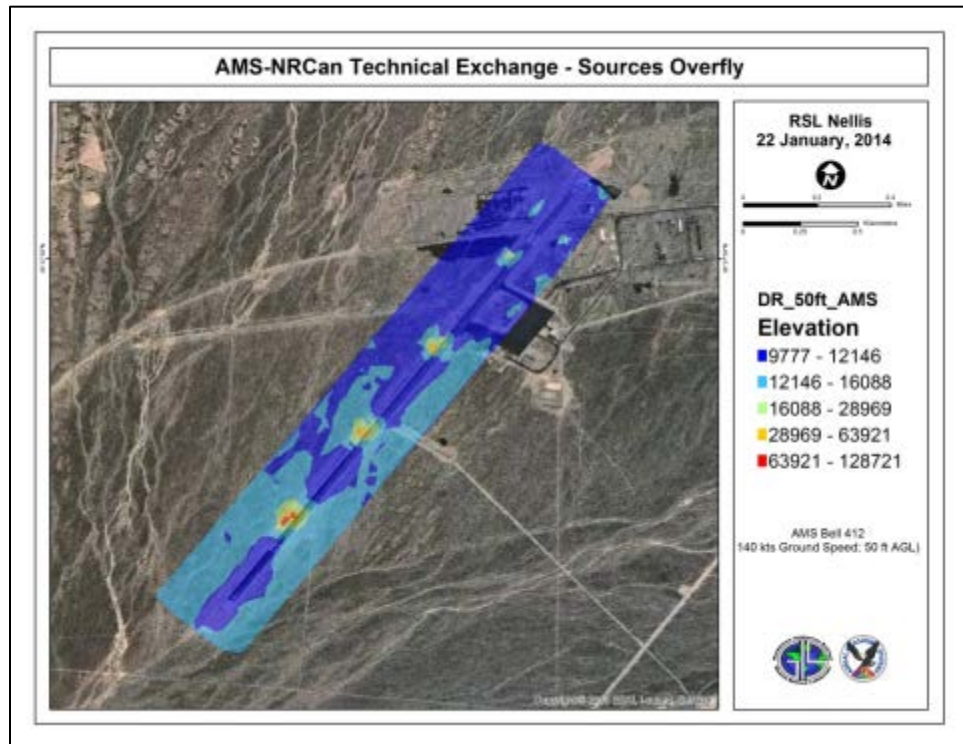
FIGURE 25 AMS RESULTS OF SOURCES OVERFLY AT DESERT ROCK AIRPORT AT 50 FT AGL.
