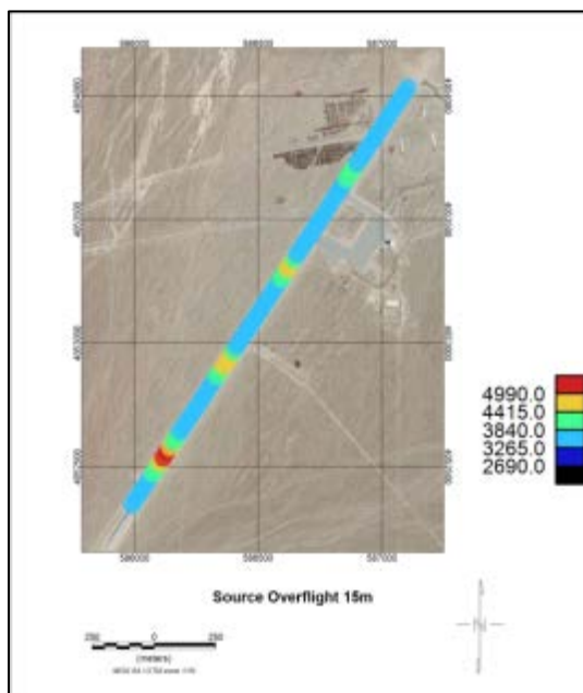
FIGURE 28 NRCAN GROSS-COUNT RESULT FOR THE 15 M (~50 FT) OVERFLIGHT.
