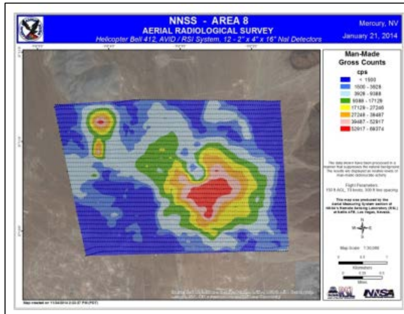
FIGURE 39 CONTOUR OF MAN-MADE ACTIVITY FROM NNSS AREA 8 CREATED USING AMS DETECTION SYSTEM AND AMS DATA PROCESSING TECHNIQUES.
