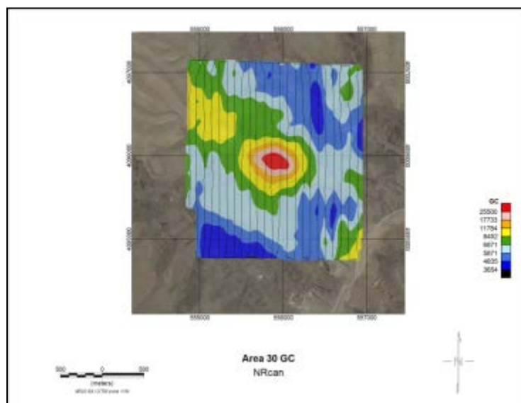
FIGURE 46 CONTOUR OF GROSS ACTIVITY FROM NNSS AREA 30 CREATED USING NRCan DETECTION SYSTEM AND NRCan DATA PROCESSING TECHNIQUES. (2014-01-22 PM)
