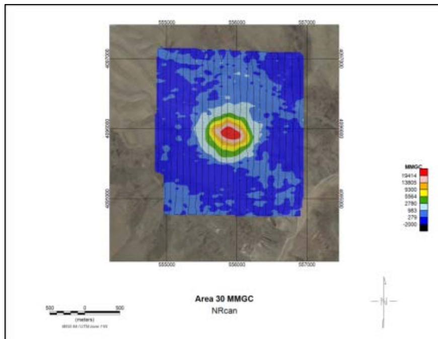
FIGURE 48 CONTOUR OF MAN-MADE ACTIVITY FROM NNSS AREA 30 CREATED USING NRCan DETECTION SYSTEM AND NRCan DATA PROCESSING TECHNIQUES.
