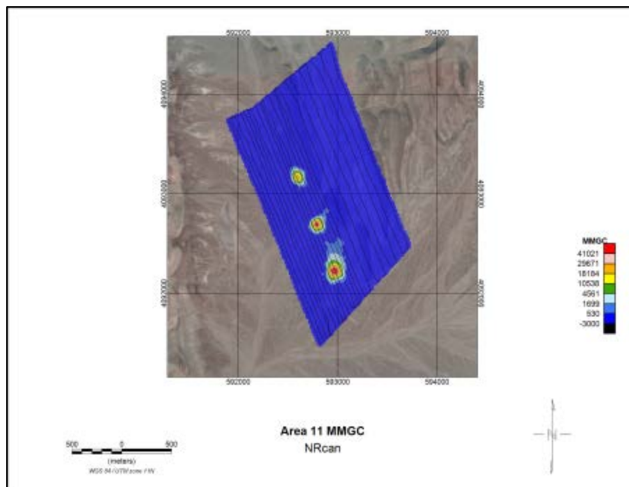
FIGURE 44 CONTOUR OF MAN-MADE ACTIVITY FROM NNSS AREA 11 CREATED USING NRCAN DETECTION SYSTEM AND NRCAN DATA PROCESSING TECHNIQUES.
