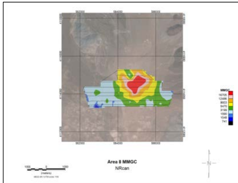
FIGURE 40 CONTOUR OF MAN-MADE ACTIVITY FROM NNSS AREA 8 CREATED USING NRCAN DETECTION SYSTEM AND NRCAN DATA PROCESSING TECHNIQUES.
