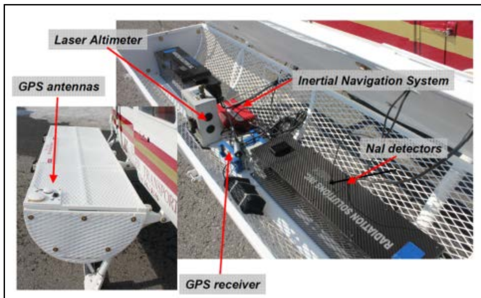
FIGURE 9 NRCAN RSI DETECTORS AND SUPPORT INSTRUMENTATION: 2 DETECTORS, LASER, RADAR ALTIMETERS AND GYROSCOPES.
