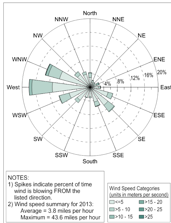
Figure 1-3 Annual Wind Patterns
