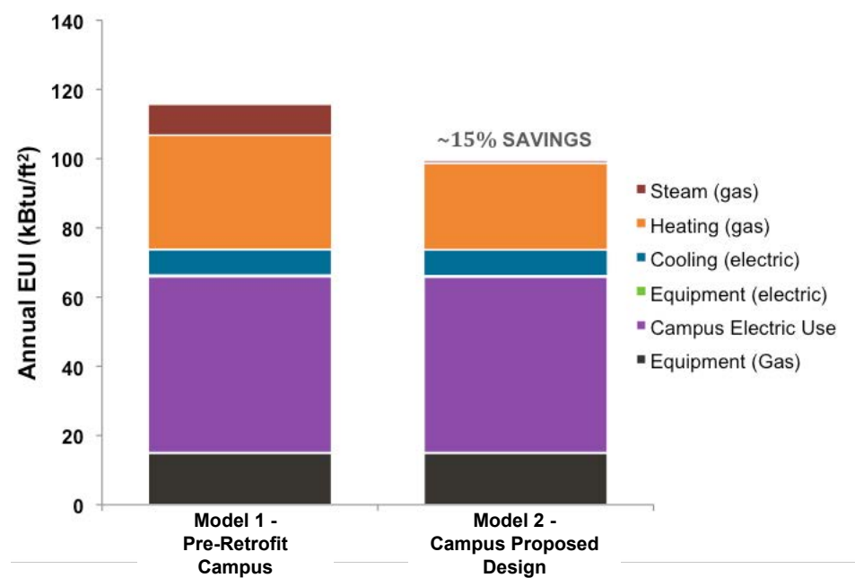
Comparing EUI of Pre-Retrofit and Proposed Design for the Campus
