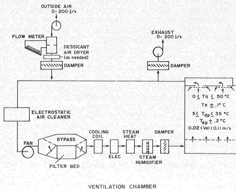
Fig. 4. Schematic view of environmental chamber and control equipment. Arrows in box at right portray the flow of air from the plenum beneath the floor to the return ducts in the ceiling.
