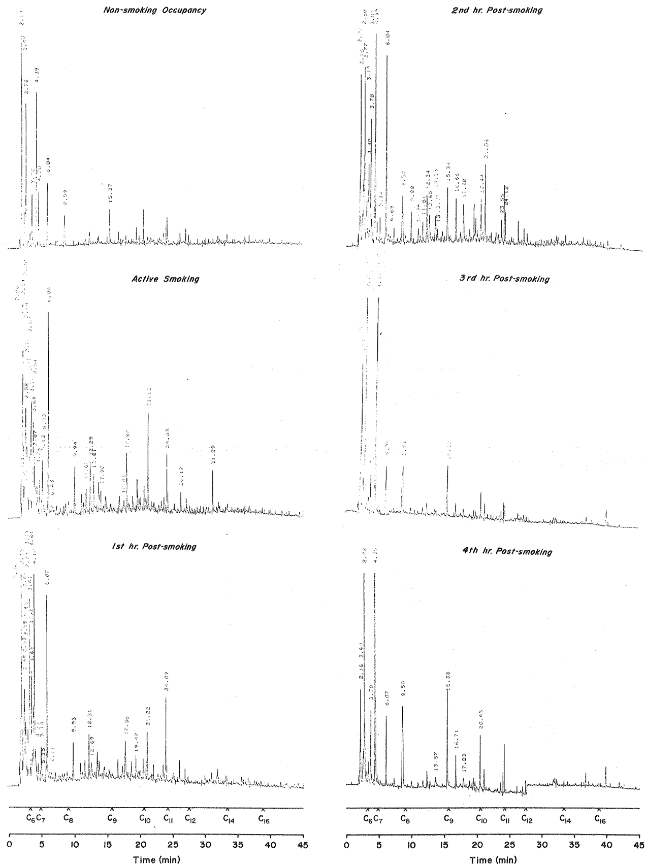
Fig. 52. Gas chromatograms for successive 1-hr samples from the period of nonsmoking occupancy (4 occupants), active smoking (12 cigarettes in 1.5-hr), and four subsequent hours. Peaks annotated with retention times represent concentrations of 0.1 ppm (v/v in air) or above. The cumulative area under the annotated peaks provided a rough indication of total hydrocarbons (see Fig. 53). The scale at the bottom indicates, for reference, retention times of various normal alkanes.
