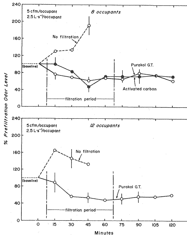
Fig. 47. Showing how Purakol G.T. and activated carbon reduced occupancy odor (butanol matching in ppm expressed as percentage of prefiltration level) in comparison to a condition of no filtration. Ventilation rate equalled 5 cfm ( 2.5 \text{ L}\cdot\text{s}^{-1} ) per occupant. Bars depict standard errors. Matched level in the period just before filtration, arbitrarily denoted t=0 , averaged approximately 83 ppm.
