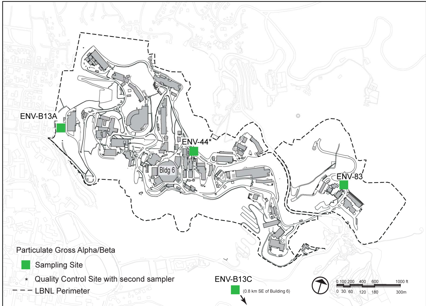
Figure 4-2 Ambient Air Monitoring Network Sampling Locations
