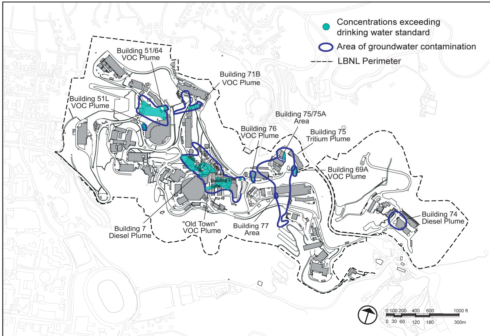
Figure 4-6 Locations of Plumes and Extent of Groundwater Contamination Above Drinking Water Standards (September 2010)
