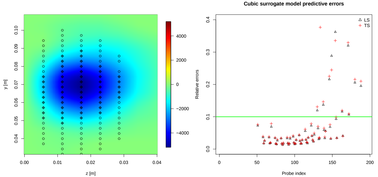
Figure 4. Left: Plot of experimental vorticity inside \mathcal{W} with the probes constituting \mathcal{P}_* overlaid on it and marked with \circ . Right: Comparison of \overline{\delta}_{LS}^{(p)} and \overline{\delta}_{TS}^{(p)} for all 108 probes in \mathcal{P}_* . We note that the two relative errors are of the same magnitudes, indicating that there is little overfitting of the surrogates. We also see that for some probes, the relative errors can be big i.e., surrogates are not necessarily accurate for all probes. Some of the errors also lie outside the range of the vertical axis and are not plotted. The green line at 10% error demarcates the probes that can be used in calibration; the rest of the polynomial surrogates are too inaccurate for any practical use. The probes which lie under the green line are plotted on the right with + symbols.
