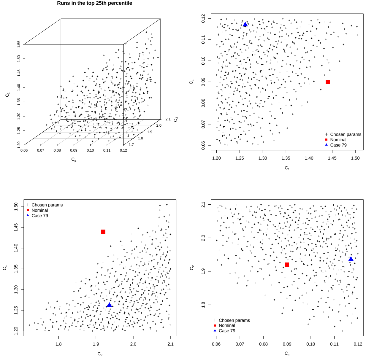
Figure 2. The set of N_s points in the (C_\mu, C_{\epsilon 2}, C_{\epsilon 1}) space that constitute \mathcal{R} . Top left: Scatterplot of the points describing \mathcal{R} . Top right: The projection on the (C_{\epsilon 1}, C_\mu) plane. \mathbf{C}_{nom} and the best parameter combination found in [1], called Case 79, are also plotted. Bottom: Projections on (C_{\epsilon 2}, C_{\epsilon 1}) and (C_\mu, C_{\epsilon 2}) space show that \mathbf{C}_{nom} does not lie in \mathcal{R} .
