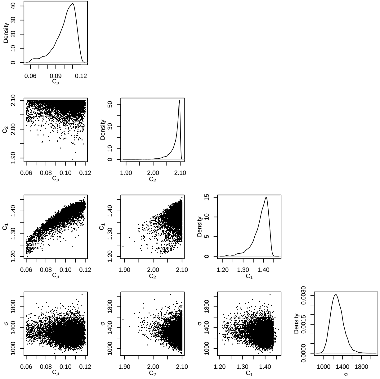
Figure 7. Pairwise plots for the parameters calibrated in Fig. 5. There is a clear correlation between (C_\mu, C_{\epsilon 1}) and (C_\mu, C_{\epsilon 2}) in the posterior.
