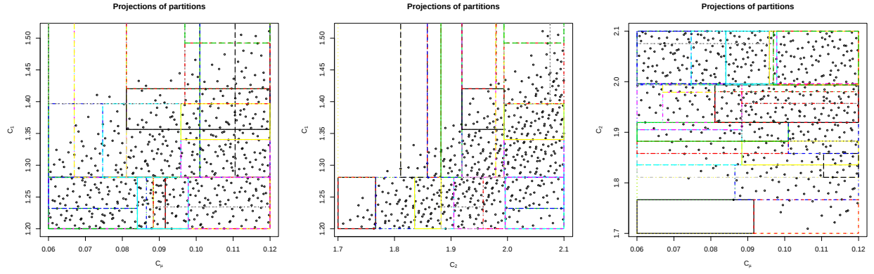
Figure 3. The highest probability or maximum a posteriori partitioning tree of the N_s points in \mathcal{C} that define \mathcal{R} . The points that lie outside \mathcal{R} are used in the calculation of the tree, but are not plotted here because there are too many of them for a clear plot. They inhabit the blank regions of the plots above and are uniformly distributed there. The boxes are the nodes of the tree projected on 2D slices. Data in leaf nodes are approximated with a linear model.
