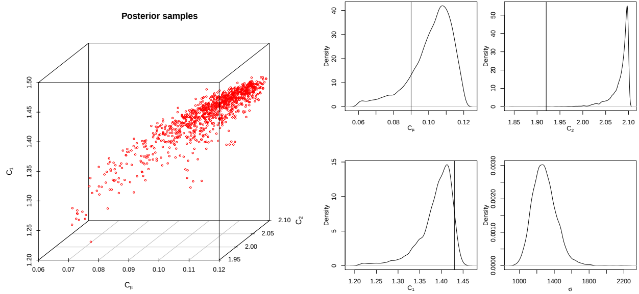
Figure 5. Left: 1000 points sampled randomly from the posterior distribution and plotted in the (C_\mu, C_{\epsilon 2}, C_{\epsilon 1}) space. We see that the posterior distribution has a support that lies inside \mathcal{R} , but the density is clearly concentrated at the far top right corner of the parameter space. Right: Marginalized PDFs for C_\mu, C_{\epsilon 2}, C_{\epsilon 1}, \sigma computed as a solution to Eq. 3. The nominal values of the parameters are shown using the vertical line. The MAP estimates of all parameters except C_{\epsilon 1} vary significantly from their nominal value.
