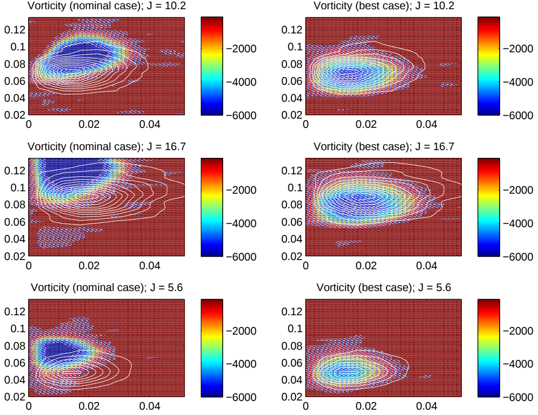
Figure 10. Left column: Streamwise vorticity in the crossplane computed using \mathbf{C}_{nom} , overlaid with vorticity, as measured in experiments. J = 10.2, 16.7, 5.6 for the top, middle and bottom rows. Right column: Crossplane streamwise vorticity predicted using the “optimal” values of (C_\mu, C_{\epsilon 2}, C_{\epsilon 1}), \mathbf{C}_{opt} . Qualitatively, the agreement is quite good. The improvement over \mathbf{C}_{nom} (left column) is stark.
