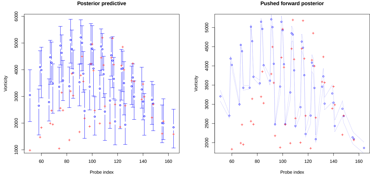
Figure 8. Left: The posterior predictive test using the posterior distribution plotted in Fig. 5. Experimental streamwise vorticity on the crossplane is plotted using +; the median and interquartile ranges computed from 100 PPT simulations are plotted using o and error bars. Right: The same predictions but without the addition of the data - model mismatch \sim \mathcal{N}(0, \sigma^2) . Median predictions are in o and the dashed lines indicate the interquartile range. We see that parametric variability has hardly any effect on the vorticity predictions.
