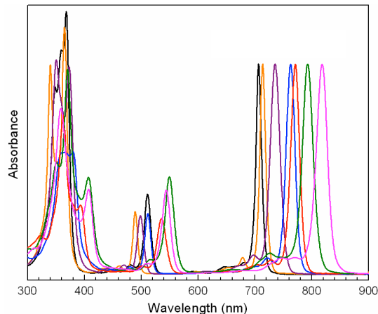
Chart 6. Bacteriopheophytin a and auxochromic synthetic analogues.
