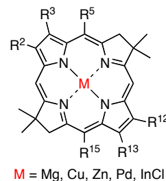
Chart 9. Metallo-bacteriochlorins.
