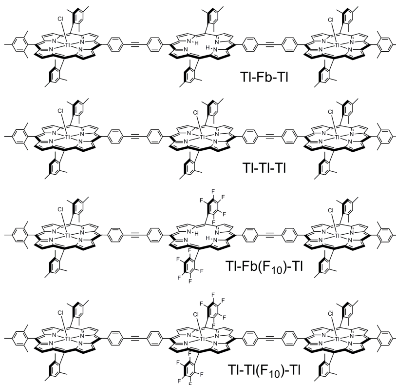
Chart 2. Triads for hole-transfer studies.
