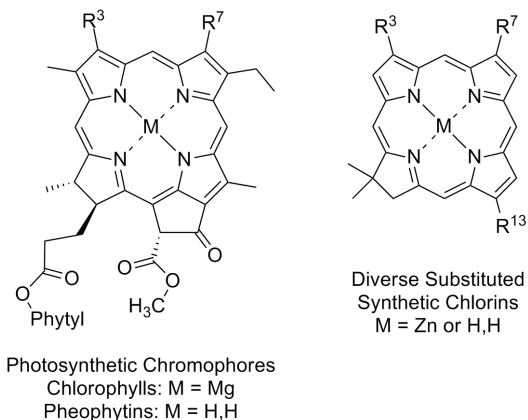
Chart 4. Natural chlorophylls and auxochrome-substituted synthetic analogues.
