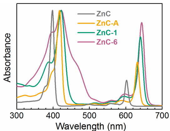
Figure 4. Normalized absorption spectra of the zinc chlorins in toluene.
