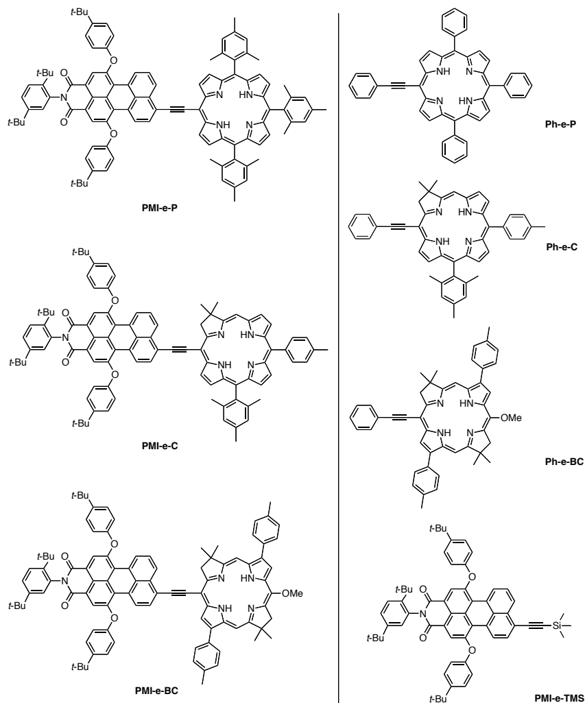
Chart 10. Perylene–tetrapyrrole dyads (left) and benchmarks (right).
