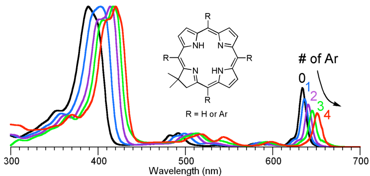
Figure 3. Absorption spectra of chlorins with meso-aryl substituents.
