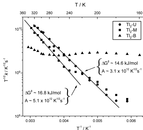
Figure 2. Marcus-equation plots for the monocations of TI 2 -U , TI 2 -M , and TI 2 -B .
