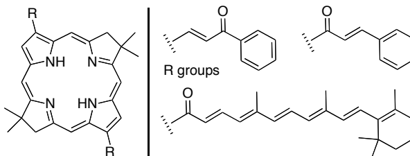
Chart 7. Bacteriochlorin-chalcones.
