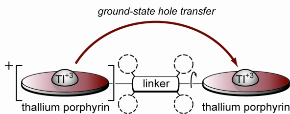
Chart 1. Torsionally constrained dyads.
