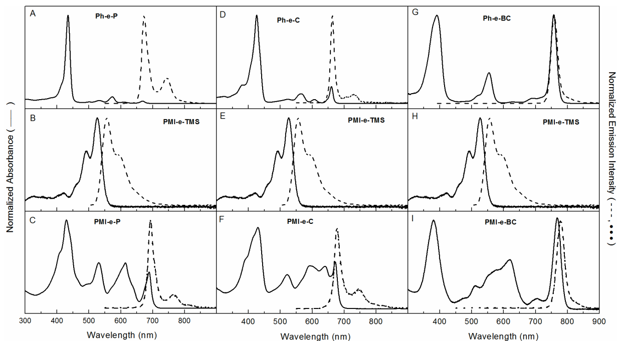
Figure 6. Absorption (solid) and fluorescence spectra of the perylene–tetrapyrrole arrays. Note the panchromatic absorption of the dyads (bottom row). In each column, the dyad absorption is not the sum of the parts (tetrapyrrole + perylene).
