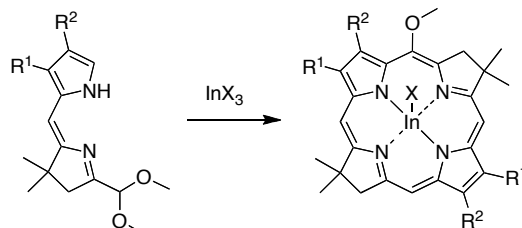
Chart 8. Synthesis of indium bacteriochlorins.
