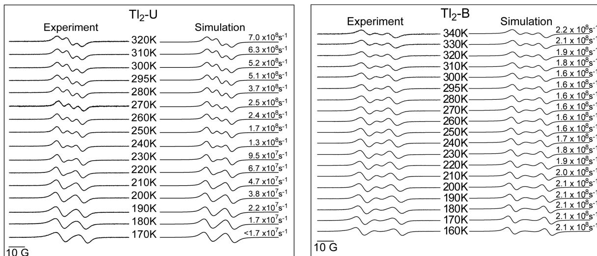
Figure 1. Variable-temperature EPR spectra the unhindered dyad TI 2 -U (left panel) and bishindered dyad TI 2 -B . (right panel). The left traces in each panel are the experimental spectra and the right traces are simulations and derived hole/electron-transfer rates.
