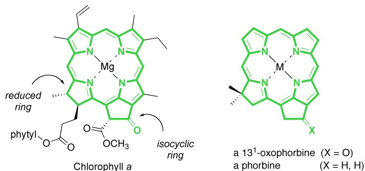
Chart 3. Structure of chlorophyll a and sparsely substituted synthetic analogues.
