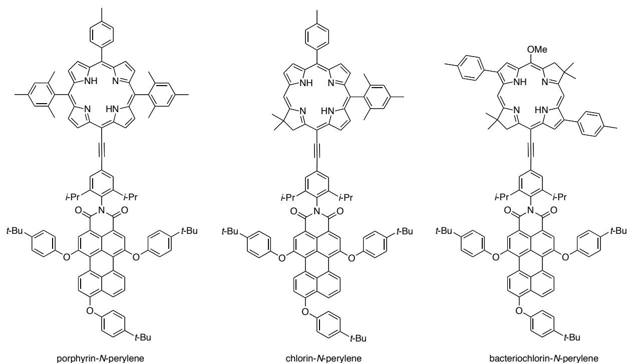
Chart 11. Perylene–tetrapyrrole dyads (moderately coupled) for studies of energy transfer.
