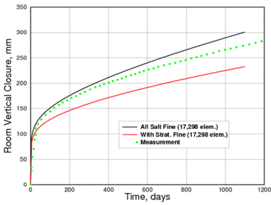
Figure 4.3. Benchmarking Room D deformation.
