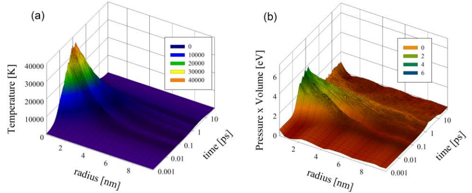
FIG. 10. (a) Temperature and (b) pressure spikes for a simulated 22 keV/nm fission fragment in an \text{UO}_2 system with \tau_{\text{ep}} of 150 fs. While no track was observed for fission fragments, a stress zone from oxygen defect clusters may be observed near the simulated fission fragment path.
