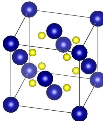
FIG. 1. Uranium dioxide crystallizes into a fluorite structure (space group Fm\bar{3}m ). Uranium atoms are blue (dark) and oxygen atoms are yellow (light).
