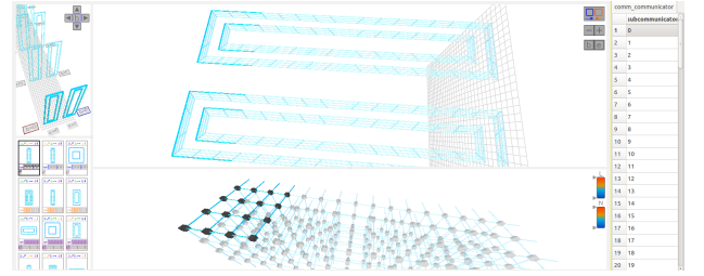
Fig. 10: Single X sub-communicator under the Tile mapping. The 4D slices show this sub-communicator occupies adjacent C and D links for both E=0 and E=1. The 3D slice shows detail in the E=0 subtorus.
