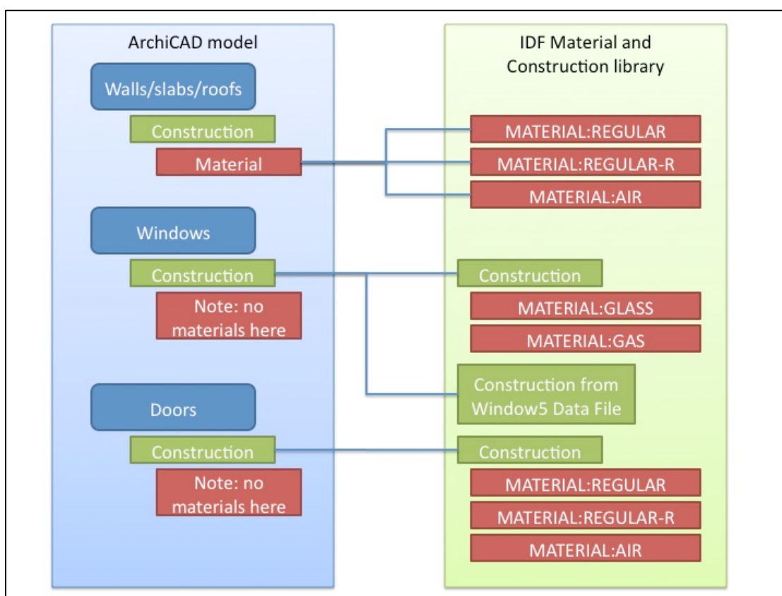
Figure 5: Material and Construction mappings for walls, slabs, roofs, doors and windows from ArchiCAD to EnergyPlus
