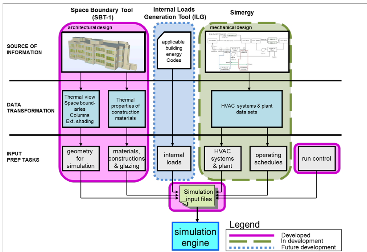
Figure 1: Implementation of the methodology for semi-automated building energy performance simulation
