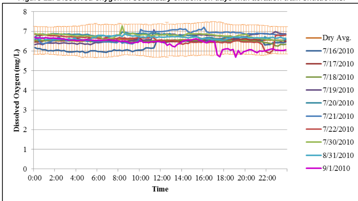
Figure 12: Dissolved oxygen in secondary effluent on days with aeration train shutdowns.
