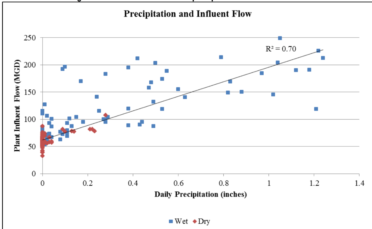
Figure A-7: Correlation between precipitation and influent flow
