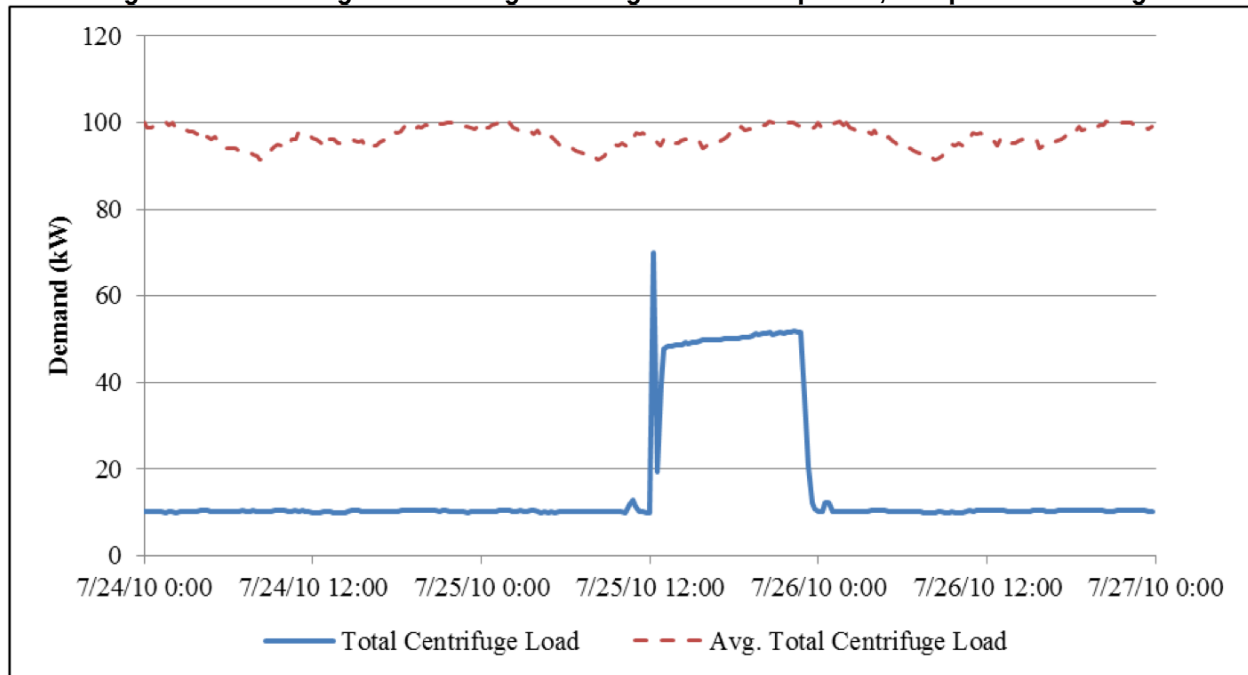
Figure 13: Centrifuge load during centrifuge shutdown period, compared to average
