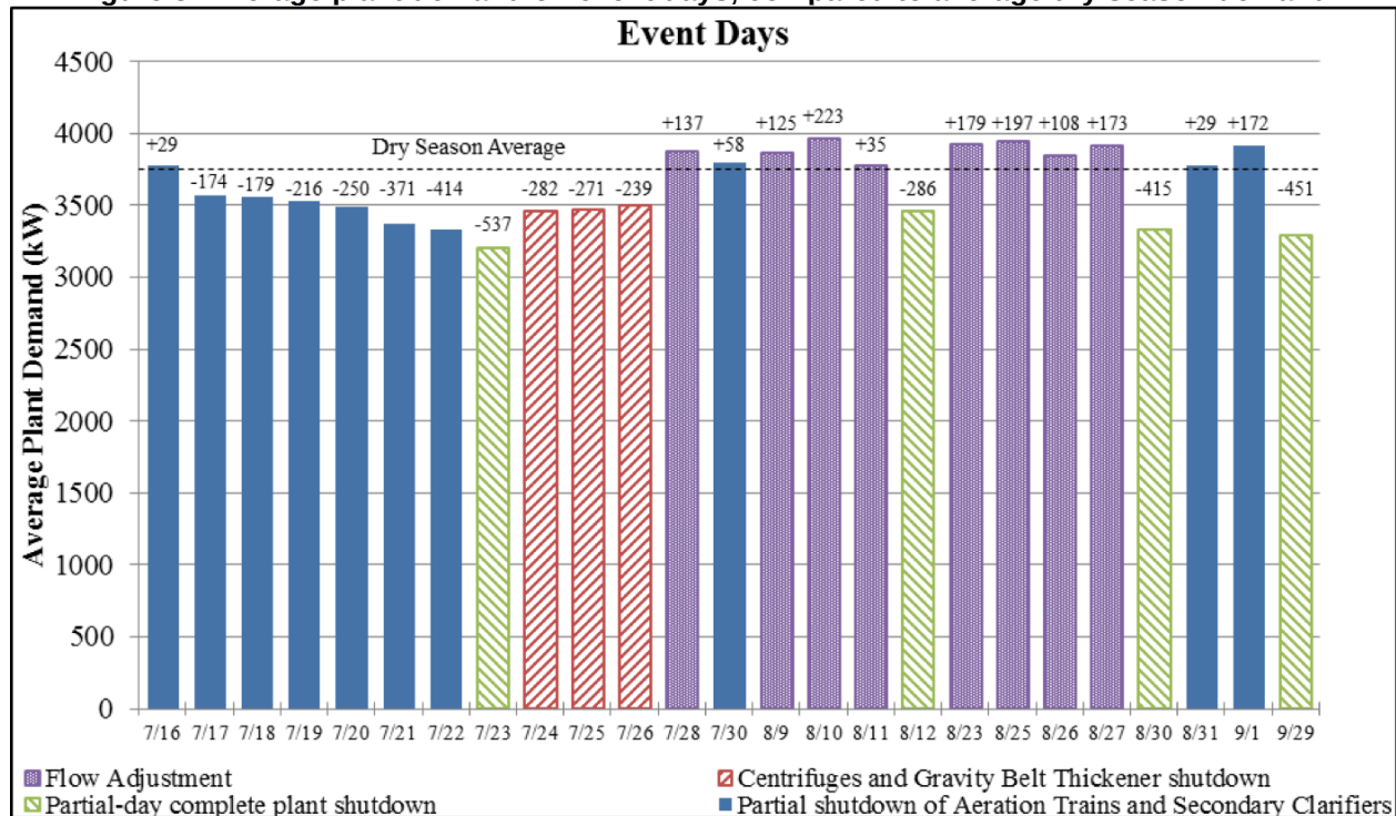
Figure 8: Average plant demand on event days, compared to average dry season demand
