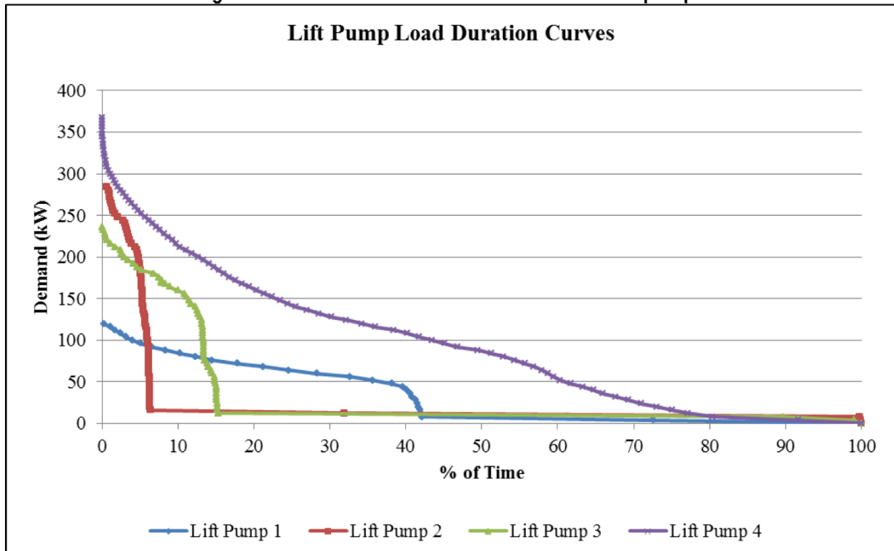
Figure A-13: Load curves for four submetered lift pumps
