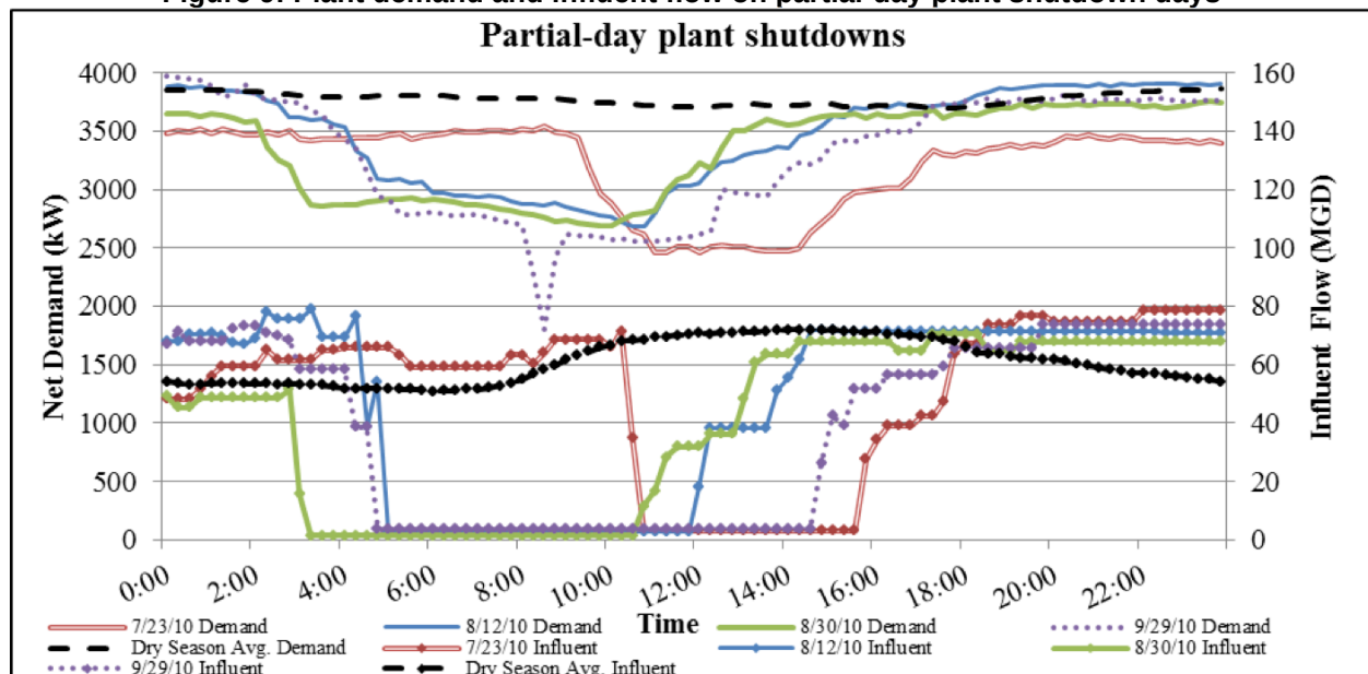
Figure 9: Plant demand and influent flow on partial-day plant shutdown days
