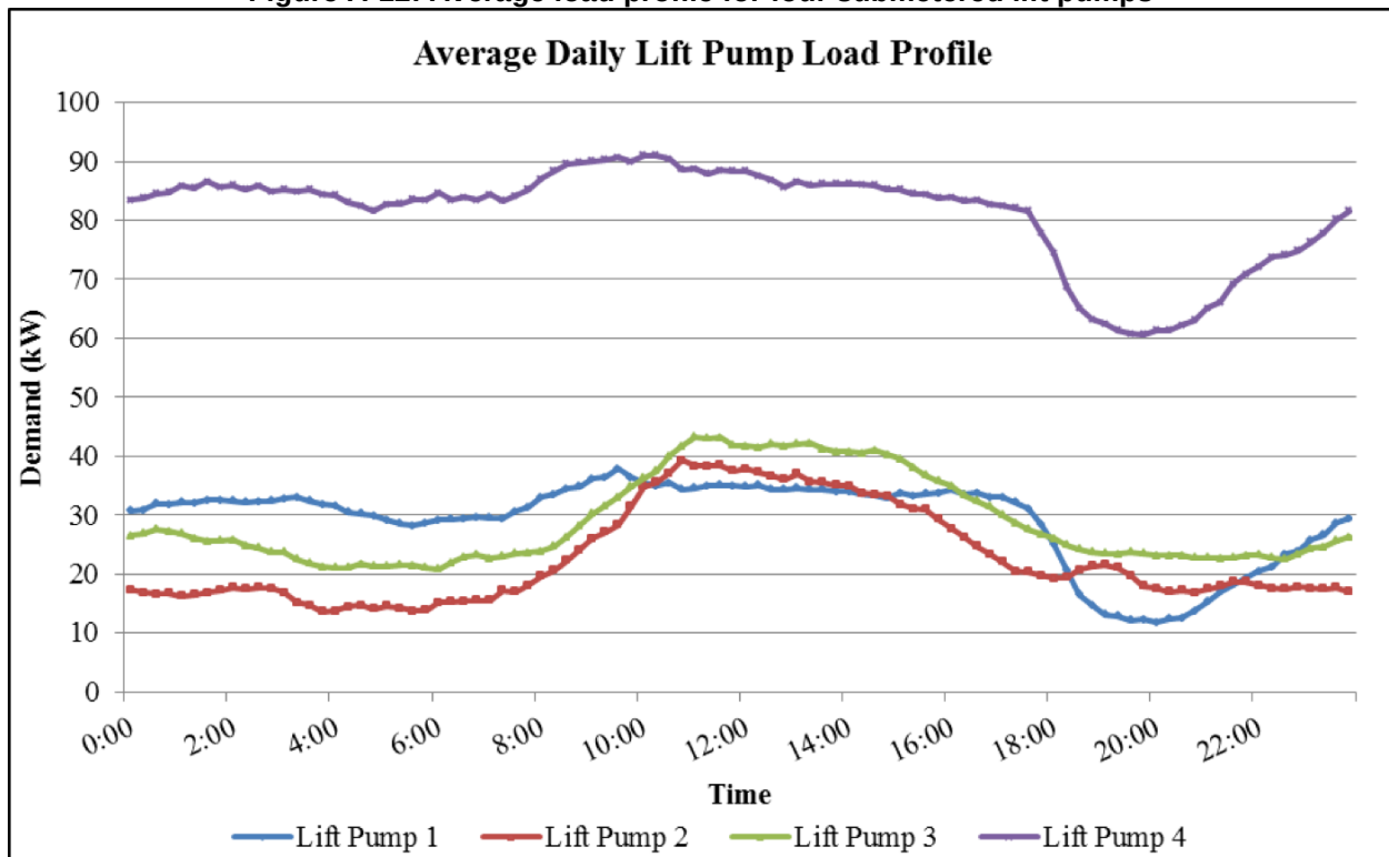
Figure A-12: Average load profile for four submetered lift pumps
