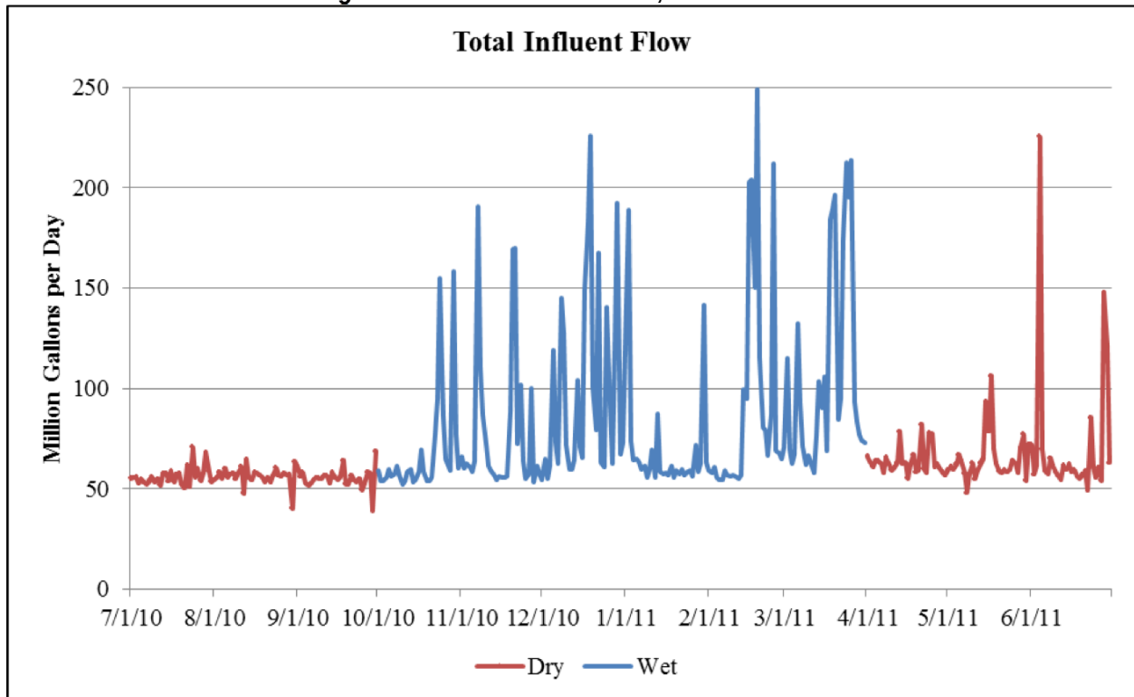
Figure A-3. Plant influent flow, 7/1/10-6/30/11
