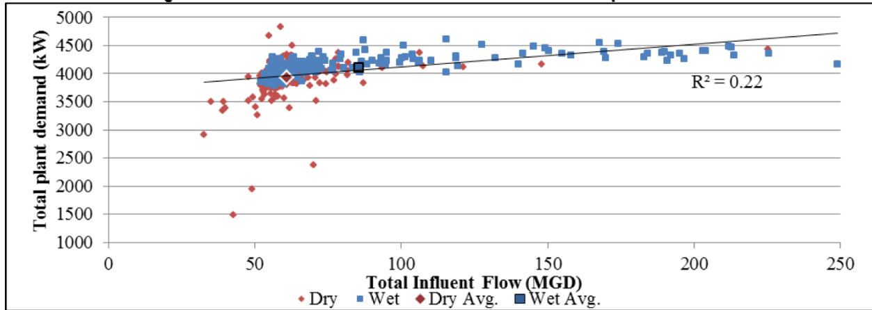
Figure 6: Correlation between influent flow and total plant demand
