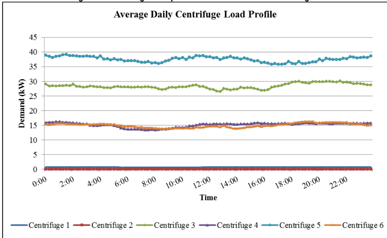
Figure A-9: Average load profile for six submetered centrifuges
