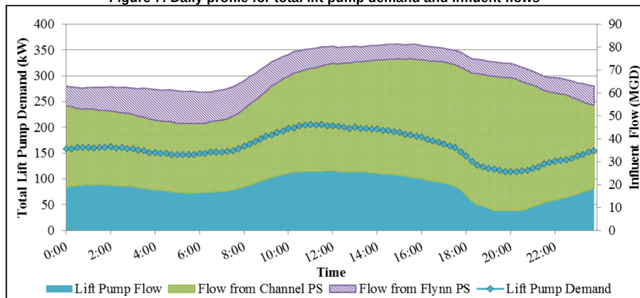
Figure 7: Daily profile for total lift pump demand and influent flows
