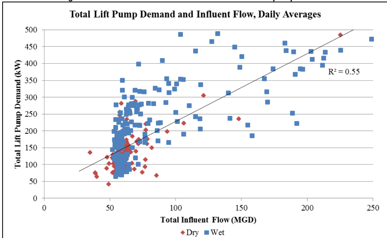
Figure A-14: Correlation between influent flow and lift pump demand
