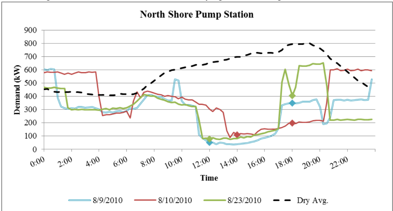
Figure 15: Demand from North Shore Pumping Station during shutdown events.
