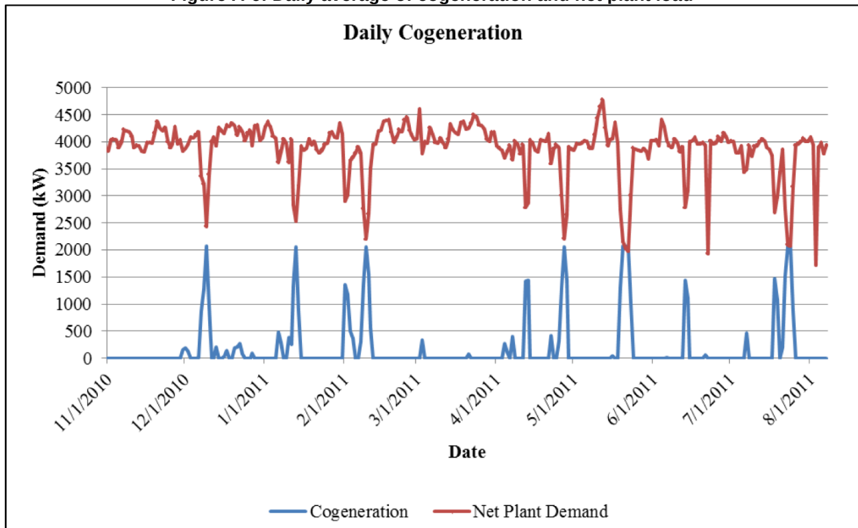
Figure A-6: Daily average of cogeneration and net plant load
