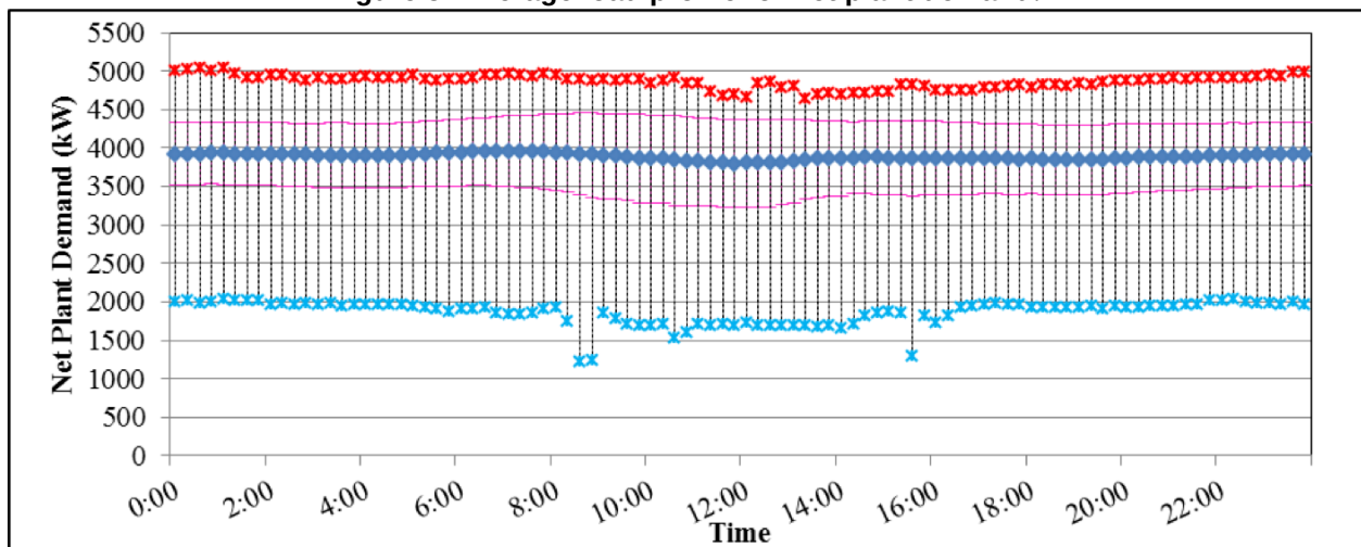
Figure 5: Average load profile for net plant demand.
