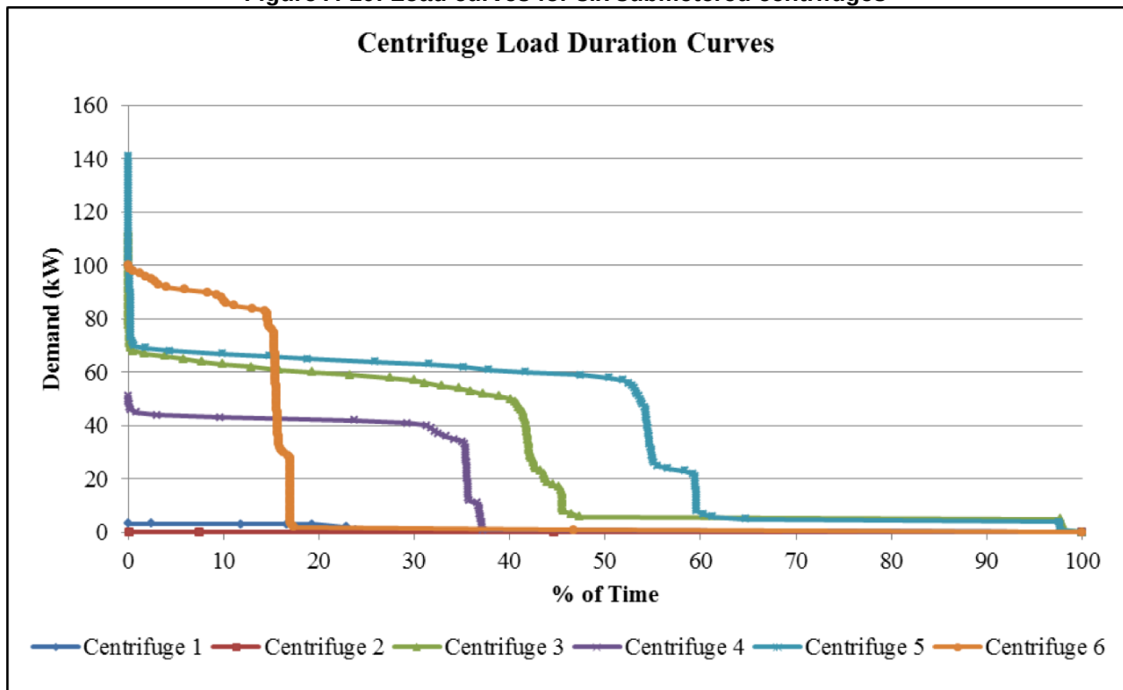
Figure A-10: Load curves for six submetered centrifuges
