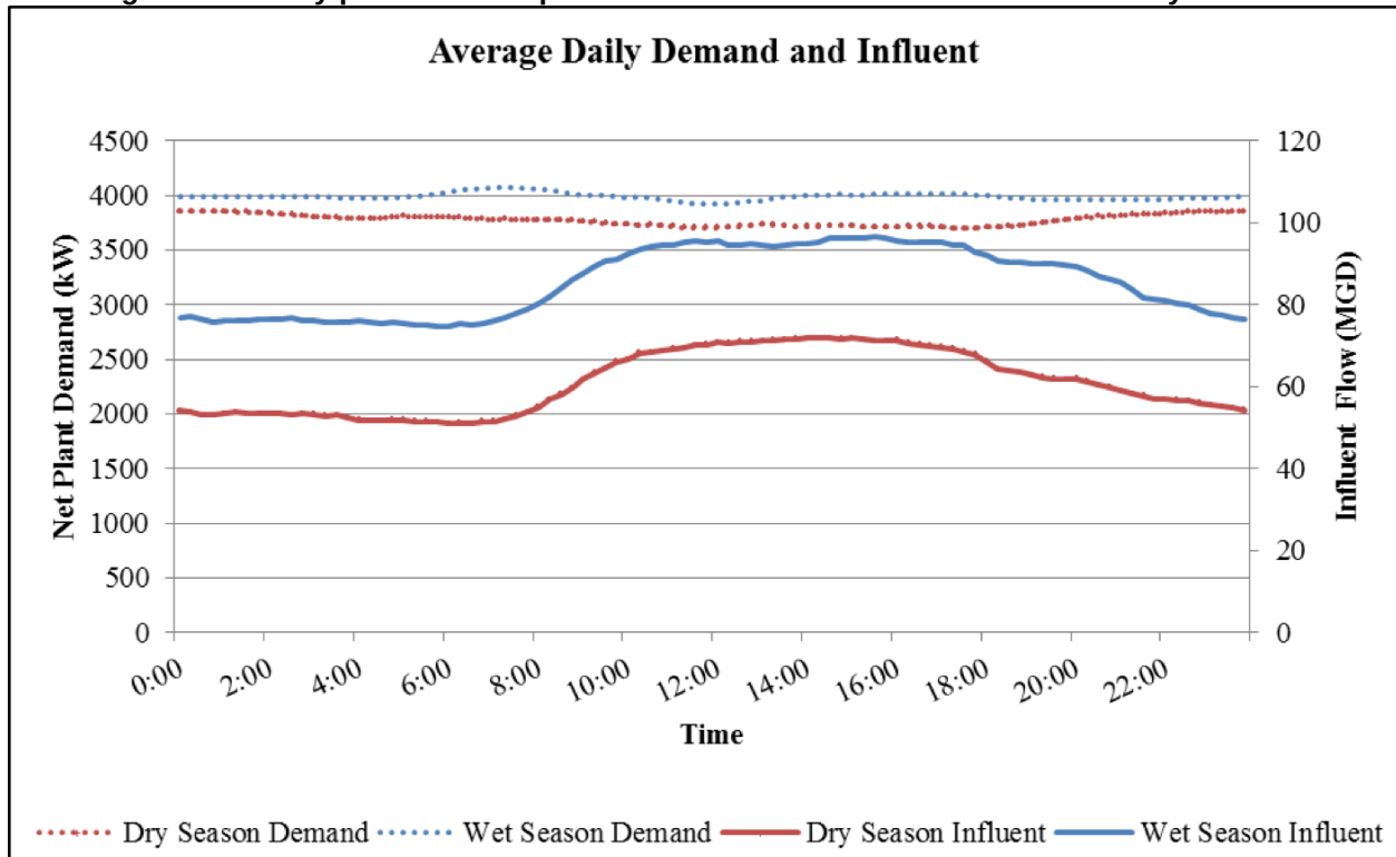
Figure A-4: Daily profile for net plant demand and influent flow in wet and dry seasons
