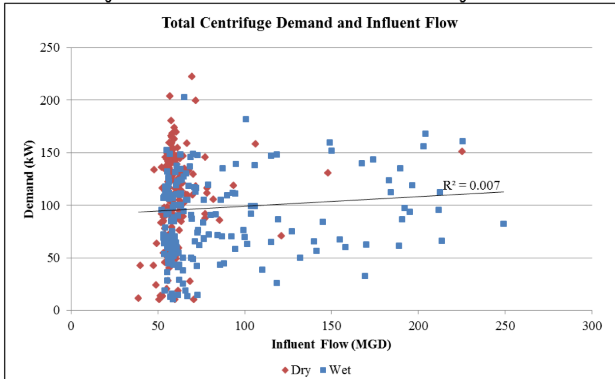
Figure A-11: Correlation between influent flow and centrifuge demand
