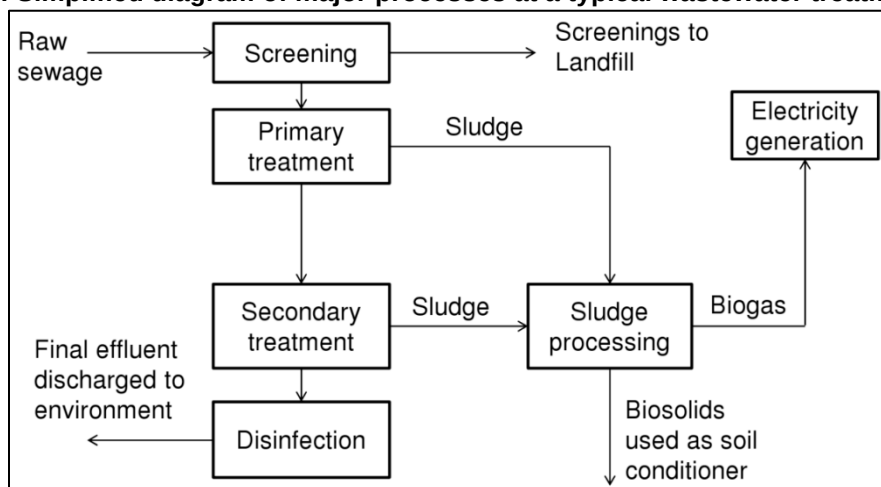
Figure 1: Simplified diagram of major processes at a typical wastewater treatment plant
