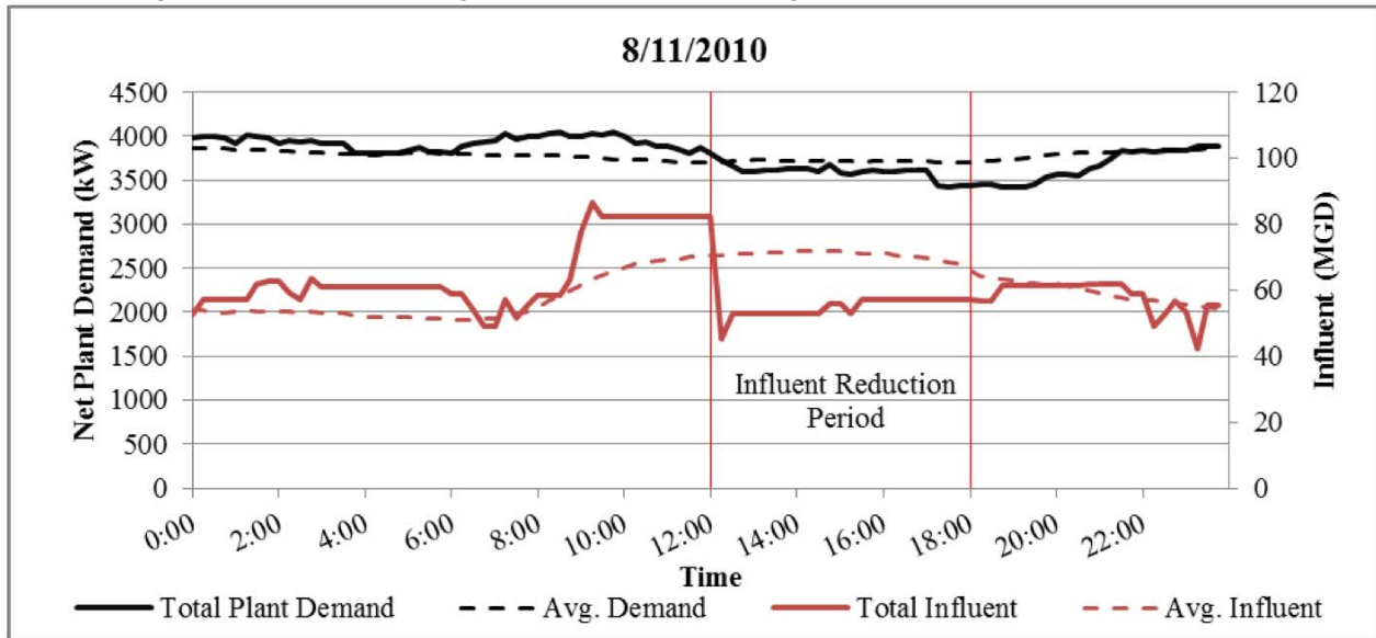
Figure 14: Reduction in plant demand coinciding with a reduction in influent flow
