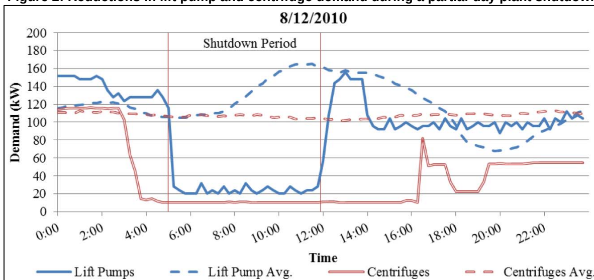
Figure 2: Reductions in lift pump and centrifuge demand during a partial-day plant shutdown
