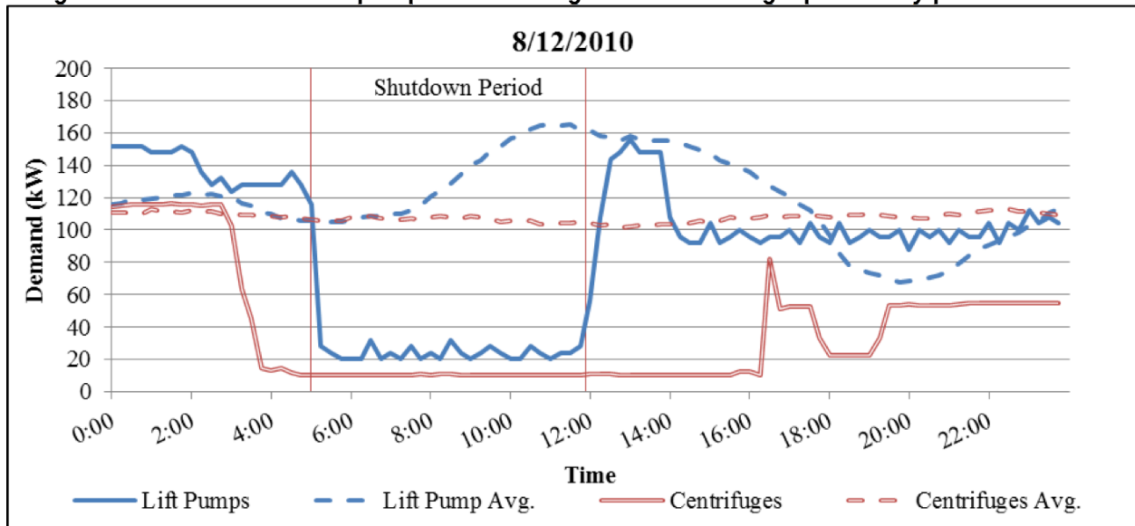
Figure 10: Reductions in lift pump and centrifuge demand during a partial-day plant shutdown
