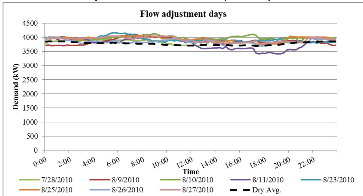
Figure A-16: Plant demand on flow adjustment days
