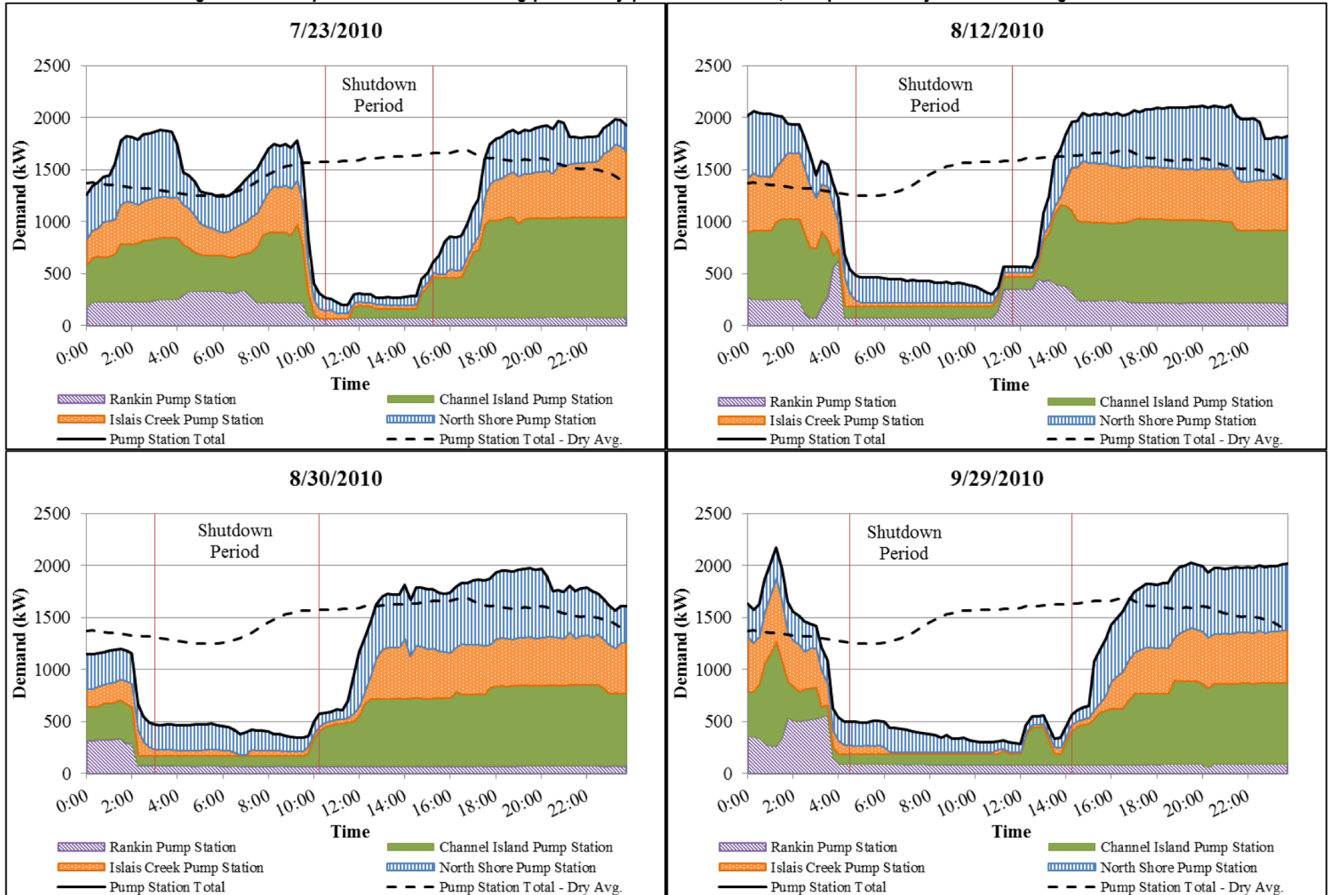
Figure 11: Pump station demand during partial-day plant shutdowns, compared to dry season average demand
