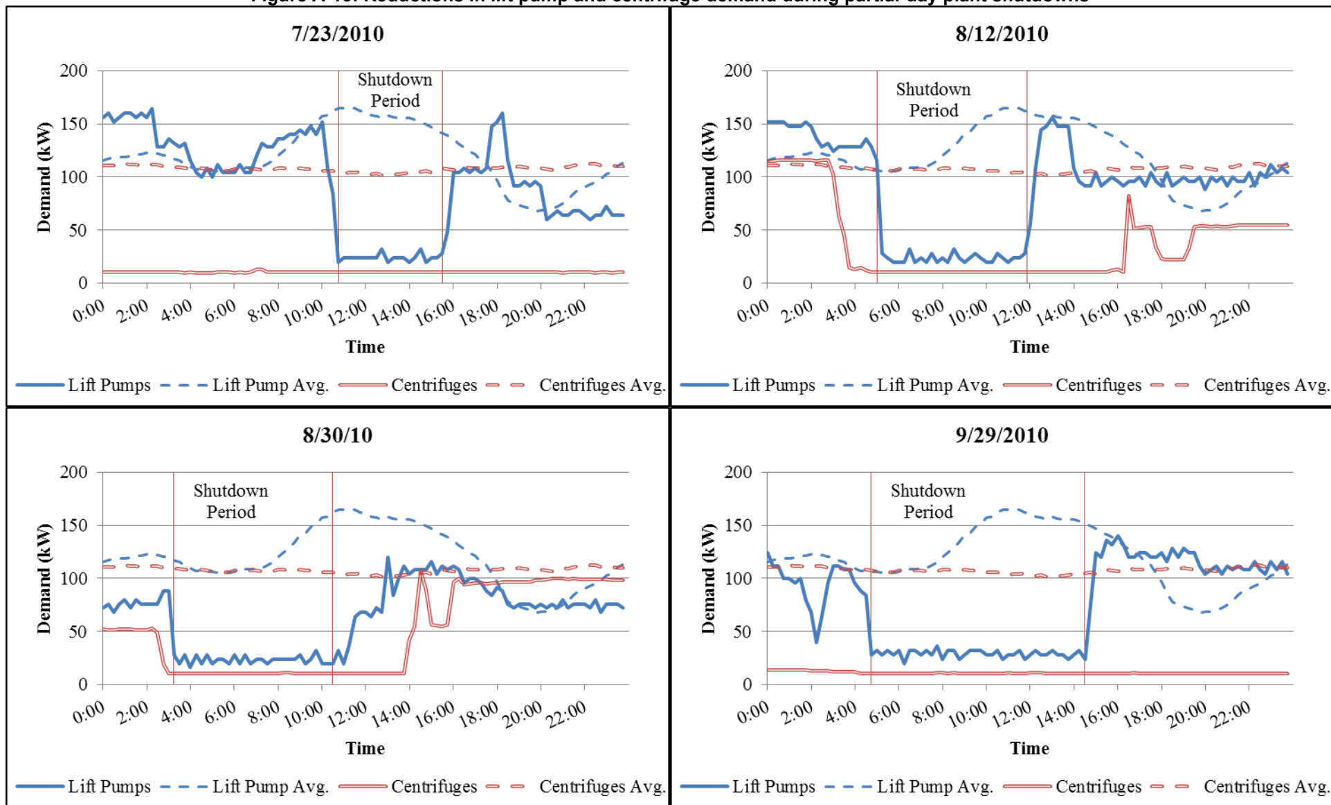
Figure A-15: Reductions in lift pump and centrifuge demand during partial-day plant shutdowns
