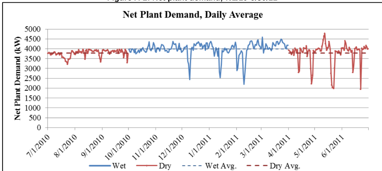
Figure A-2: Net plant demand, 7/1/10-6/30/11
