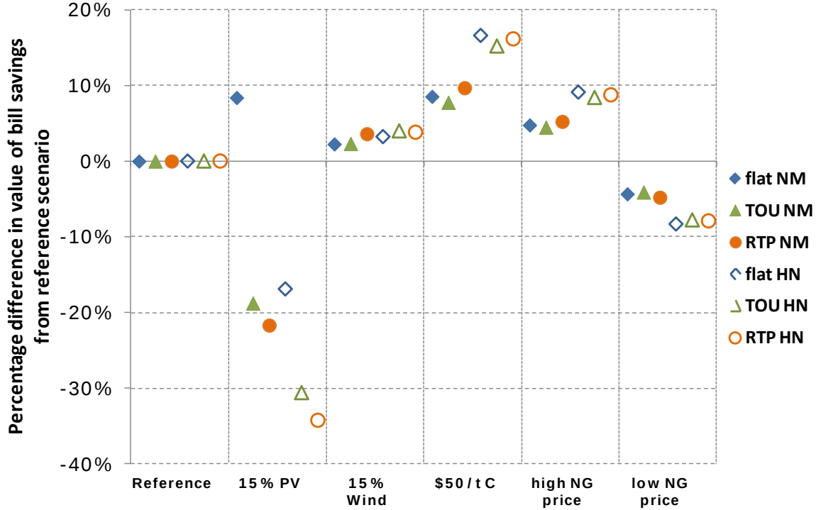
Figure 10: Value of bill savings for the isolation scenarios relative to the reference scenario's corresponding rate with net metering (NM) and hourly netting (HN). 75% PV-to-load ratio assumed.
