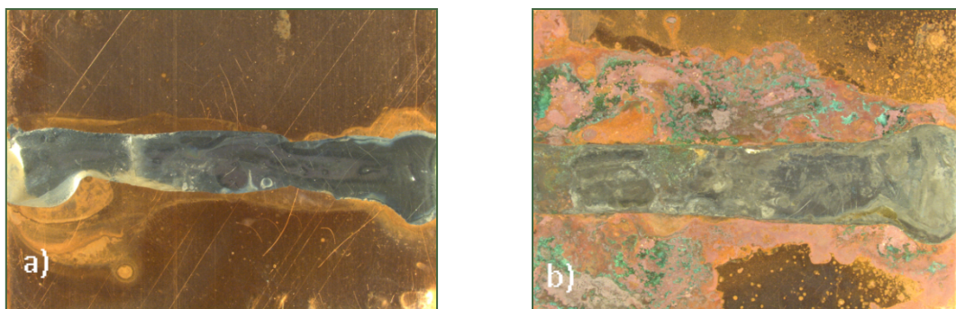
Figure 11. Clean B: a) BEST, RMA flux D, defluxer A1, b) WORST, ORH1 flux, defluxer V1.
