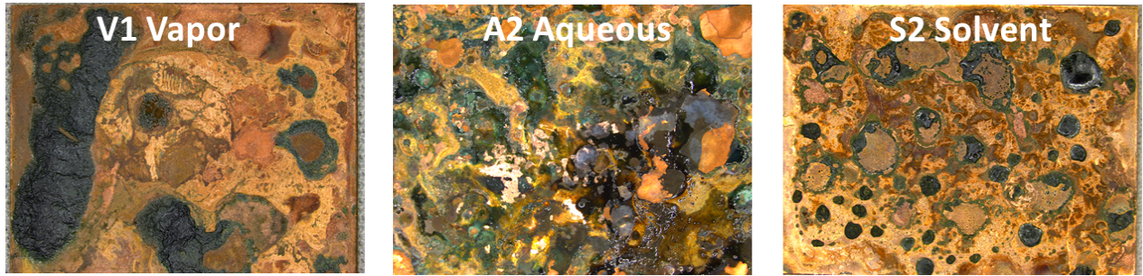
Figure 7. Worst of Low Temperature, C1 water soluble ORL1 flux.
