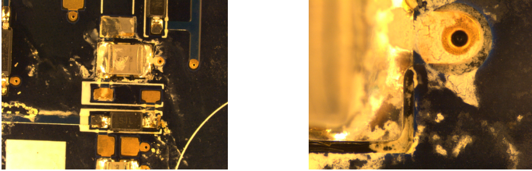
Figure 15. Printed wiring board with the greatest visible flux residue, V3 vapor defluxer.
