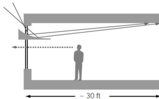
Figure 14: Direction of light at high level using a light shelf
