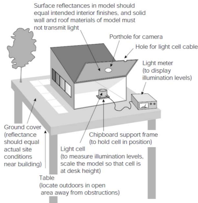
Figure 17: Scale models studied outdoors show the quality of lighting, flag glare problems, and provide measured daylight readings. Source: Concepts in Architectural Lighting , by M. D. Egan, McGraw-Hill, 2001.
