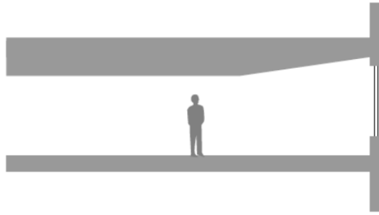
Figure 8: A sloping ceiling at the perimeter raises the window head without increasing floor-to-floor height.
