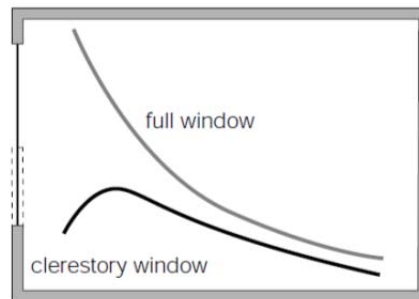
Figure 12: The curves indicate light levels for a full window and a clerestory, with the clerestory giving a softer gradient.
