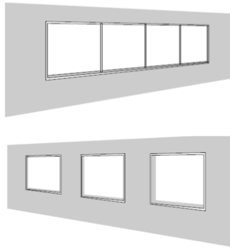
Figure 5: Strip windows are an easy way to provide uniform daylighting. Punched windows should be paired with work areas when possible.
