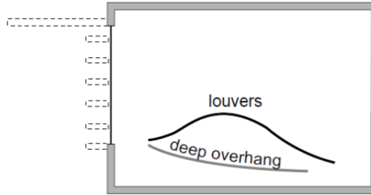
Figure 10: Illustration of the use of horizontal shapes to create a better distribution of daylight.
