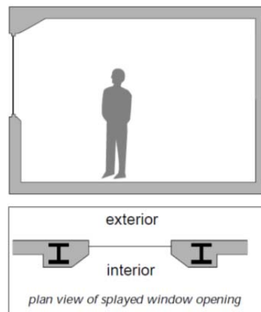
Figure 3: A splayed window opening, such as this one, helps to soften glare. These surfaces should be light-colored and provide an intermediate brightness between window and room surfaces, making an easier transition for the eye.
