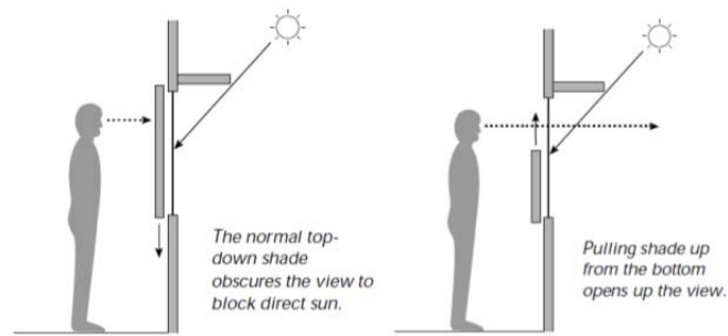
Figure 24: Left, the normal top-down shade obscures the view to block direct sun whereas pulling shade up from the bottom, right, opens up the view.
