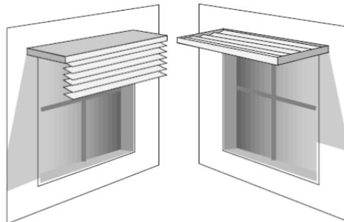
Figure 21: The use of louvers in place of a solid dropped edge (left) or solid overhang (right) provides diffuse natural light while still shading.
