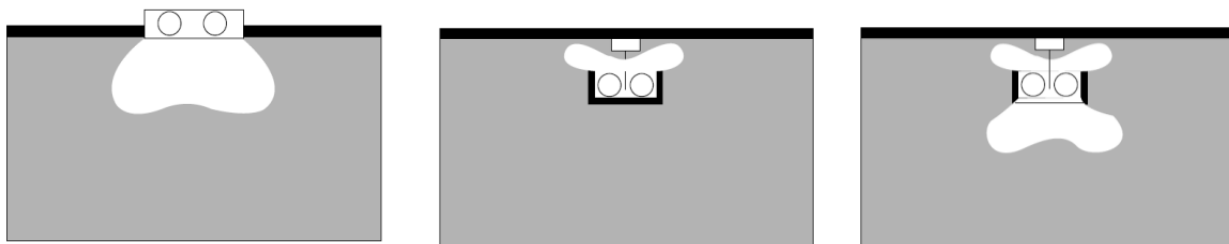
Figure 30: Illustrations of typical candlepower distribution for different ceiling-mounted lighting designs; left, direct lighting; center, indirect lighting; right, direct/indirect lighting
