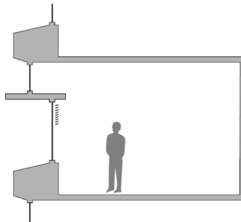
Figure 2: Section drawing illustrating a deep wall section providing some self-shading. This allows easy integration of a light shelf, creates surfaces that mitigate glare, and reduces noise
